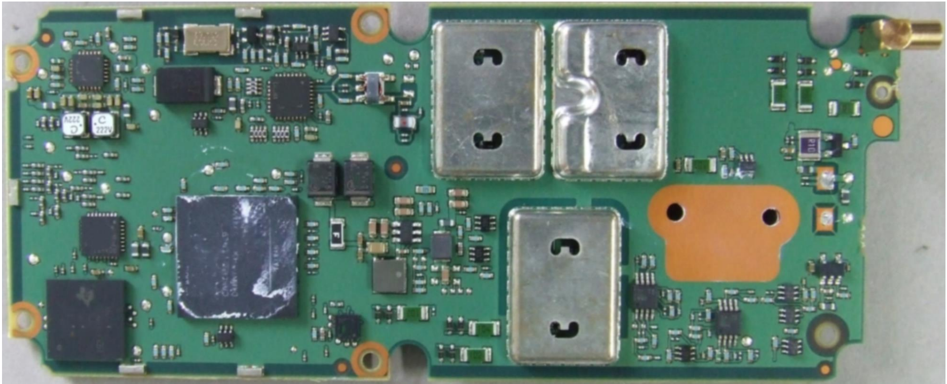
Photograph 03: Receive-Transmit PCB - bottom (with shields)
