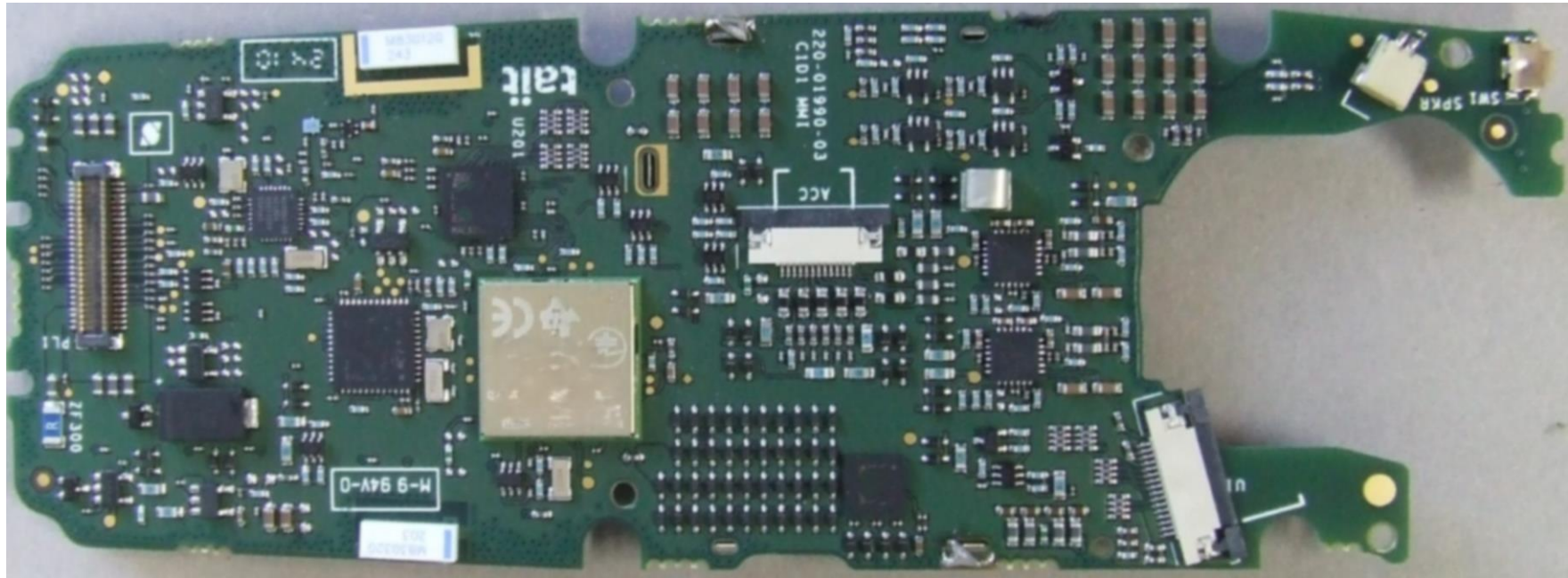
Photograph 06: Control PCB - Bottom
