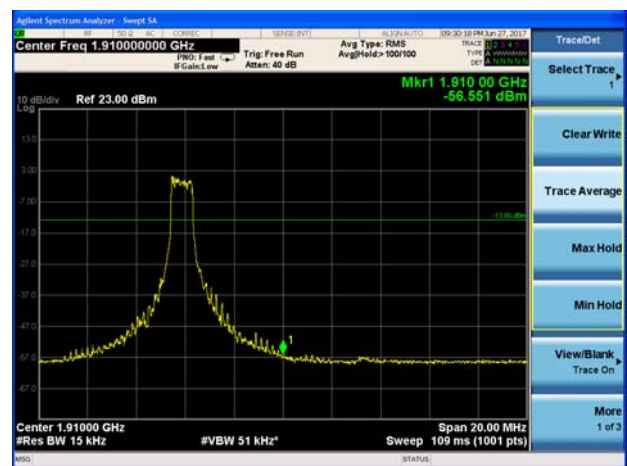
LTE Band 2 10MHz 16QAM 1RB CH-High
