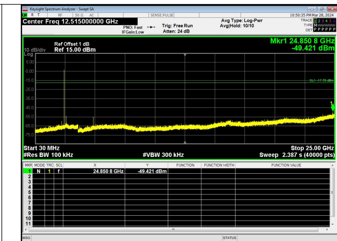
Spurious Emissions 8DPSK_3-DH5_Channel 39
