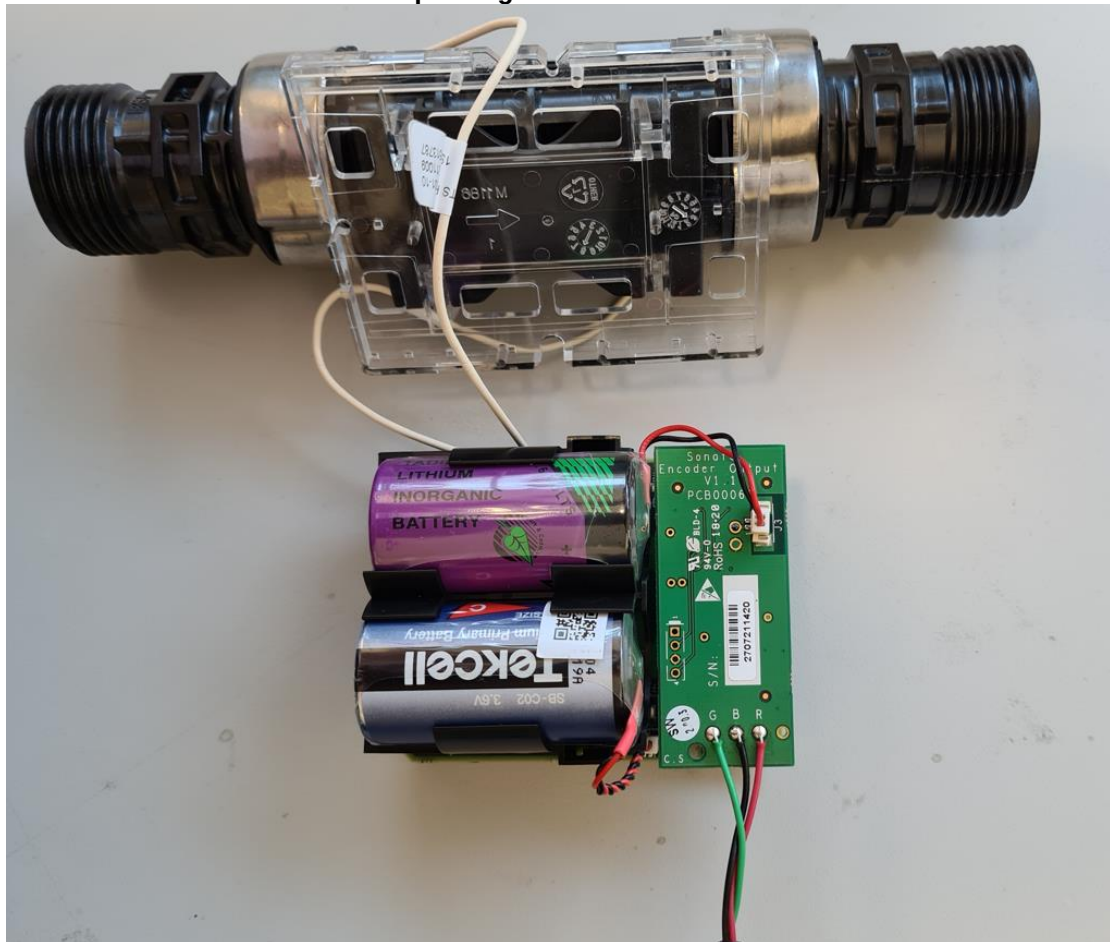
Photograph No.2 Sonata Sprint - general rear internal view
