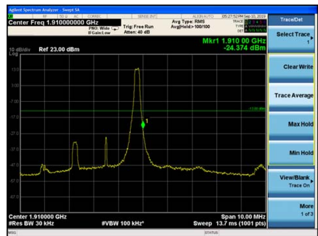
LTE Band 2 3MHz 16QAM 100%RB CH-High
