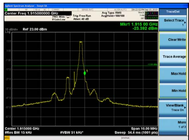
LTE Band 25 1.4MHz QPSK 1RB CH-High
