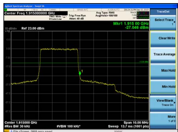
LTE Band 25 3MHz QPSK 100%RB CH-High
