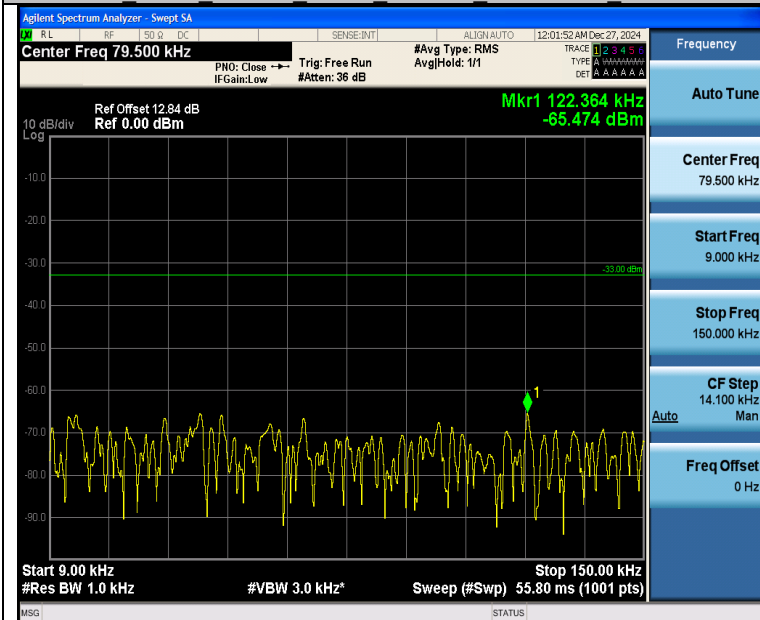
Band26_5MHz_QPSK_26915_1RB#0_0.009~0.15_0.009~0.15
