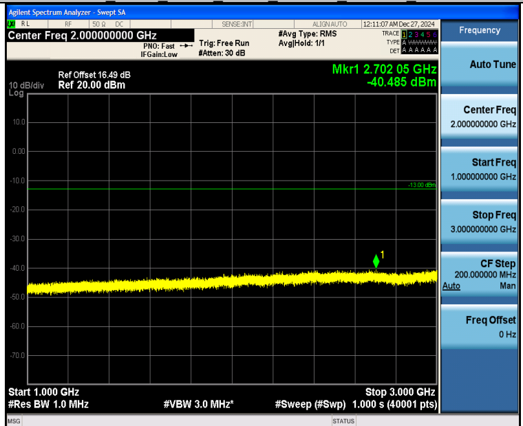
Band26_5MHz_QPSK_27015_1RB#24_1000~3000_1000~3000
