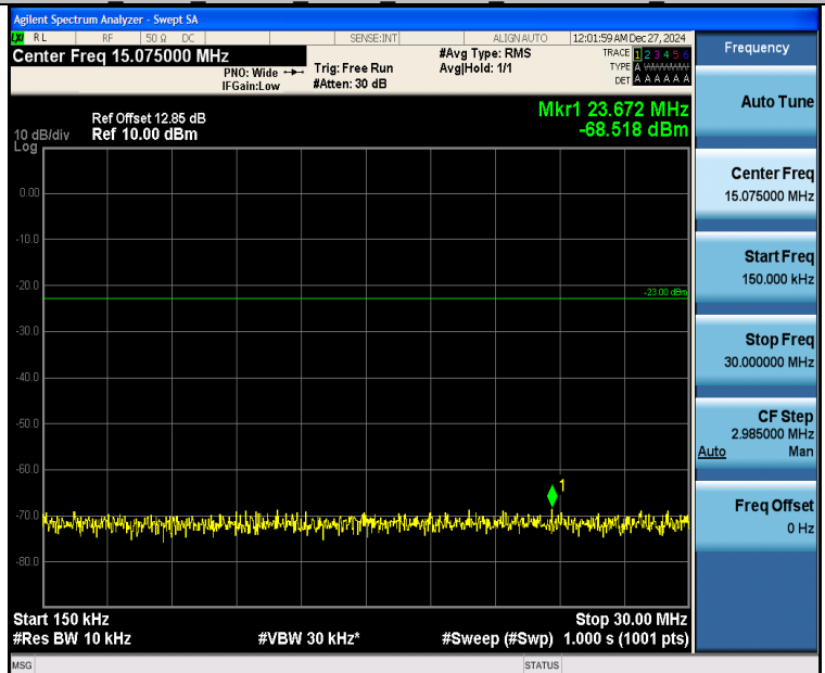
Band26_5MHz_QPSK_26915_1RB#0_0.15~30_0.15~30
