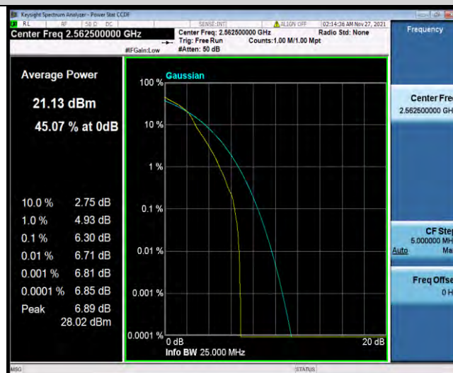
Band7-15MHz-16QAM-21375-27RB#0
