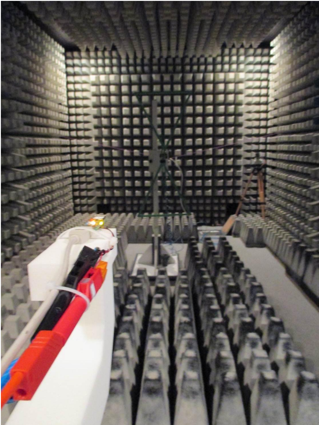
151496_16: Test setup - Radiated emission, internal antenna (fully anechoic chamber)
