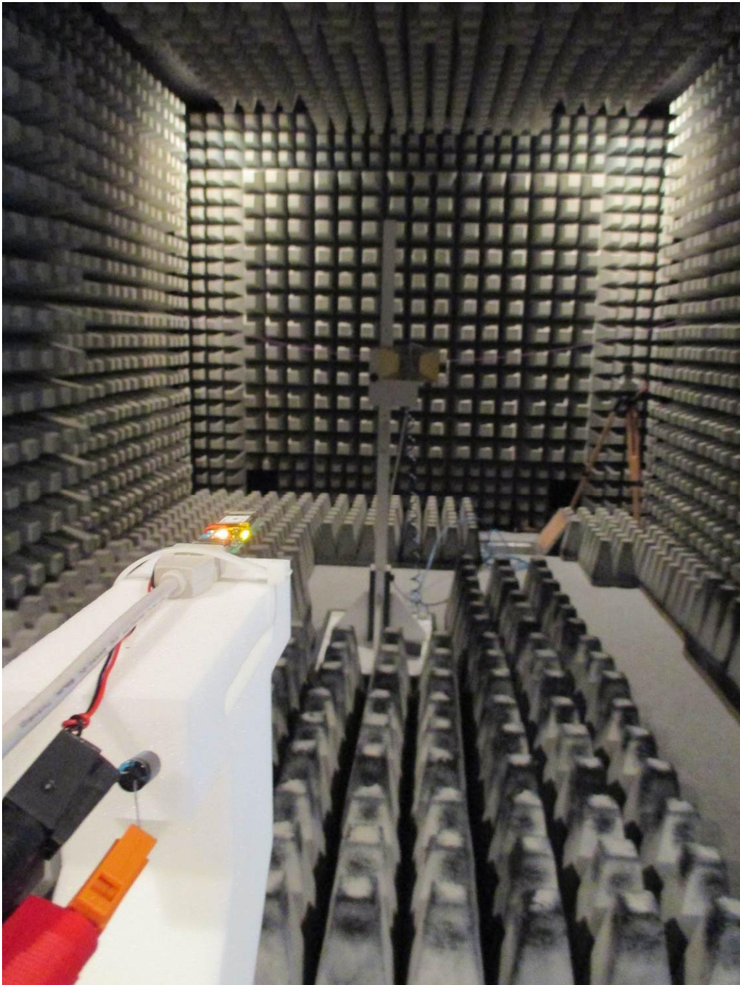
151496_17: Test setup - Radiated emission, internal antenna (fully anechoic chamber)
