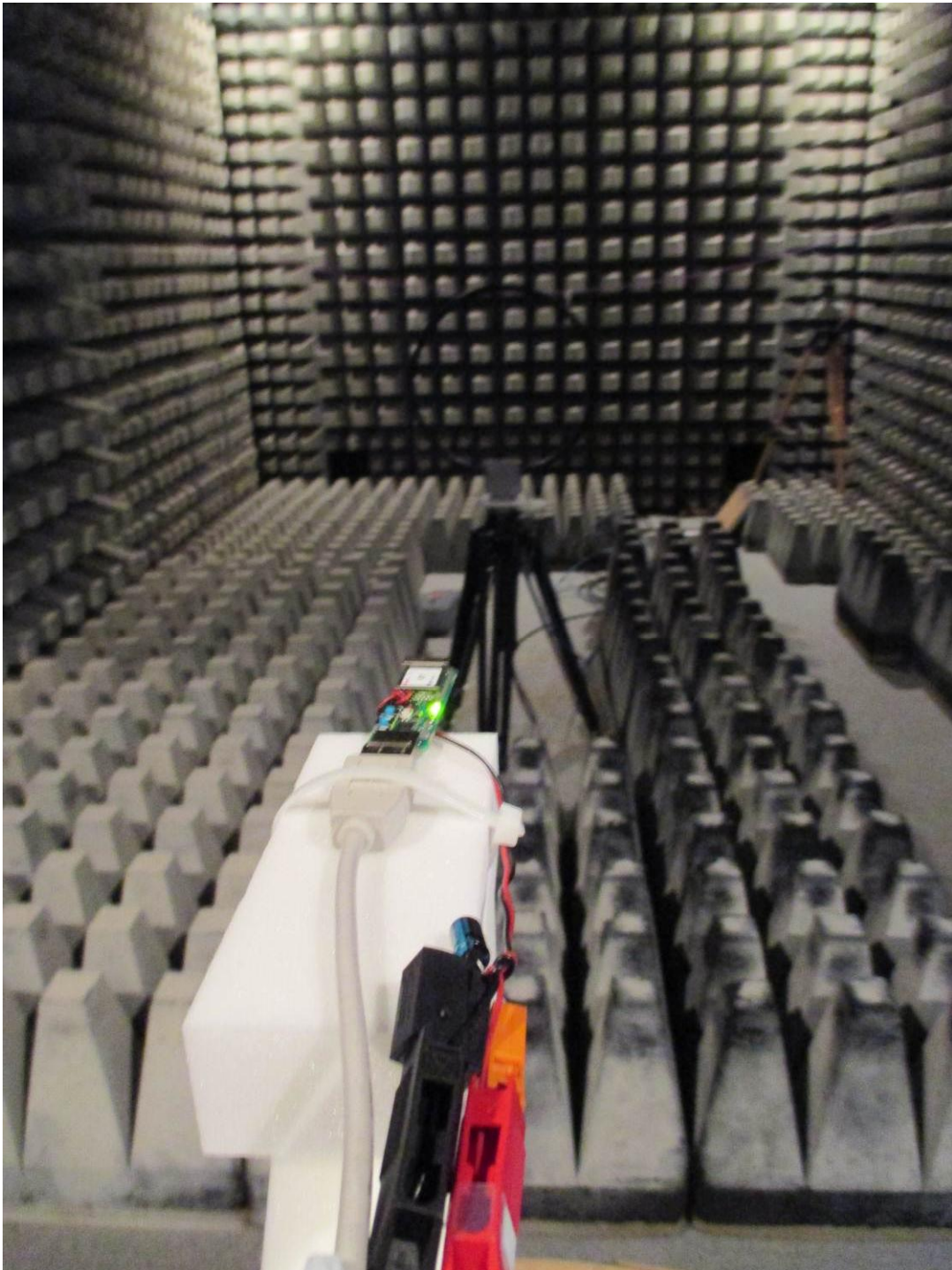
151496_19: Test setup - Radiated emission, internal antenna (fully anechoic chamber)
