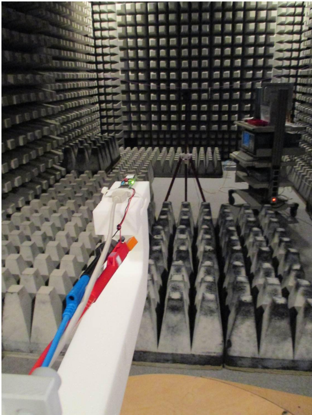
151496_18: Test setup - Radiated emission, Antennas terminated (fully anechoic chamber)
