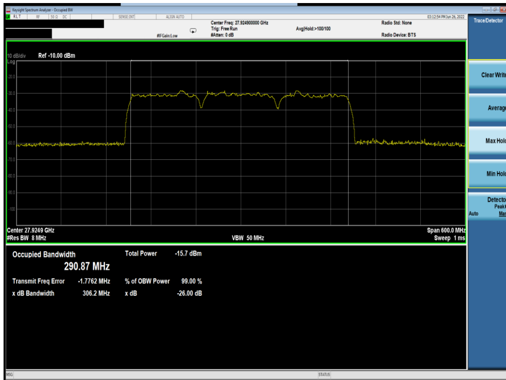
Plot 7-291. Ant M0 OBW (Band n261-100MHz-3CC SISO Dual Pol DFTs-OFDM – \pi/2 BPSK – Mid Channel)
