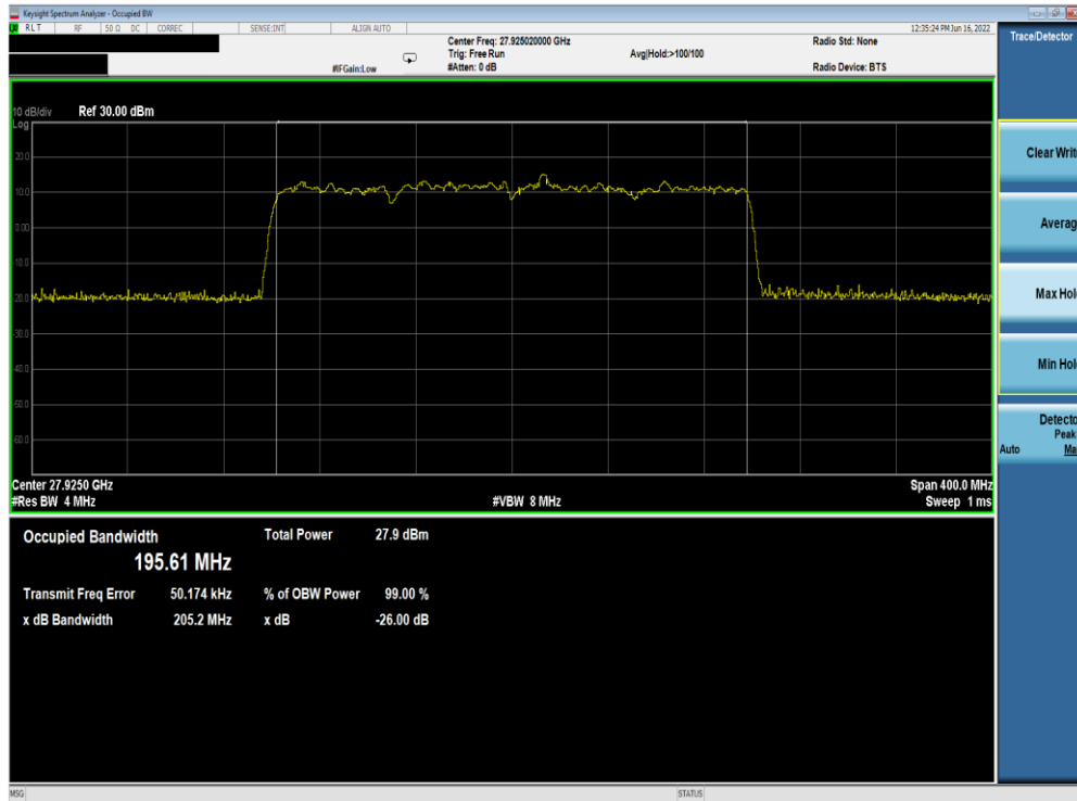
Plot 7-249. Ant M0 OBW (Band n261-50MHz-4CC SISO Dual Pol DFTs-OFDM – \pi/2 BPSK – Mid Channel)
