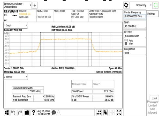
Band2_20MHz_256QAM_RB100_0_CH19100
