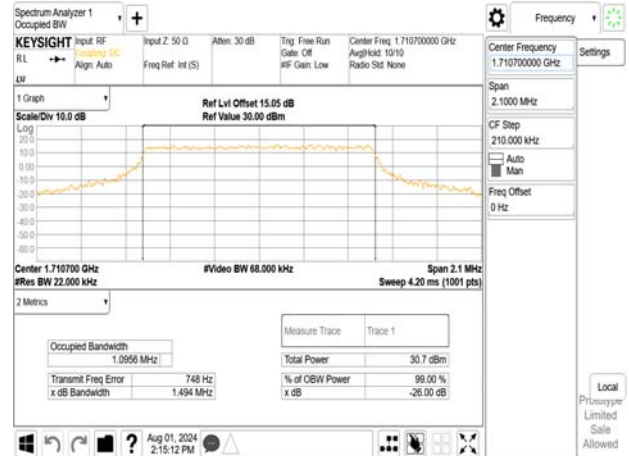
Band4_1.4MHz_16QAM_RB6_0_CH20175
