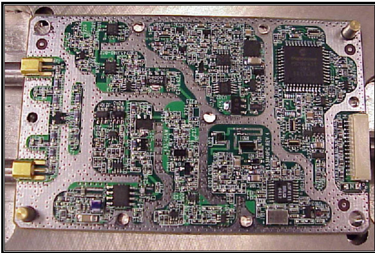
PHOTOGRAPH 15: ALIEN RFID CARD SIDE 1
