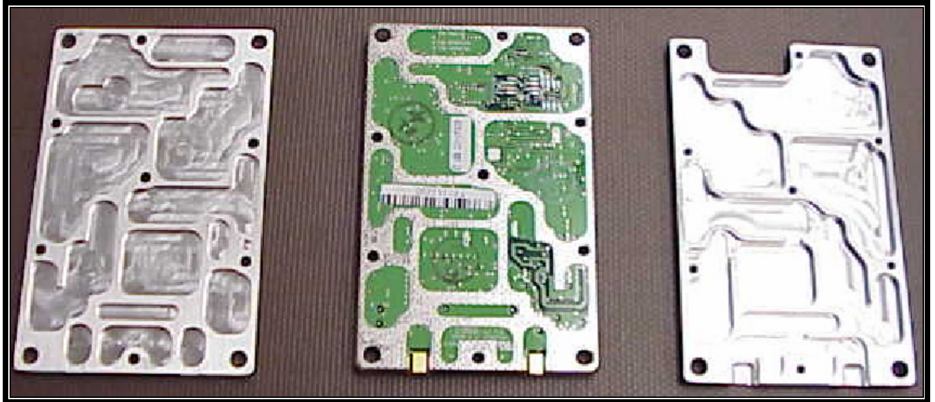
PHOTOGRAPH 16: ALIEN RFID CARD SIDE 2 AND INSIDE CASE
