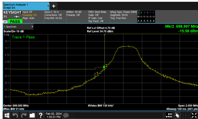
Band12-3MHz-QPSK-23025-1RB#14
