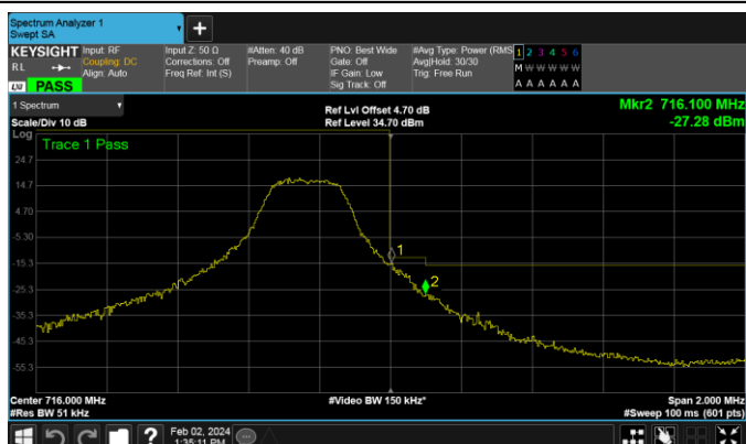
Band12-3MHz-16QAM-23165-15RB#0
