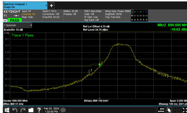
Band12-3MHz-16QAM-23025-1RB#14
