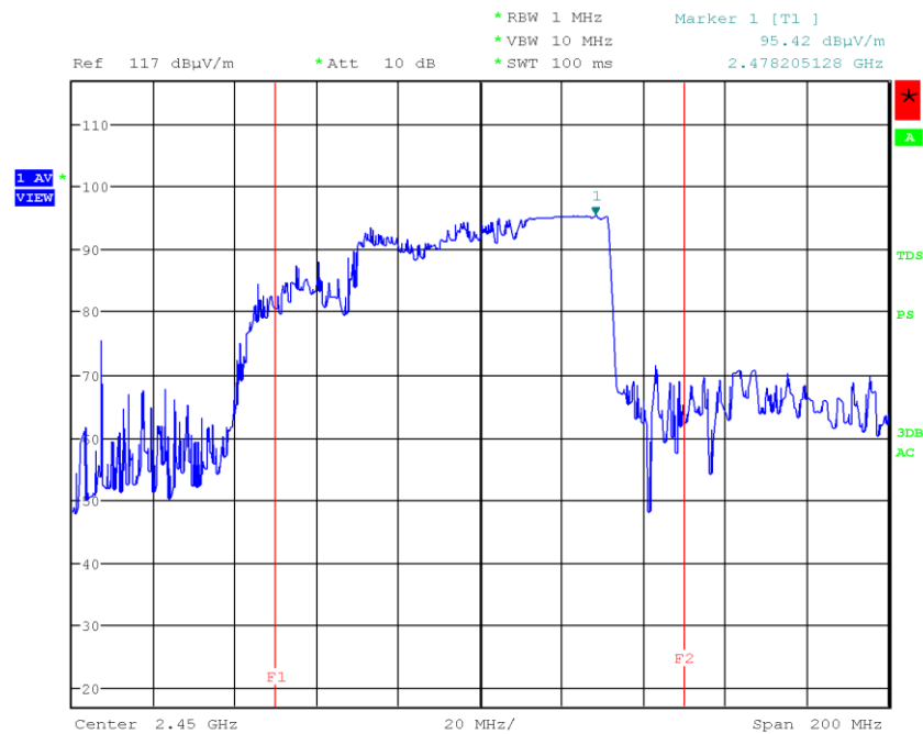
< Fig 9. Frequency Measurements _Load (Maximum Frequency Observed: 2.478 GHz) >
