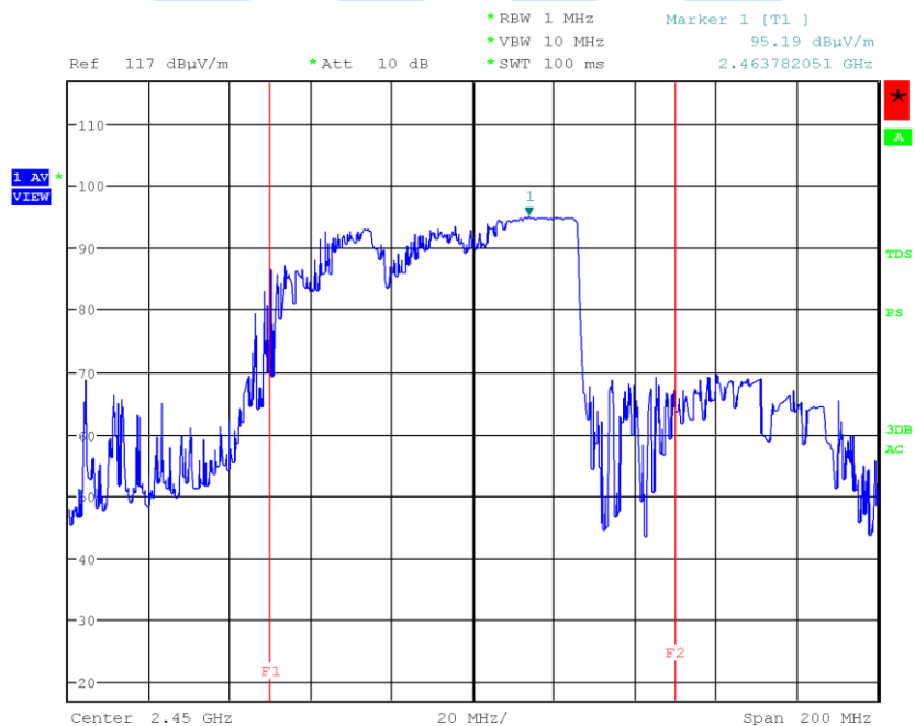
< Fig 8. Frequency Measurements _ Voltage (Minimum Frequency Observed: 2.463 GHz) >
