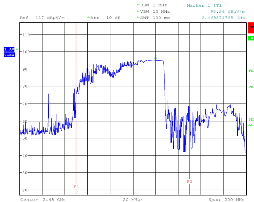
< Fig 10. Frequency Measurements _Load (Minimum Frequency Observed: 2.469 GHz) >
