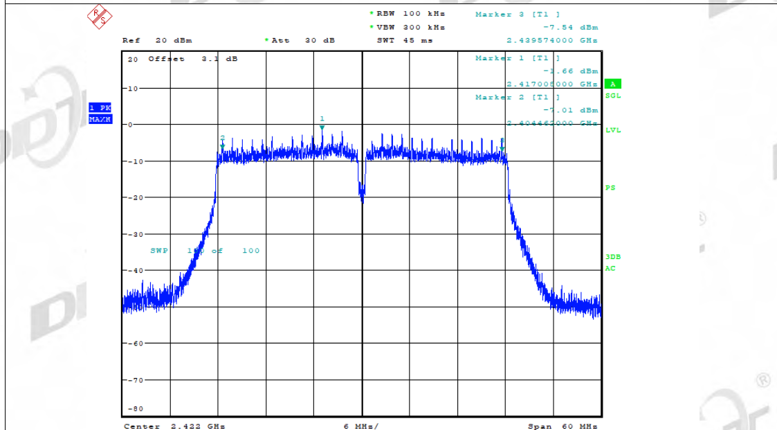
-6dB Bandwidth NVNT n40 2422MHz Ant2
