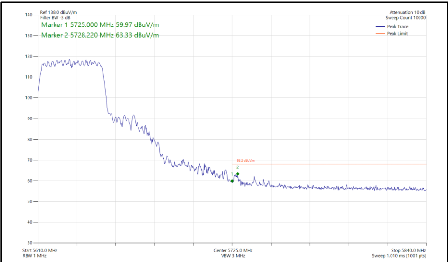
Figure 543 - 802.11n HT40, CDD, Core 0 - Core 1 - 5630 MHz Band Edge Frequency 5725 MHz
