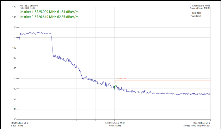
Figure 501 - 802.11ax HE40, SU, SISO, Core 0 - 5630 MHz Band Edge Frequency 5725 MHz
