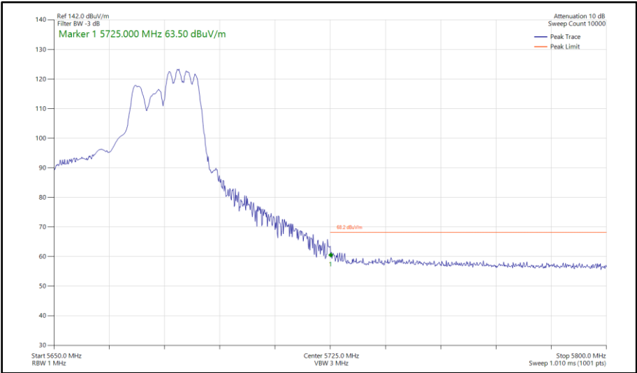
Figure 548 - 802.11ax HE40, RU 106-56, CDD, Core 0 - Core 1 - 5670 MHz Band Edge Frequency 5725 MHz
