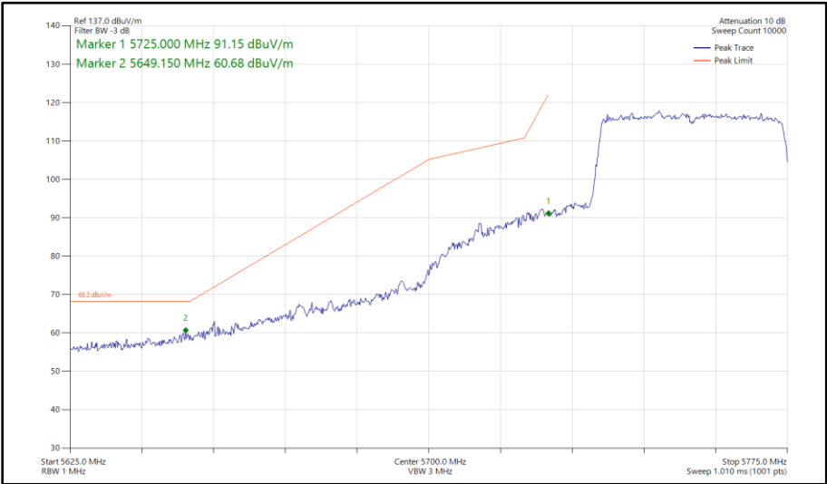
Figure 497 - 802.11ax HE40, SU, SISO, Core 0 - 5755 MHz Band Edge Frequency 5725 MHz
