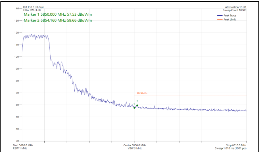
Figure 549 - 802.11n HT40, CDD, Core 0 - Core 1 - 5710 MHz Band Edge Frequency 5850 MHz
