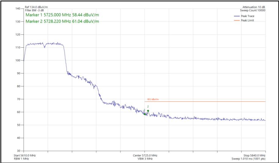
Figure 499 - 802.11n HT40, SISO, Core 0 - 5630 MHz Band Edge Frequency 5725 MHz
