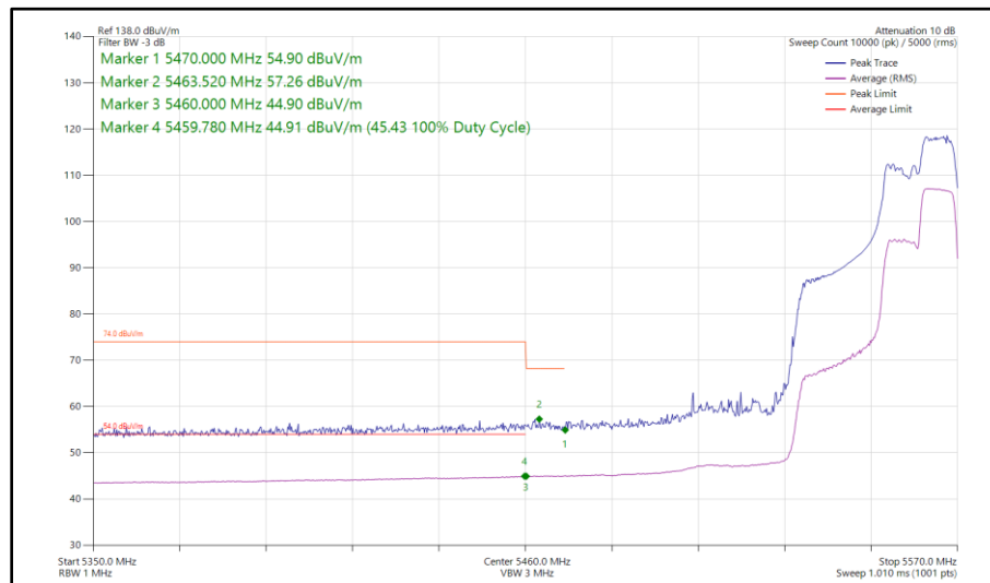
Figure 495 - 802.11ax HE40, RU 106-56, SISO, Core 0 - 5550 MHz Band Edge Frequency 5470 MHz
