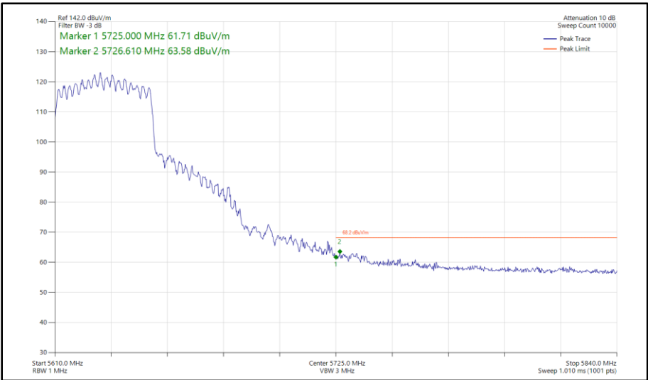
Figure 545 - 802.11ax HE40, SU, CDD, Core 0 - Core 1 - 5630 MHz Band Edge Frequency 5725 MHz
