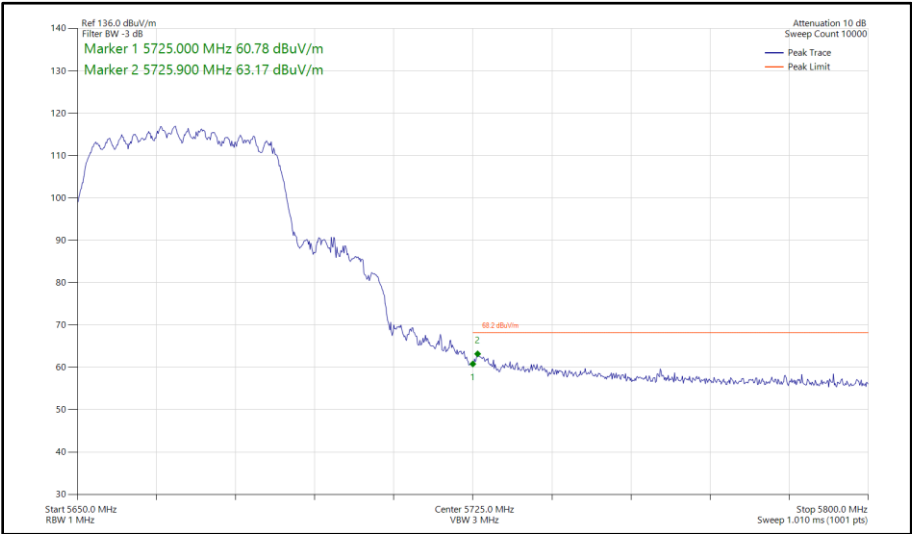
Figure 544 - 802.11n HT40, CDD, Core 0 - Core 1 - 5670 MHz Band Edge Frequency 5725 MHz
