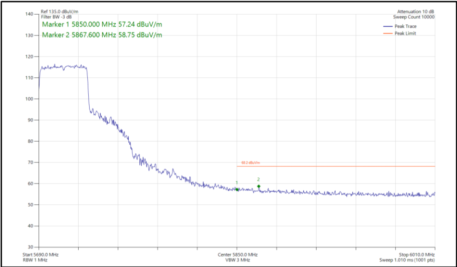
Figure 507 - 802.11ax HE40, SU, SISO, Core 0 - 5710 MHz Band Edge Frequency 5850 MHz
