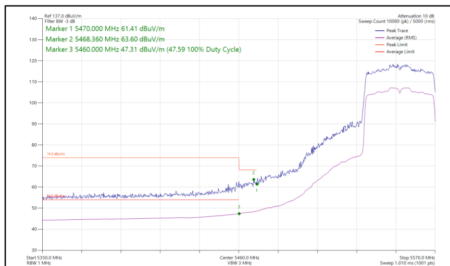
Figure 515 - 802.11ax HE40, SU, SISO, Core 1 - 5550 MHz Band Edge Frequency 5470 MHz
