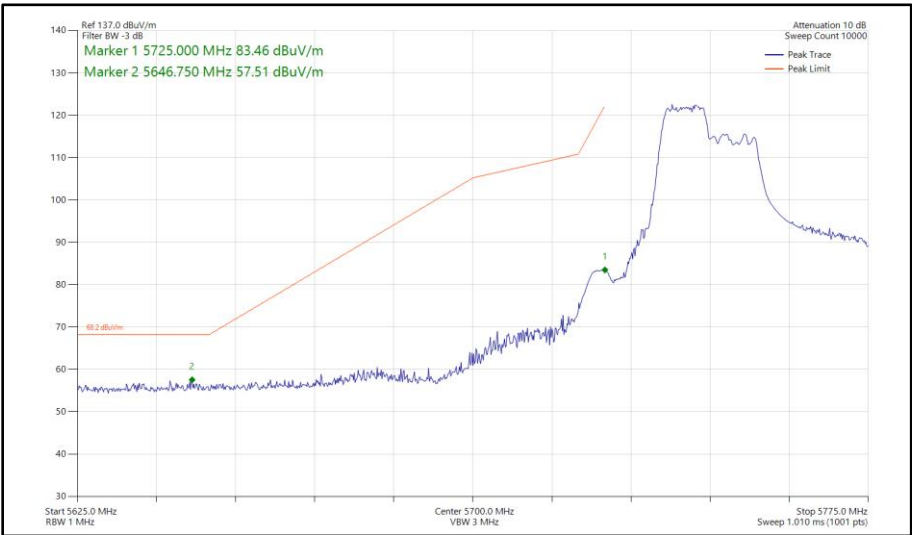
Figure 519 - 802.11ax HE40, RU 106-53, SISO, Core 1 - 5755 MHz Band Edge Frequency 5725 MHz
