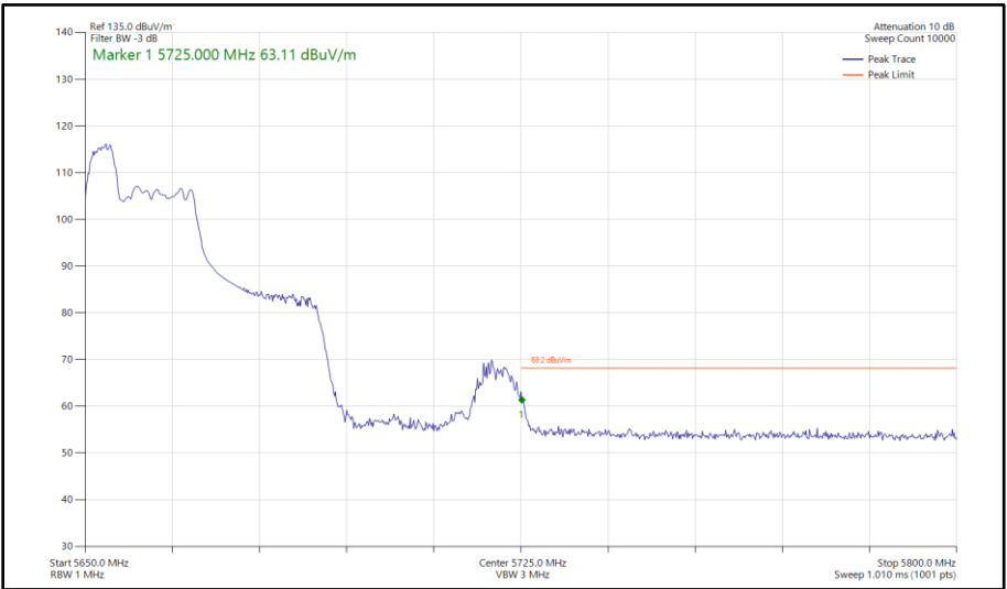
Figure 504 - 802.11ax HE40, RU 52-37, SISO, Core 0 - 5670 MHz Band Edge Frequency 5725 MHz
