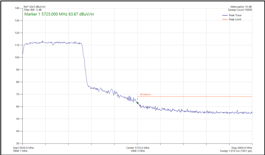
Figure 524 - 802.11ax HE40, SU, SISO, Core 1 - 5670 MHz Band Edge Frequency 5725 MHz
