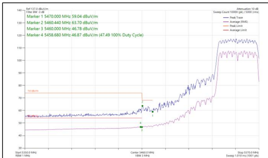
Figure 533 - 802.11n HT40, CDD, Core 0 - Core 1 - 5550 MHz Band Edge Frequency 5470 MHz
