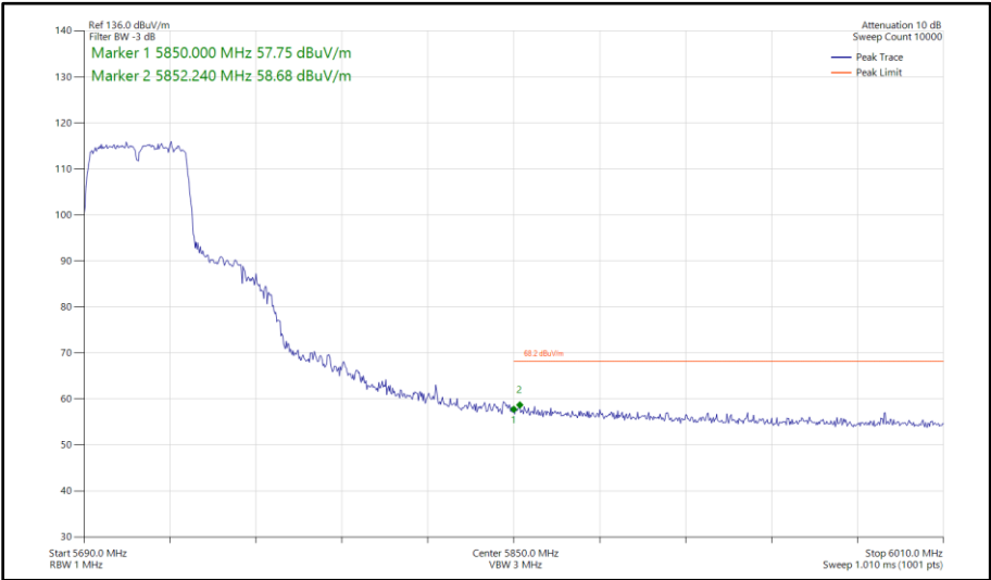
Figure 505 - 802.11n HT40, SISO, Core 0 - 5710 MHz Band Edge Frequency 5850 MHz
