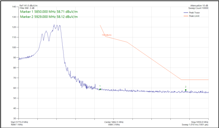
Figure 554 - 802.11ax HE40, RU 106-56, CDD, Core 0 - Core 1 - 5795 MHz Band Edge Frequency 5850 MHz
