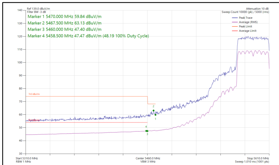
Figure 561 - 802.11ax HE40, SU, SDM, Core 0 - Core 1 - 5590 MHz Band Edge Frequency 5470 MHz
