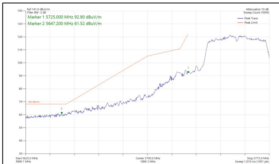
Figure 562 - 802.11n HT40, SDM, Core 0 - Core 1 - 5755 MHz Band Edge Frequency 5725 MHz
