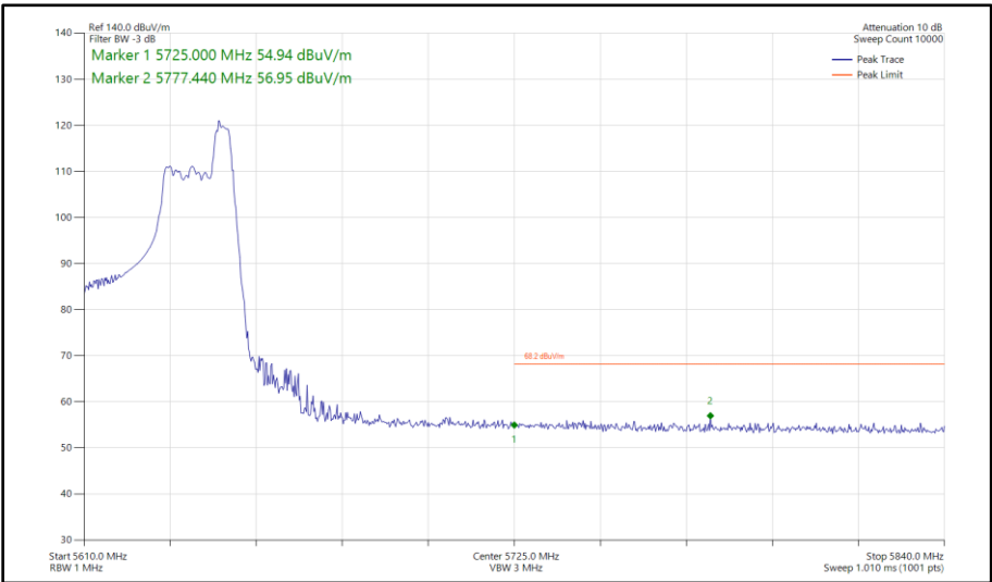
Figure 502 - 802.11ax HE40, RU 52-44, SISO, Core 0 - 5630 MHz Band Edge Frequency 5725 MHz
