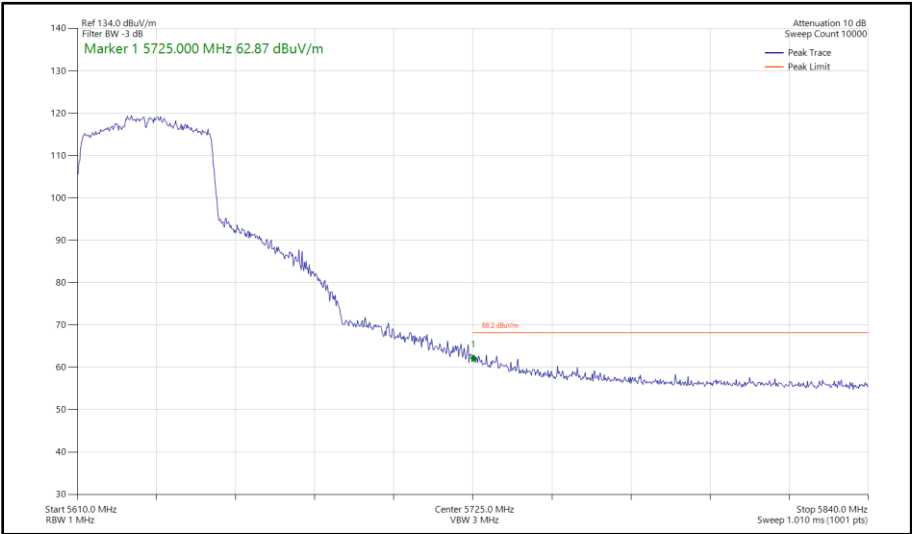
Figure 522 - 802.11ax HE40, SU, SISO, Core 1 - 5630 MHz Band Edge Frequency 5725 MHz
