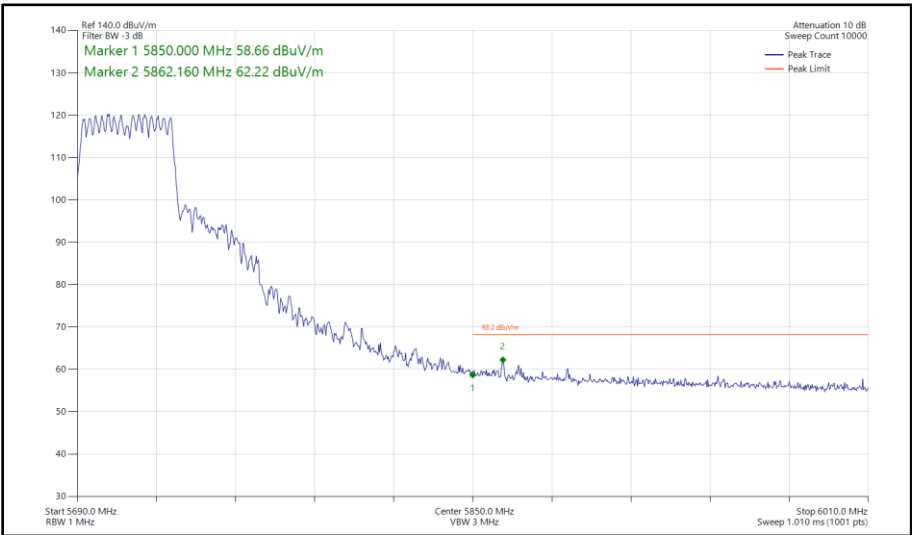
Figure 551 - 802.11ax HE40, SU, CDD, Core 0 - Core 1 - 5710 MHz Band Edge Frequency 5850 MHz
