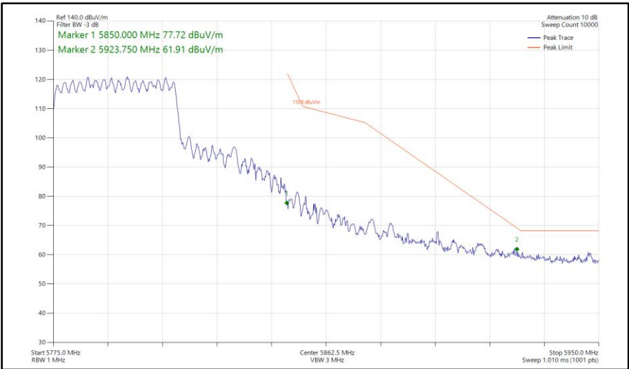
Figure 553 - 802.11ax HE40, SU, CDD, Core 0 - Core 1 - 5795 MHz Band Edge Frequency 5850 MHz
