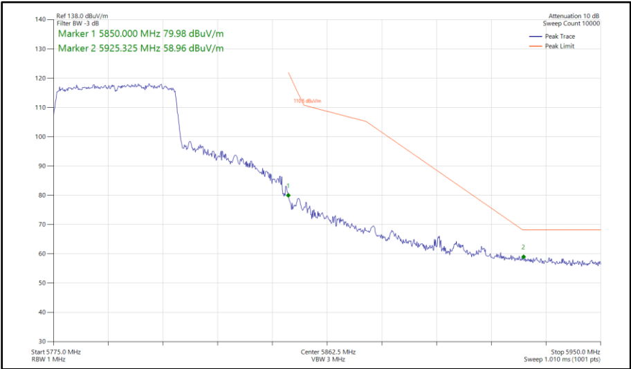
Figure 509 - 802.11ax HE40, SU, SISO, Core 0 - 5795 MHz Band Edge Frequency 5850 MHz
