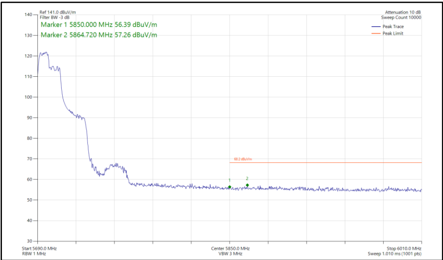
Figure 529 - 802.11ax HE40, RU 106-53, SISO, Core 1 - 5710 MHz Band Edge Frequency 5850 MHz
