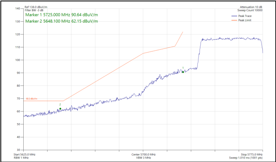
Figure 518 - 802.11ax HE40, SU, SISO, Core 1 - 5755 MHz Band Edge Frequency 5725 MHz
