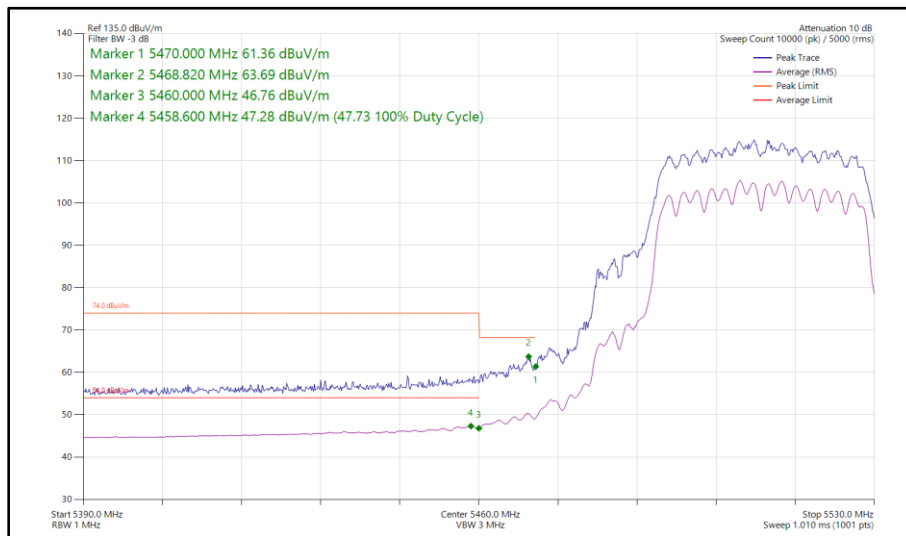
Figure 532 - 802.11n HT40, CDD, Core 0 - Core 1 - 5510 MHz Band Edge Frequency 5470 MHz
