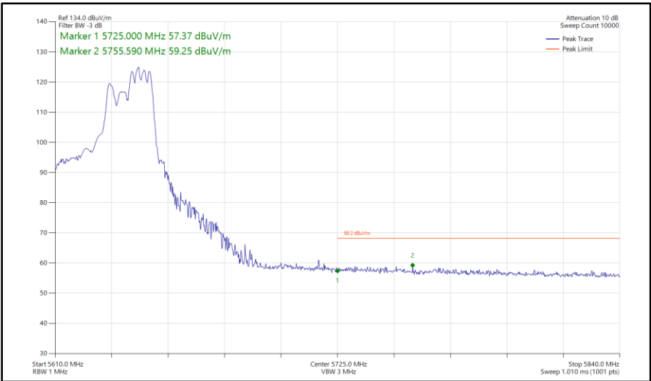
Figure 568 - 802.11ax HE40, RU 106-56, SDM, Core 0 - Core 1 - 5630 MHz Band Edge Frequency 5725 MHz
