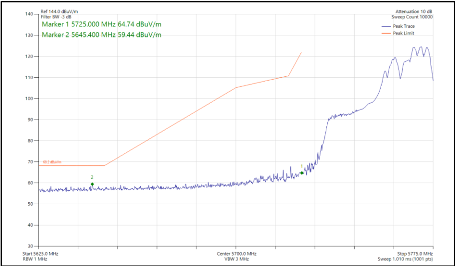
Figure 542 - 802.11ax HE40, RU 106-56, CDD, Core 0 - Core 1 - 5755 MHz Band Edge Frequency 5725 MHz
