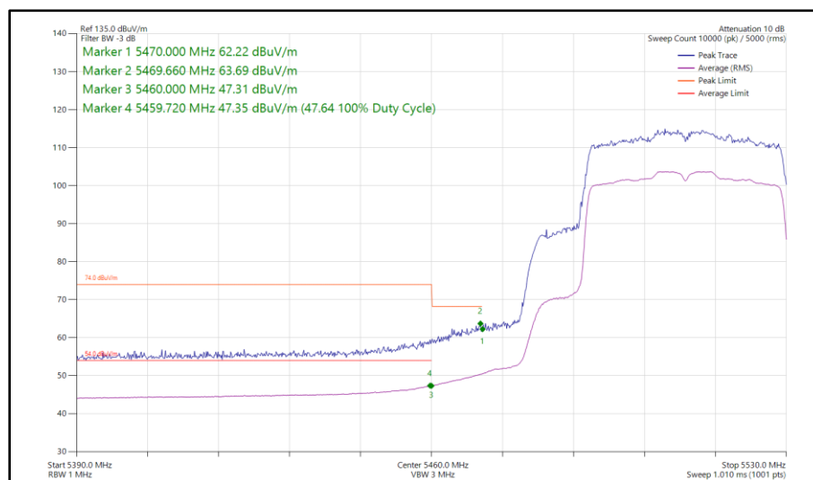
Figure 513 - 802.11ax HE40, SU, SISO, Core 1 - 5510 MHz Band Edge Frequency 5470 MHz
