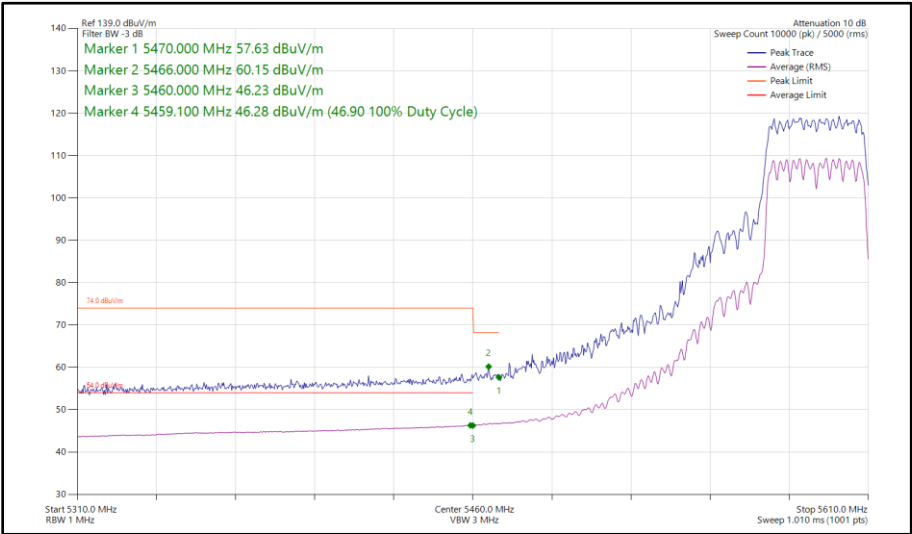
Figure 534 - 802.11n HT40, CDD, Core 0 - Core 1 - 5590 MHz Band Edge Frequency 5470 MHz
