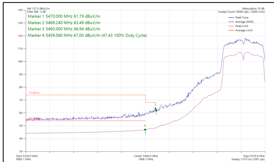
Figure 512 - 802.11n HT40, SISO, Core 1 - 5550 MHz Band Edge Frequency 5470 MHz
