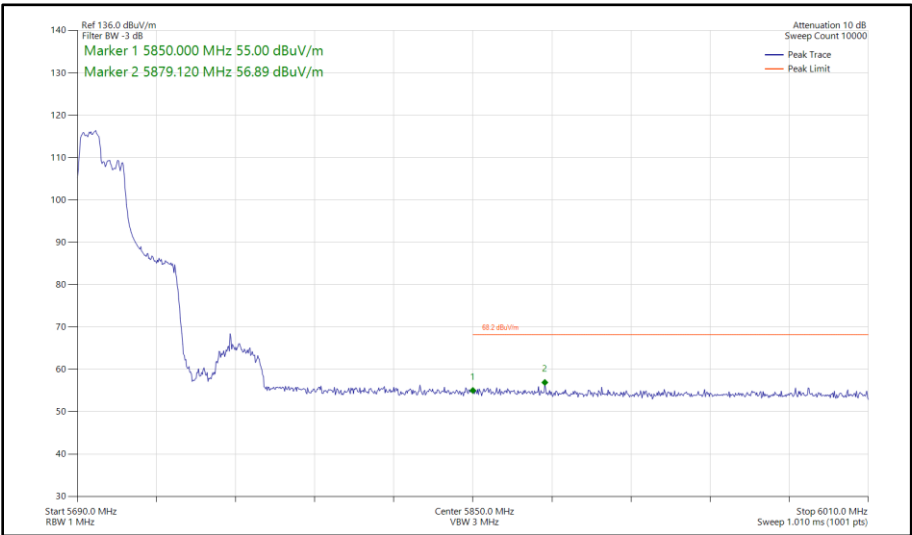
Figure 508 - 802.11ax HE40, RU 106-53, SISO, Core 0 - 5710 MHz Band Edge Frequency 5850 MHz
