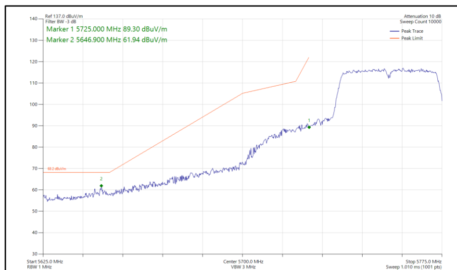
Figure 496 - 802.11n HT40, SISO, Core 0 - 5755 MHz Band Edge Frequency 5725 MHz
