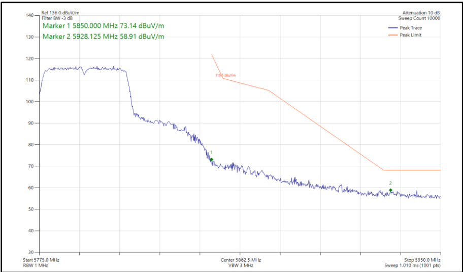
Figure 527 - 802.11n HT40, SISO, Core 1 - 5795 MHz Band Edge Frequency 5850 MHz
