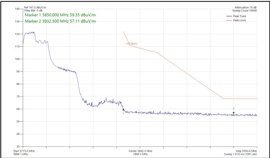
Figure 531 - 802.11ax HE40, RU 106-53, SISO, Core 1 - 5795 MHz Band Edge Frequency 5850 MHz
