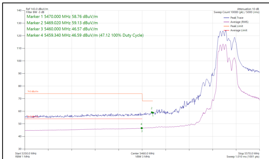
Figure 560 - 802.11ax HE40, RU 106-53, SDM, Core 0 - Core 1 - 5550 MHz Band Edge Frequency 5470 MHz
