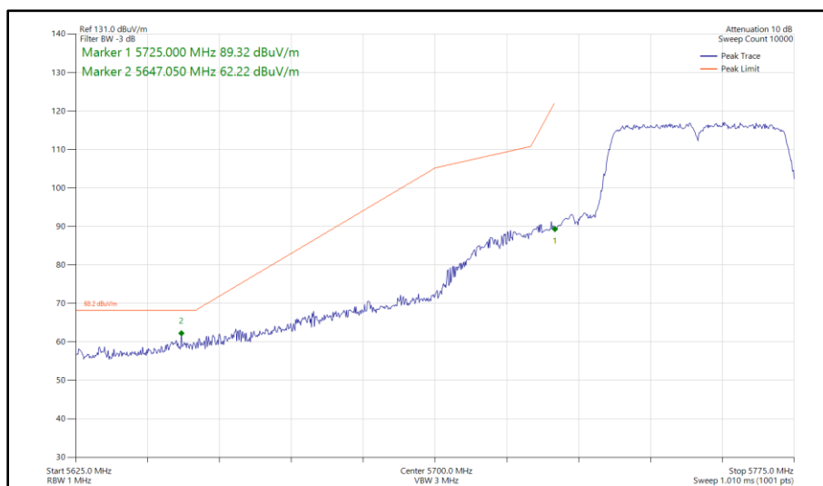
Figure 517 - 802.11n HT40, SISO, Core 1 - 5755 MHz Band Edge Frequency 5725 MHz
