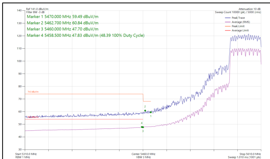
Figure 539 - 802.11ax HE40, SU, CDD, Core 0 - Core 1 - 5590 MHz Band Edge Frequency 5470 MHz
