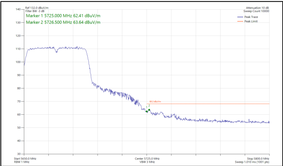
Figure 500 - 802.11n HT40, SISO, Core 0 - 5670 MHz Band Edge Frequency 5725 MHz
