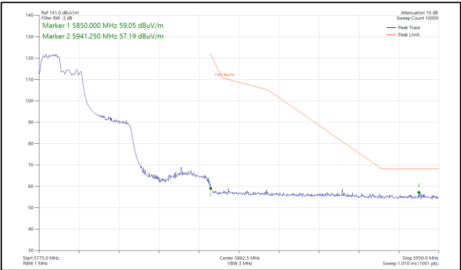
Figure 510 - 802.11ax HE40, RU 106-53, SISO, Core 0 - 5795 MHz Band Edge Frequency 5850 MHz
