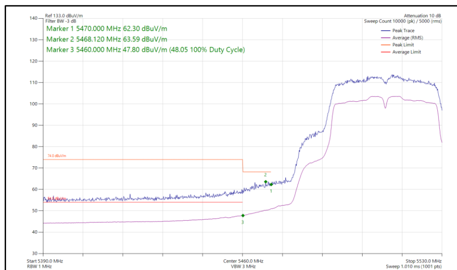
Figure 511 - 802.11n HT40, SISO, Core 1 - 5510 MHz Band Edge Frequency 5470 MHz
