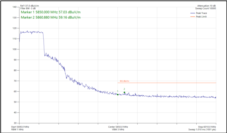
Figure 528 - 802.11ax HE40, SU, SISO, Core 1 - 5710 MHz Band Edge Frequency 5850 MHz
