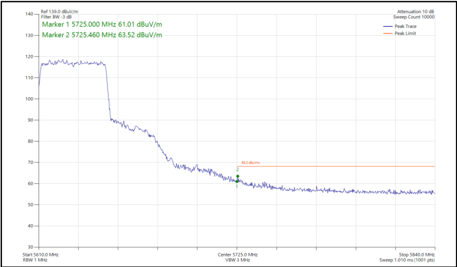
Figure 567 - 802.11ax HE40, SU, SDM, Core 0 - Core 1 - 5630 MHz Band Edge Frequency 5725 MHz
