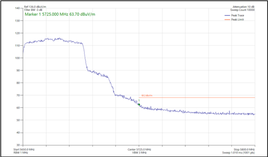
Figure 503 - 802.11ax HE40, SU, SISO, Core 0 - 5670 MHz Band Edge Frequency 5725 MHz
