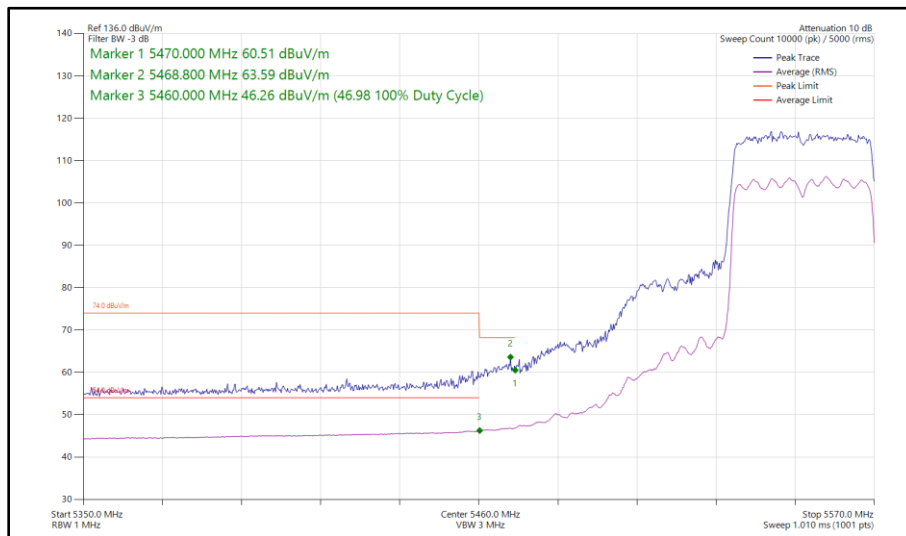
Figure 559 - 802.11ax HE40, SU, SDM, Core 0 - Core 1 - 5550 MHz Band Edge Frequency 5470 MHz
