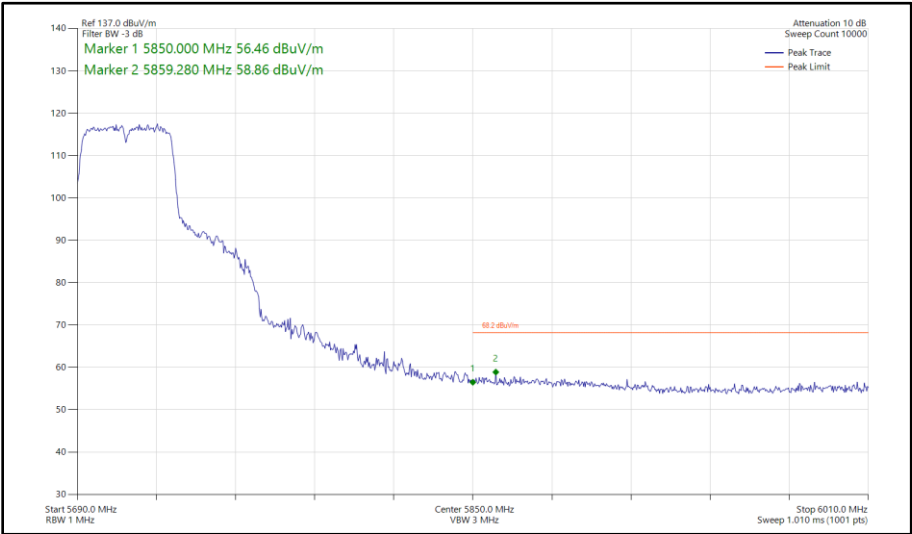
Figure 526 - 802.11n HT40, SISO, Core 1 - 5710 MHz Band Edge Frequency 5850 MHz
