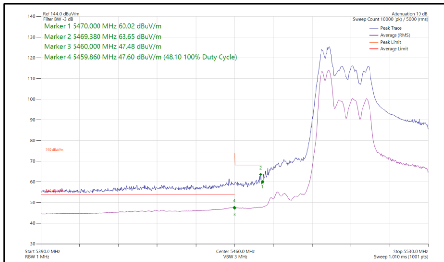
Figure 536 - 802.11ax HE40, RU 52-37, CDD, Core 0 - Core 1 - 5510 MHz Band Edge Frequency 5470 MHz
