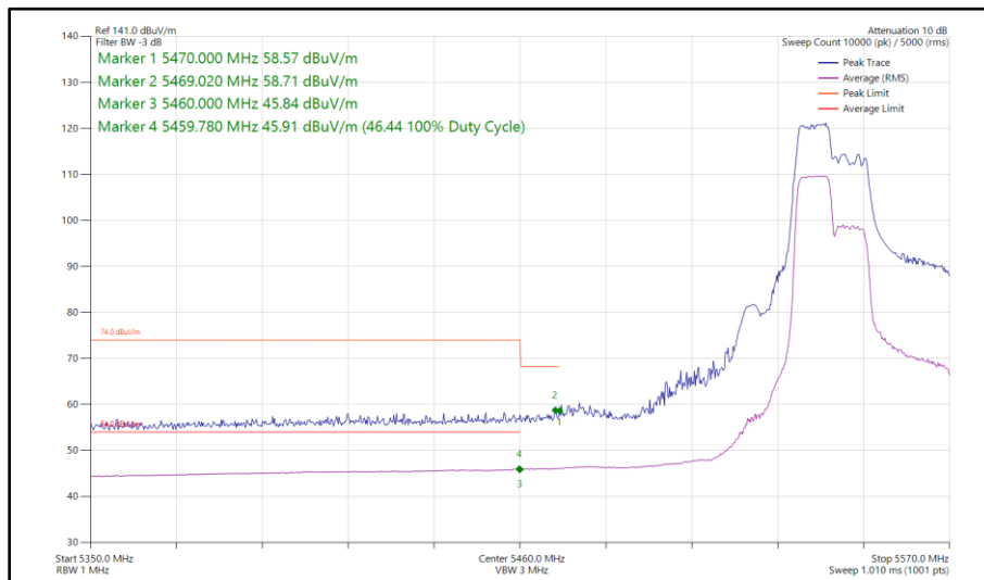
Figure 516 - 802.11ax HE40, RU 106-53, SISO, Core 1 - 5550 MHz Band Edge Frequency 5470 MHz
