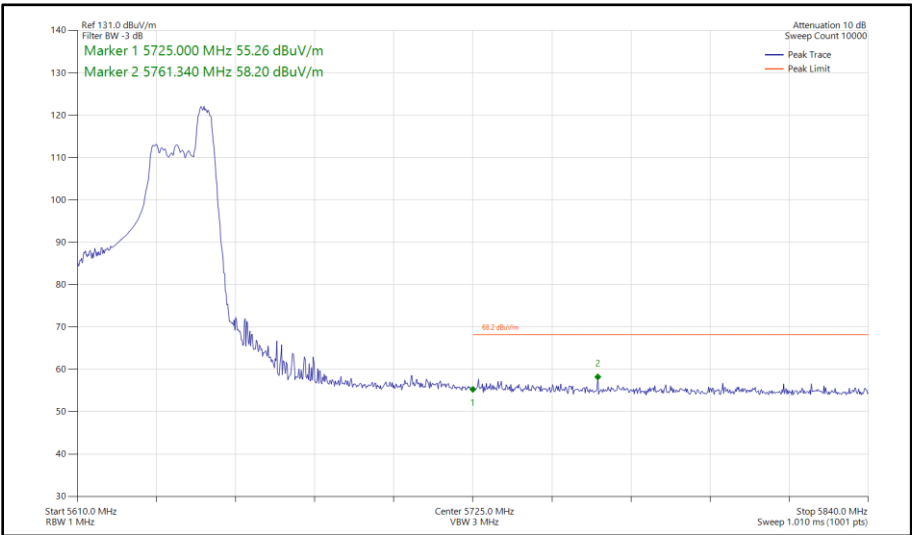
Figure 523 - 802.11ax HE40, RU 52-44, SISO, Core 1 - 5630 MHz Band Edge Frequency 5725 MHz
