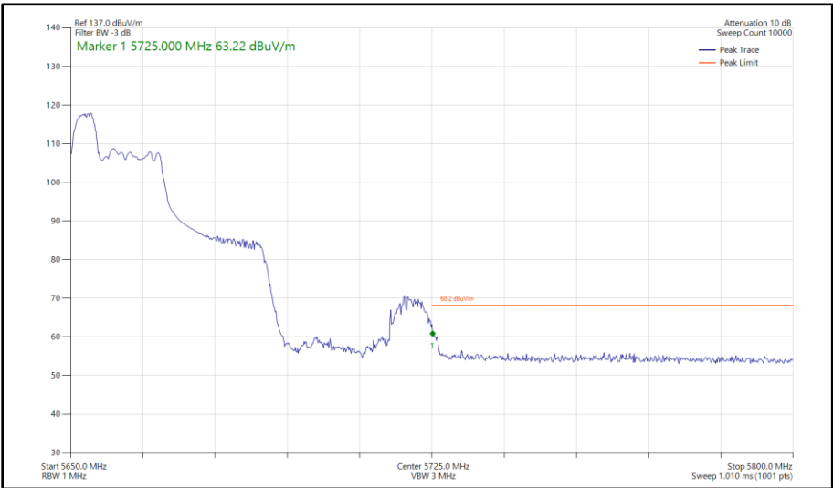
Figure 525 - 802.11ax HE40, RU 52-37, SISO, Core 1 - 5670 MHz Band Edge Frequency 5725 MHz
