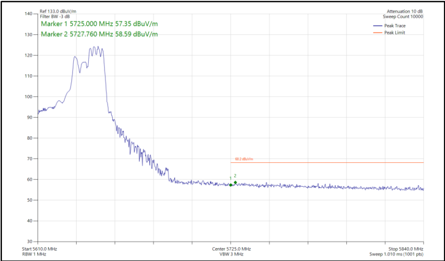
Figure 546 - 802.11ax HE40, RU 106-56, CDD, Core 0 - Core 1 - 5630 MHz Band Edge Frequency 5725 MHz
