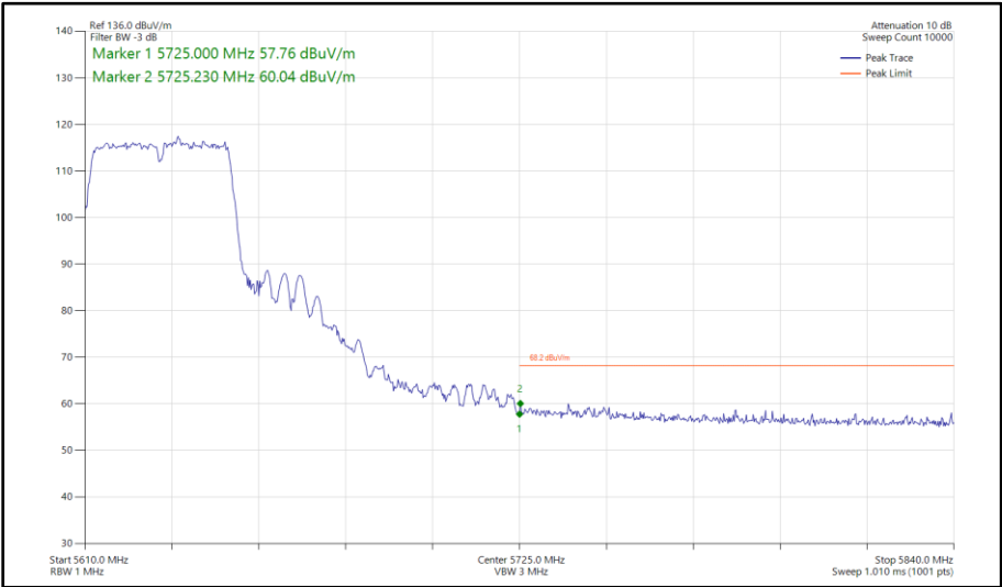
Figure 565 - 802.11n HT40, SDM, Core 0 - Core 1 - 5630 MHz Band Edge Frequency 5725 MHz
