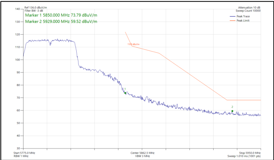
Figure 506 - 802.11n HT40, SISO, Core 0 - 5795 MHz Band Edge Frequency 5850 MHz
