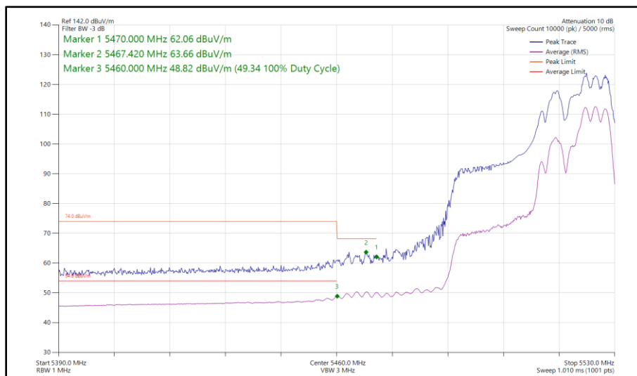
Figure 558 - 802.11ax HE40, RU 106-56, SDM, Core 0 - Core 1 - 5510 MHz Band Edge Frequency 5470 MHz
