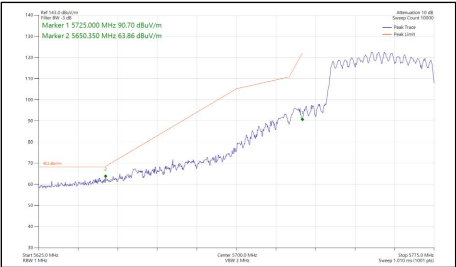
Figure 541 - 802.11ax HE40, SU, CDD, Core 0 - Core 1 - 5755 MHz Band Edge Frequency 5725 MHz
