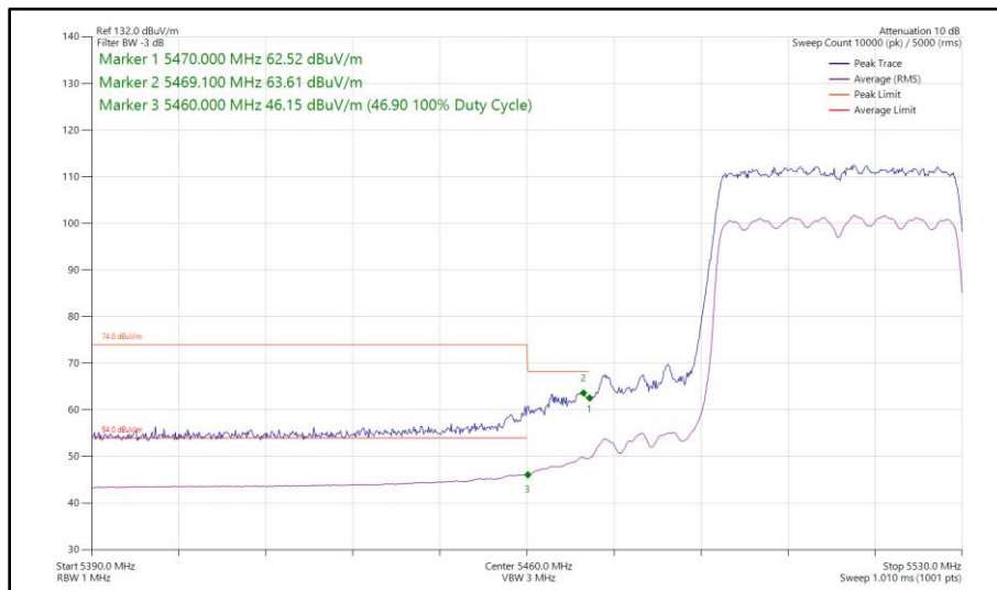
Figure 557 - 802.11ax HE40, SU, SDM, Core 0 - Core 1 - 5510 MHz Band Edge Frequency 5470 MHz
