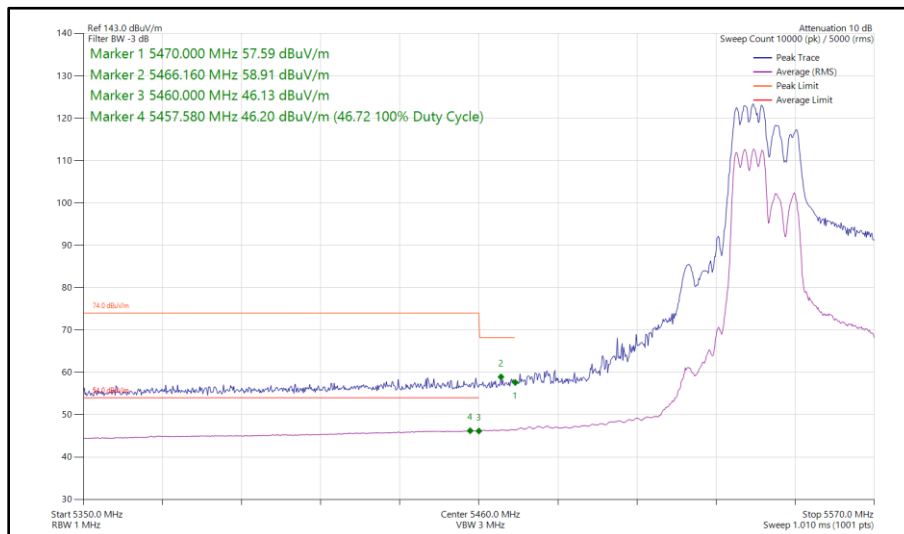
Figure 538 - 802.11ax HE40, RU 106-53, CDD, Core 0 - Core 1 - 5550 MHz Band Edge Frequency 5470 MHz
