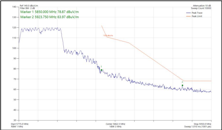
Figure 550 - 802.11n HT40, CDD, Core 0 - Core 1 - 5795 MHz Band Edge Frequency 5850 MHz
