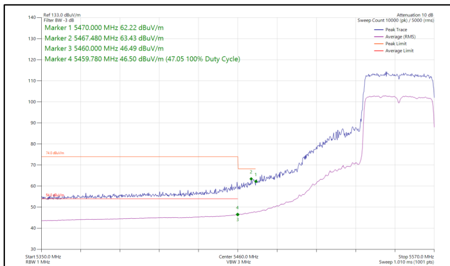
Figure 494 - 802.11ax HE40, SU, SISO, Core 0 - 5550 MHz Band Edge Frequency 5470 MHz
