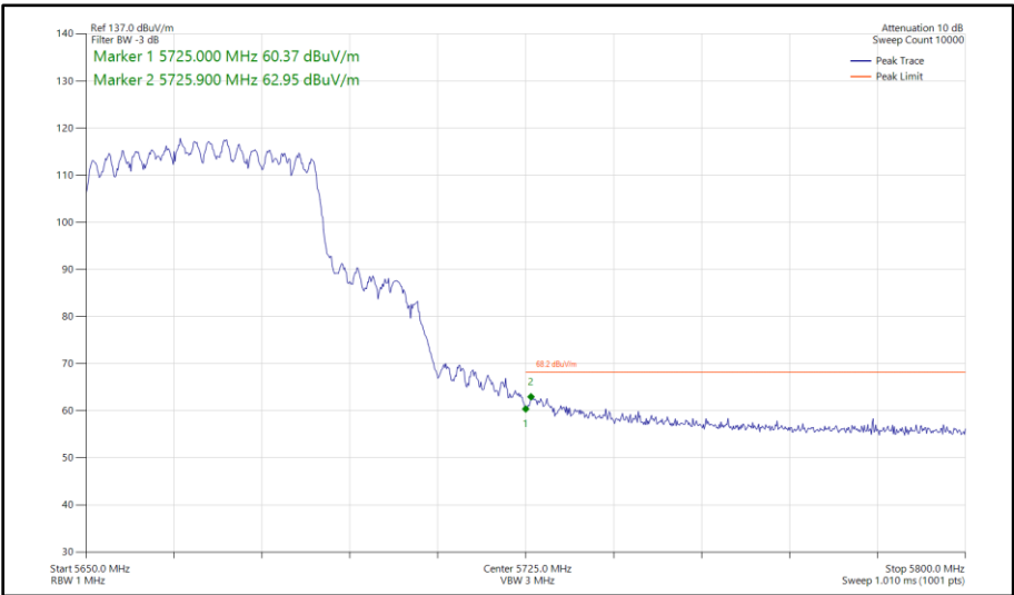
Figure 547 - 802.11ax HE40, SU, CDD, Core 0 - Core 1 - 5670 MHz Band Edge Frequency 5725 MHz
