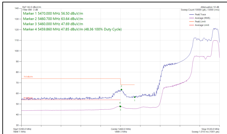
Figure 514 - 802.11ax HE40, RU 52-44, SISO, Core 1 - 5510 MHz Band Edge Frequency 5470 MHz
