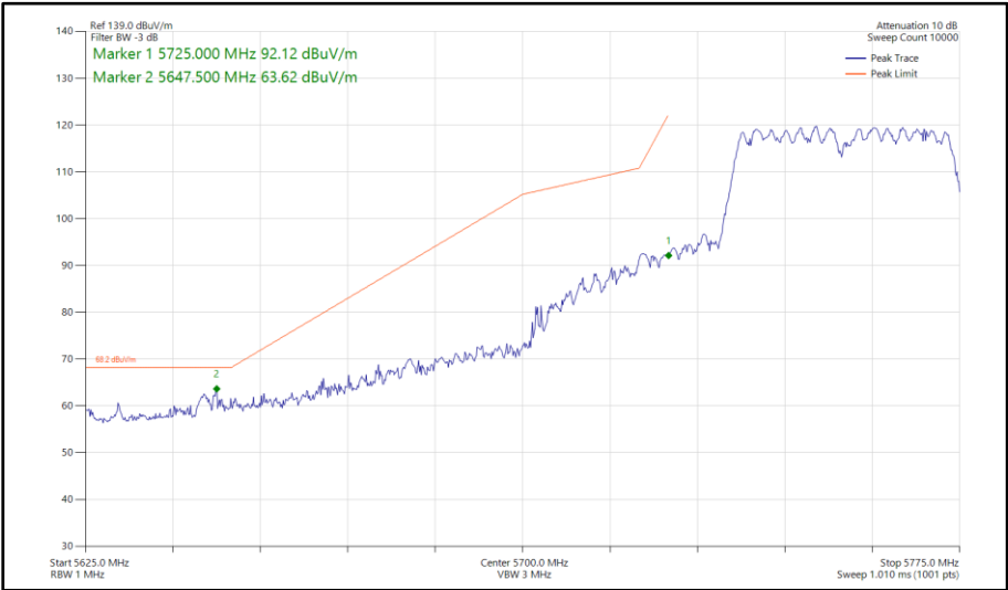
Figure 540 - 802.11n HT40, CDD, Core 0 - Core 1 - 5755 MHz Band Edge Frequency 5725 MHz
