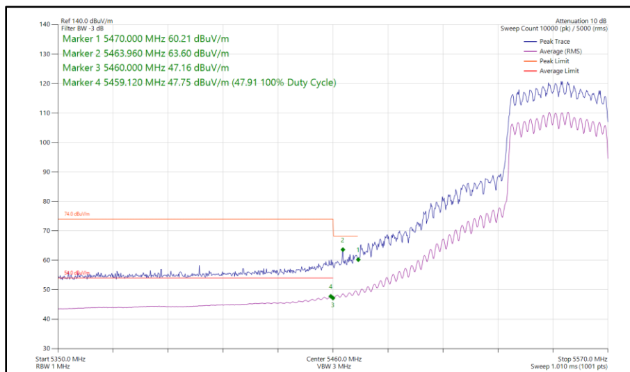
Figure 537 - 802.11ax HE40, SU, CDD, Core 0 - Core 1 - 5550 MHz Band Edge Frequency 5470 MHz
