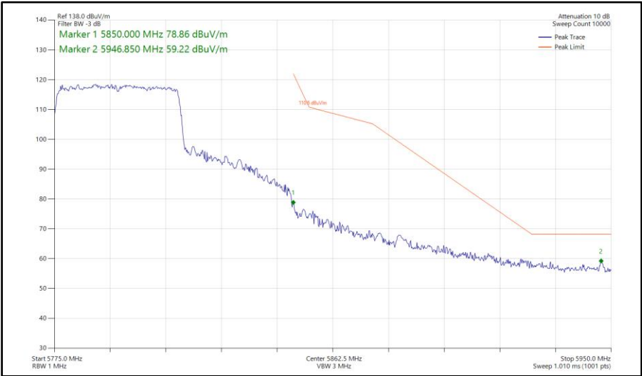
Figure 530 - 802.11ax HE40, SU, SISO, Core 1 - 5795 MHz Band Edge Frequency 5850 MHz
