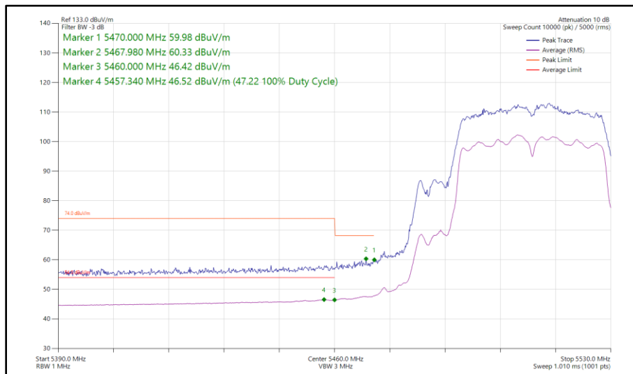
Figure 555 - 802.11n HT40, SDM, Core 0 - Core 1 - 5510 MHz Band Edge Frequency 5470 MHz
