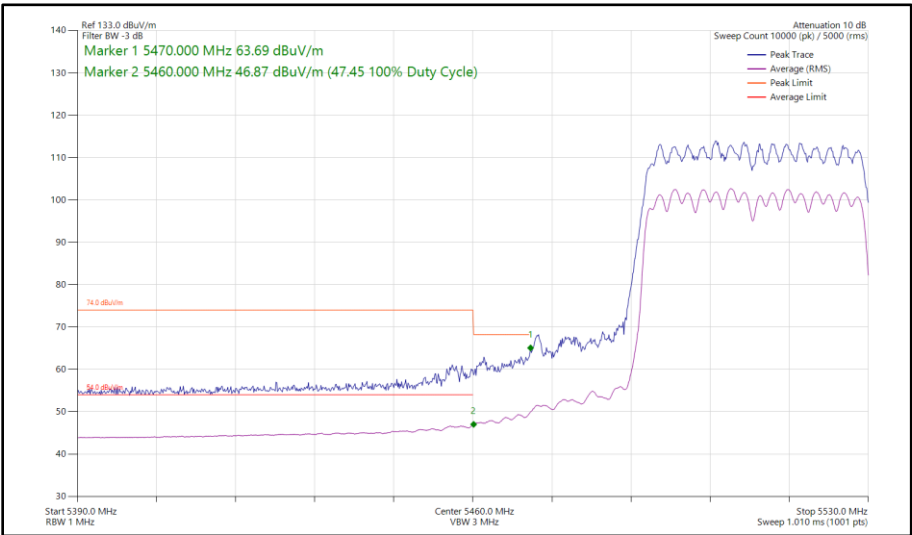
Figure 535 - 802.11ax HE40, SU, CDD, Core 0 - Core 1 - 5510 MHz Band Edge Frequency 5470 MHz
