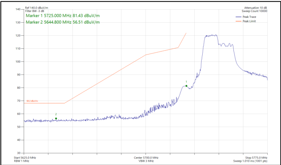
Figure 498 - 802.11ax HE40, RU 106-53, SISO, Core 0 - 5755 MHz Band Edge Frequency 5725 MHz
