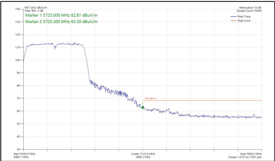
Figure 521 - 802.11n HT40, SISO, Core 1 - 5670 MHz Band Edge Frequency 5725 MHz
