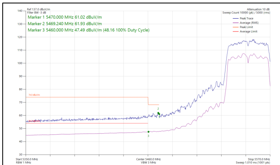
Figure 556 - 802.11n HT40, SDM, Core 0 - Core 1 - 5550 MHz Band Edge Frequency 5470 MHz
