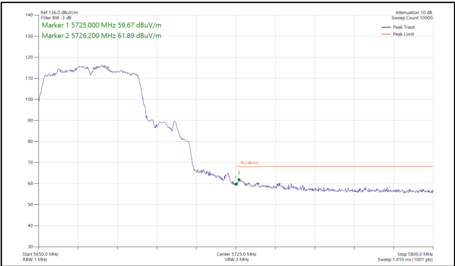
Figure 566 - 802.11n HT40, SDM, Core 0 - Core 1 - 5670 MHz Band Edge Frequency 5725 MHz
