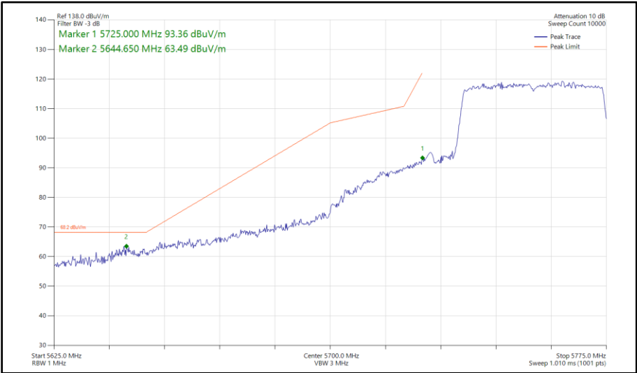
Figure 563 - 802.11ax HE40, SU, SDM, Core 0 - Core 1 - 5755 MHz Band Edge Frequency 5725 MHz
