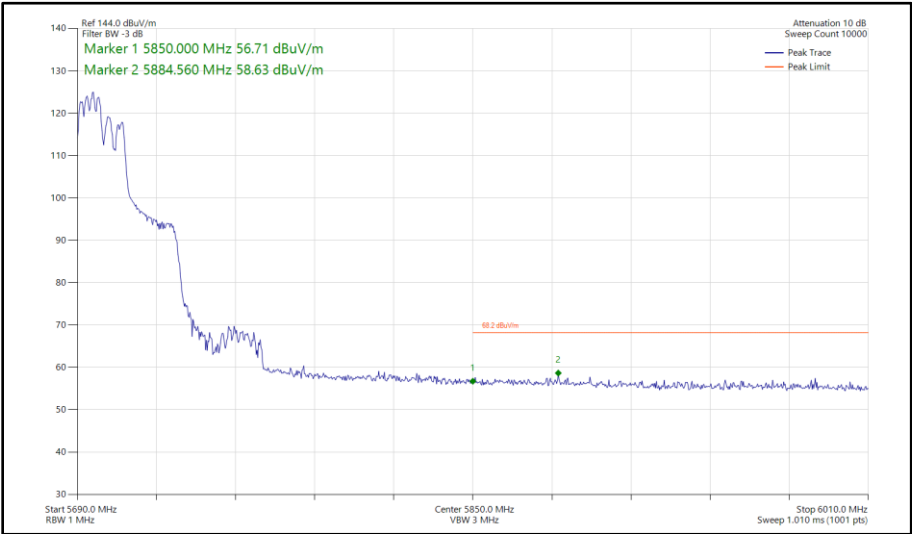
Figure 552 - 802.11ax HE40, RU 106-53, CDD, Core 0 - Core 1 - 5710 MHz Band Edge Frequency 5850 MHz
