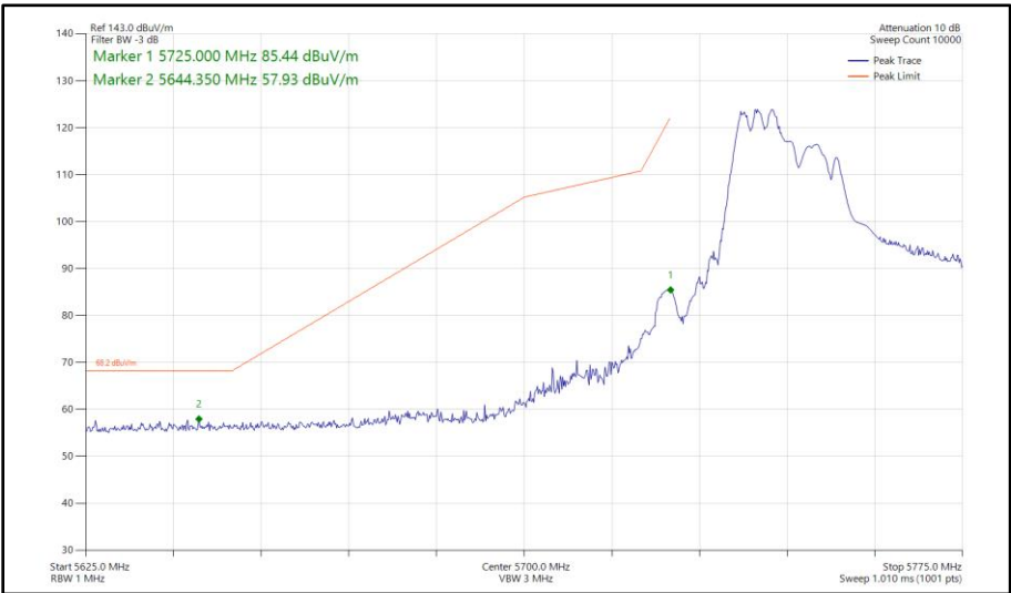
Figure 564 - 802.11ax HE40, RU 106-53, SDM, Core 0 - Core 1 - 5755 MHz Band Edge Frequency 5725 MHz
