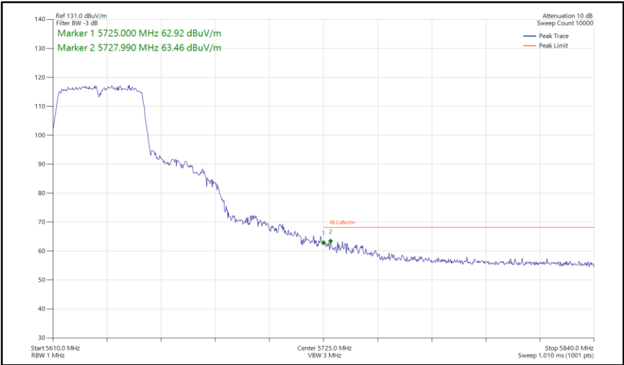
Figure 520 - 802.11n HT40, SISO, Core 1 - 5630 MHz Band Edge Frequency 5725 MHz
