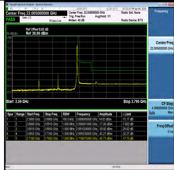
NTNV-N41-PC2-30-60-H-CP-QPSK-Edge_1RB_Right-Ant2-PASS
