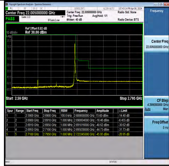
NTNV-N41-PC2-30-60-H-CP-QPSK-Edge_1RB_Right-Ant1-PASS
