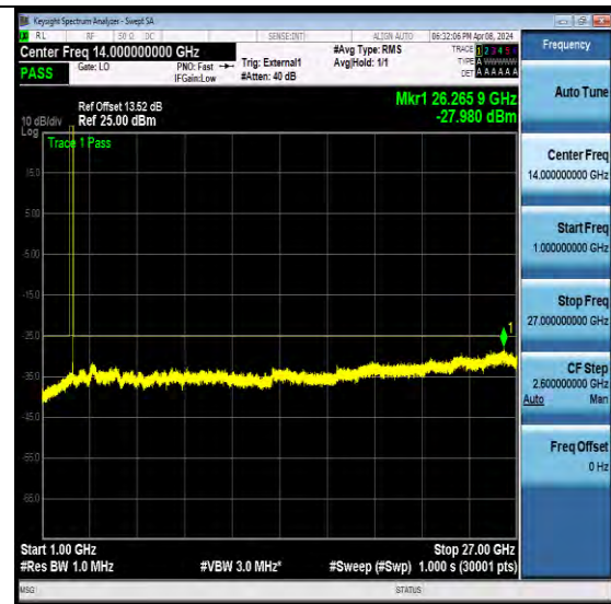
NTNV-N41-PC2-30-20-H-CP-QPSK-Edge_1RB_Left-Ant2-P ASS
