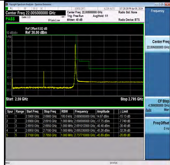
NTNV-N41-PC2-30-100-H-CP-QPSK-Edge_1RB_Right-Ant2-PASS
