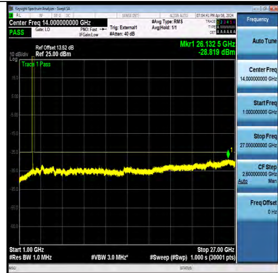
NTNV-N41-PC2-30-100-H-CP-QPSK-Edge_1RB_Left-Ant1- PASS
