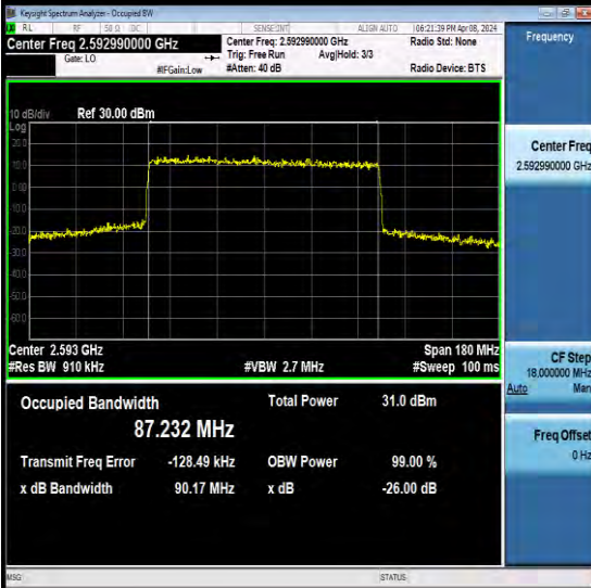
NTNV-N41-PC2-30-90-M-CP-64QAM-Outer_Full-Ant1-PASS
