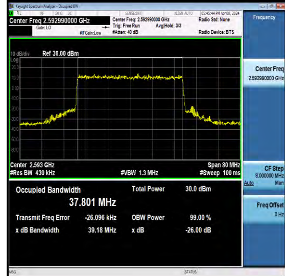
NTNV-N41-PC2-30-40-M-CP-256QAM-Outer_Full-Ant2-PASS
