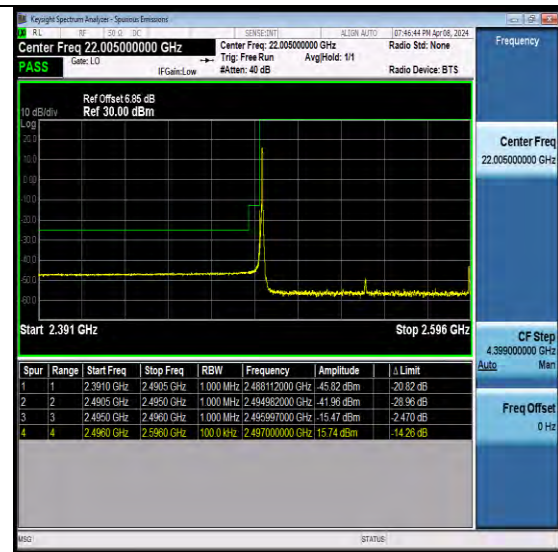
NTNV-N41-PC2-30-100-L-CP-QPSK-Edge_1RB_Left-Ant1-PASS
