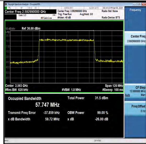
NTNV-N41-PC2-30-60-M-CP-16QAM-Outer Full-Ant1-PASS
