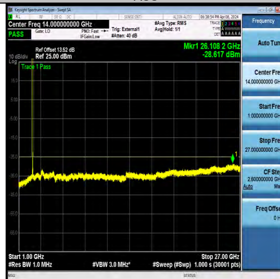
NTNV-N41-PC2-30-60-H-CP-QPSK-Edge_1RB_Left-Ant2-P ASS
