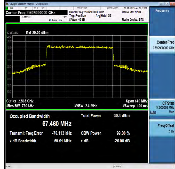
NTNV-N41-PC2-30-70-M-CP-256QAM-Outer_Full-Ant2-PASS
