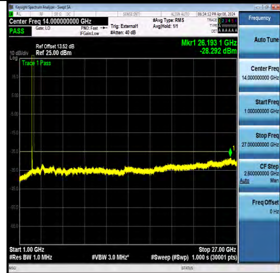
NTNV-N41-PC2-30-60-L-CP-QPSK-Edge_1RB_Left-Ant2-P SS
