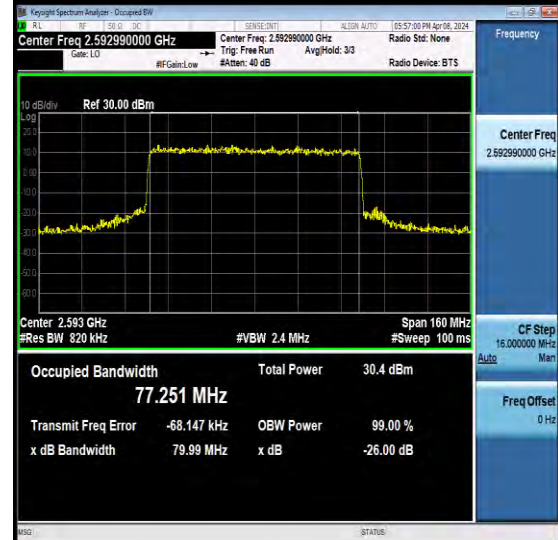
NTNV-N41-PC2-30-80-M-CP-256QAM-Outer_Full-Ant2-PASS
