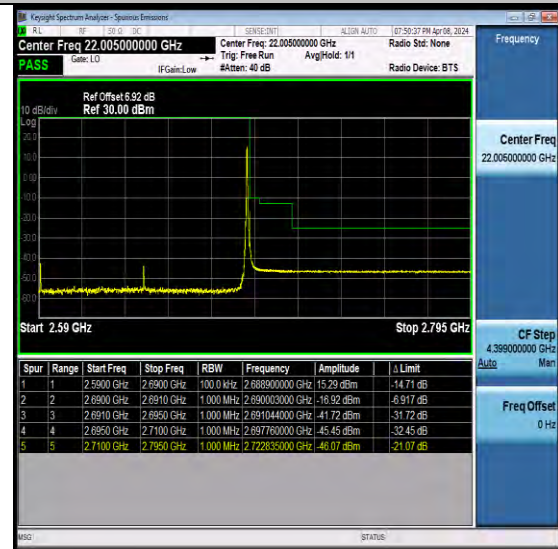
NTNV-N41-PC2-30-100-H-CP-QPSK-Edge_1RB_Right-Ant1-PASS
