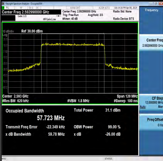
NTNV-N41-PC2-30-60-M-CP-64QAM-Outer_Full-Ant1-PASS
