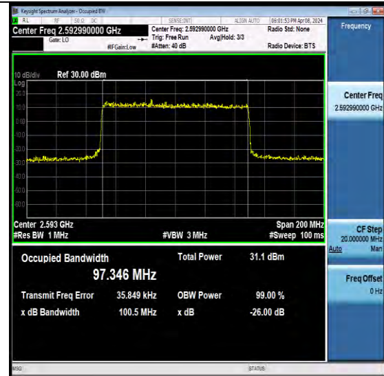
NTNV-N41-PC2-30-100-M-CP-16QAM-Outer_Full-Ant2-PASS
