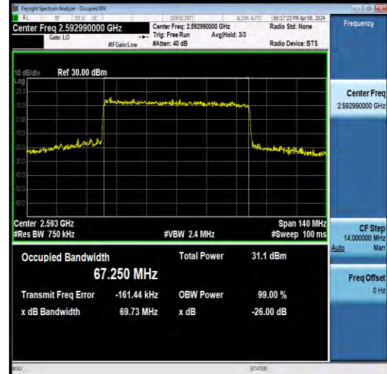
NTNV-N41-PC2-30-70-M-CP-256QAM-Outer_Full-Ant1-PASS
