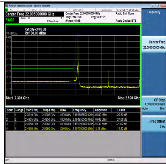
NTNV-N41-PC2-30-100-L-CP-QPSK-Edge_1RB_Left-Ant2-PASS
