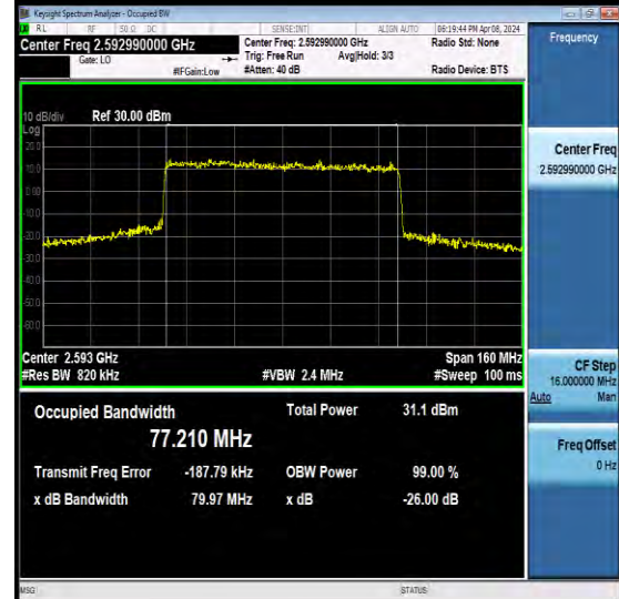
NTNV-N41-PC2-30-80-M-CP-256QAM-Outer_Full-Ant1-PASS
