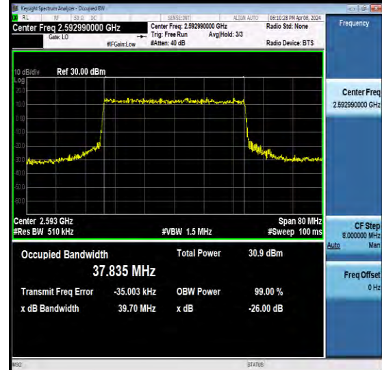
NTNV-N41-PC2-30-40-M-CP-256QAM-Outer_Full-Ant1-PASS
