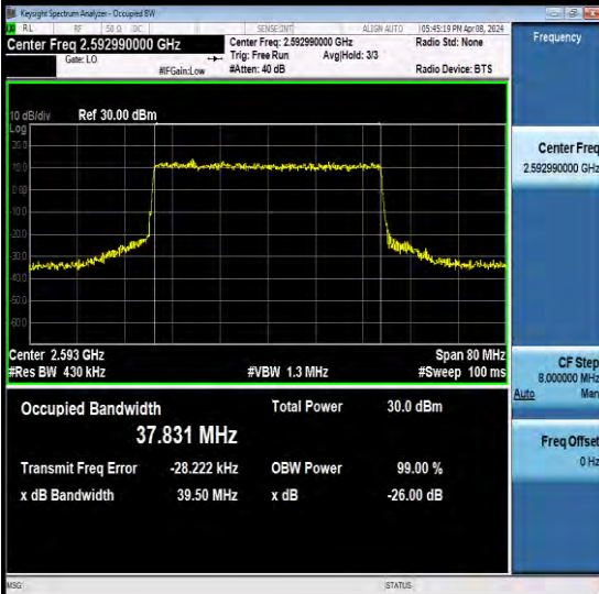
NTNV-N41-PC2-30-40-M-CP-QPSK-Outer Full-Ant2-PASS
