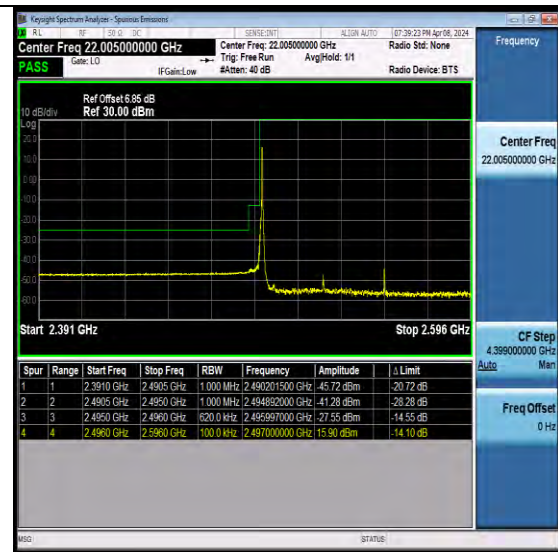
NTNV-N41-PC2-30-60-L-CP-QPSK-Edge_1RB_Left-Ant1-PASS
