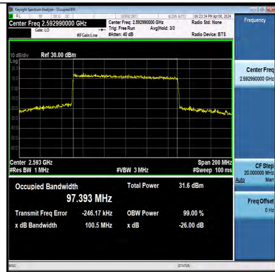
NTNV-N41-PC2-30-100-M-CP-16QAM-Outer_Full-Ant1-PASS
