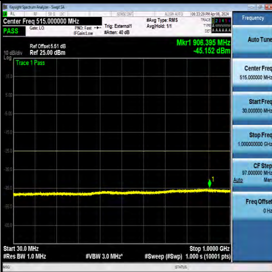
NTNV-N41-PC2-30-60-L-CP-QPSK-Edge_1RB_Left-Ant2-P SS
