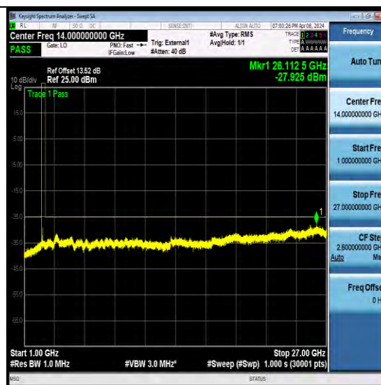
NTNV-N41-PC2-30-100-L-CP-QPSK-Edge_1RB_Left-Ant1-P ASS
