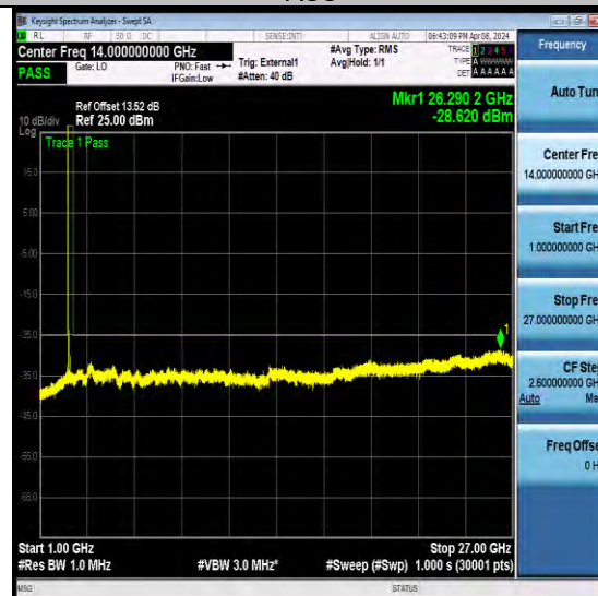
NTNV-N41-PC2-30-100-M-CP-QPSK-Edge_1RB_Left-Ant2- PASS
