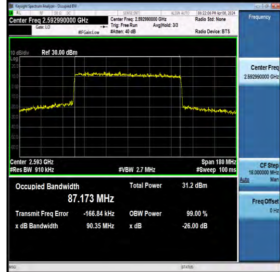
NTNV-N41-PC2-30-90-M-CP-256QAM-Outer_Full-Ant1-PASS
