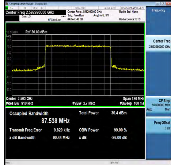
NTNV-N41-PC2-30-90-M-CP-256QAM-Outer_Full-Ant2-PASS
