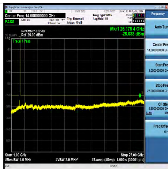
NTNV-N41-PC2-30-100-L-CP-QPSK-Edge_1RB_Left-Ant2-P ASS
