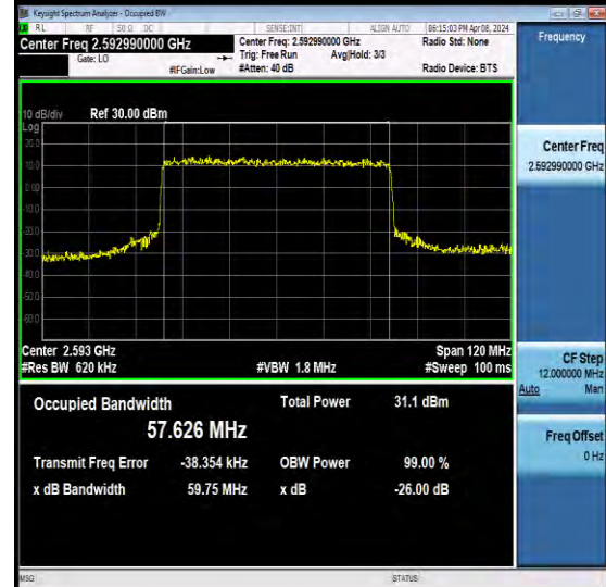
NTNV-N41-PC2-30-60-M-CP-256QAM-Outer_Full-Ant1-PASS
