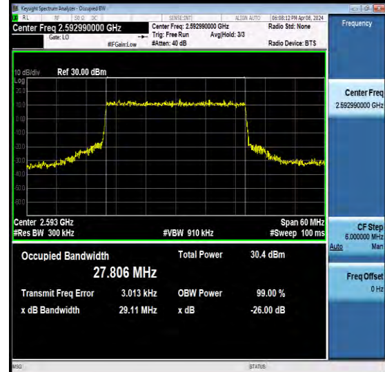
NTNV-N41-PC2-30-30-M-CP-256QAM-Outer_Full-Ant1-PASS
