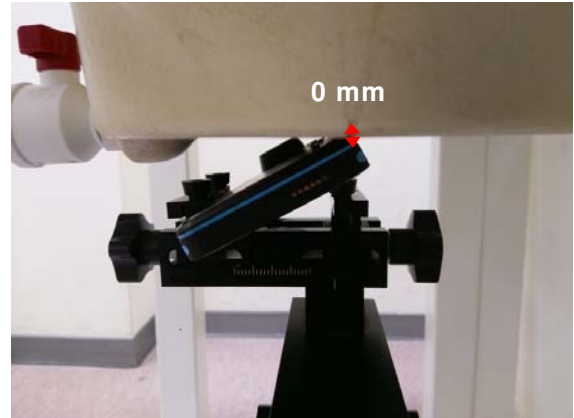
Fig.16 EUT Back side_WLAN to flat phantom
