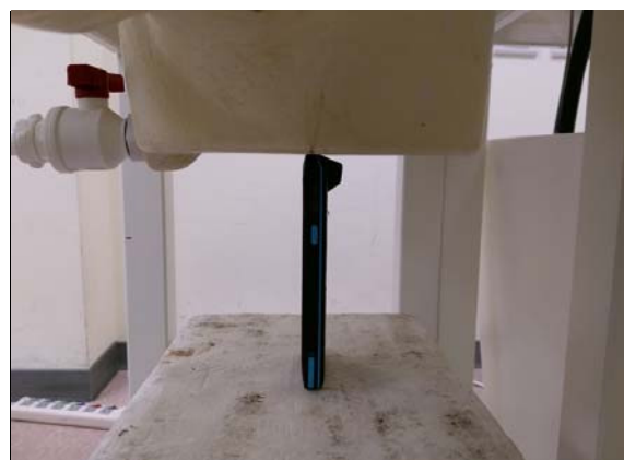
Fig.19 EUT Top side to flat phantom
