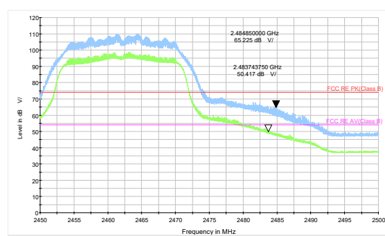
802.11n HT20-Channel 11 Peak+ Average
