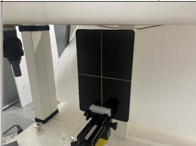
Right Side of EUT with 0.9 cm Gap
