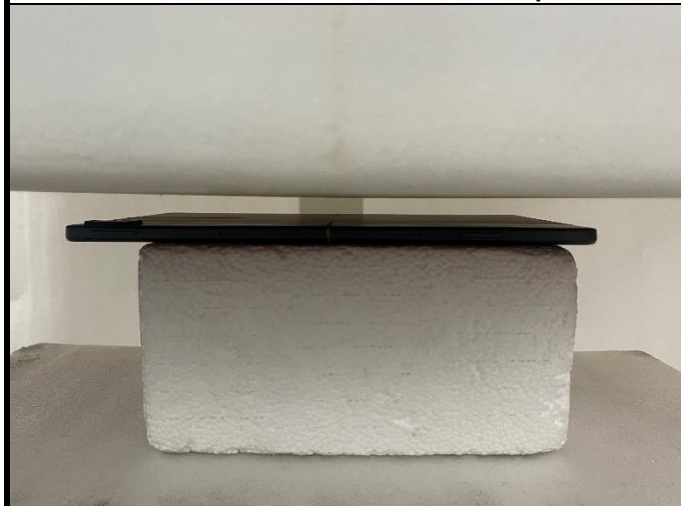
Rear Face of EUT with 1.4 cm Gap
