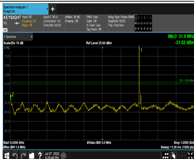
Band17-5MHz-QPSK-23790-1RB#0-Range2:30~1000MHz
