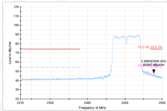
Bandedge-11N(40M)-CH9-AV
