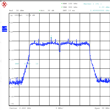
11AC20SISO-Ant1-2462-0~Reference-PASS
