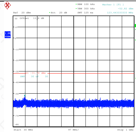
11AX40SISO-Ant1-2437-30~1000-PASS
