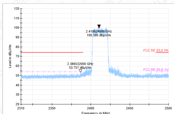
Bandedge-11AC-CH1-PK
