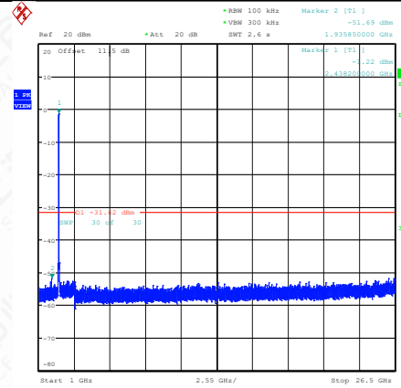
11AX40SISO-Ant1-2422-1000~26500-PASS
