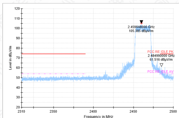
Bandedge-11AC-CH11-PK
