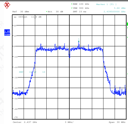
11AC20SISO-Ant1-2437-0~Reference-PASS
