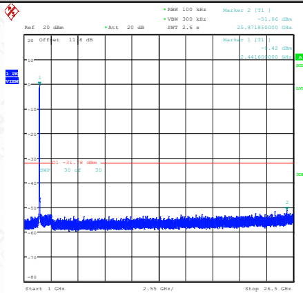
11AX40SISO-Ant1-2437-1000~26500-PASS
