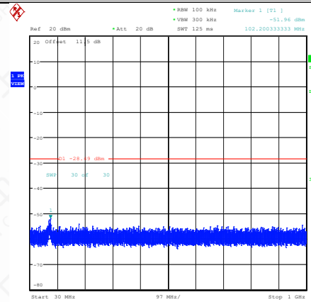
11AC20SISO-Ant1-2412-30~1000-PASS
