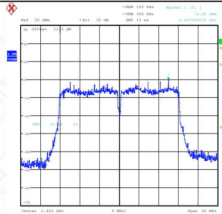
11AC40SISO-Ant1-2422-0~Reference-PASS
