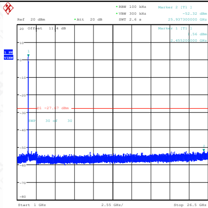
11AC20SISO-Ant1-2462-1000~26500-PASS
