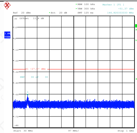
11AC20SISO-Ant1-2462-30~1000-PASS
