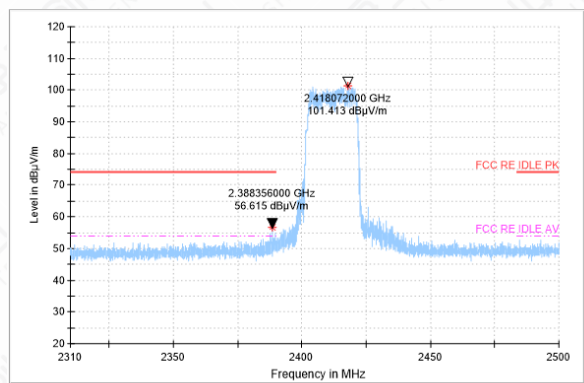
Bandedge-11AX-CH1-PK
