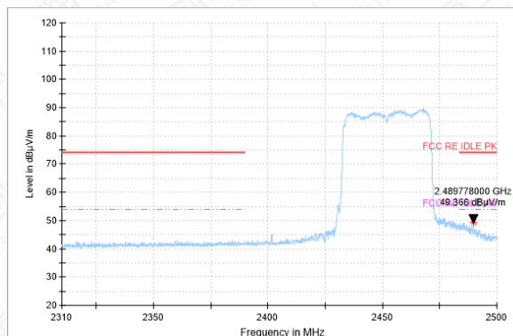
Bandedge-11AX(40M)-CH9-AV
