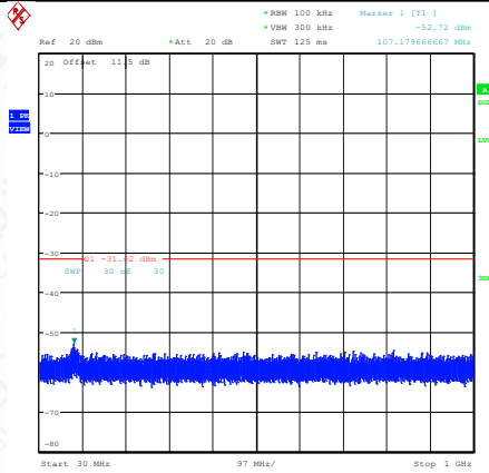
11AX40SISO-Ant1-2422-30~1000-PASS
