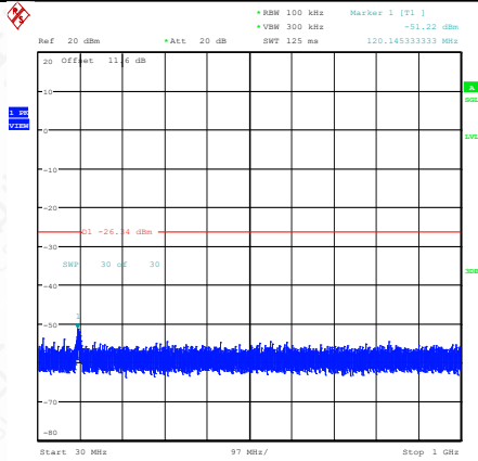
11AC20SISO-Ant1-2437-30~1000-PASS
