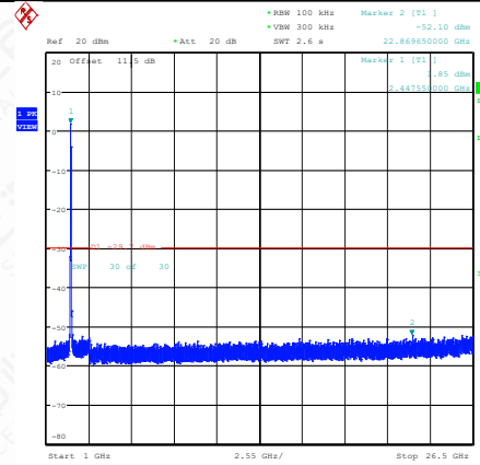
11N40SISO-Ant1-2452-1000~26500-PASS
