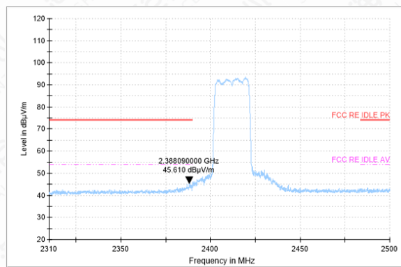
Bandedge-11AX-CH1-AV
