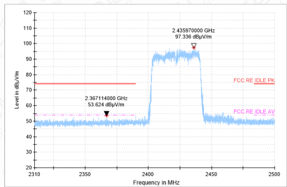
Bandedge-11AX(40M)-CH3-PK
