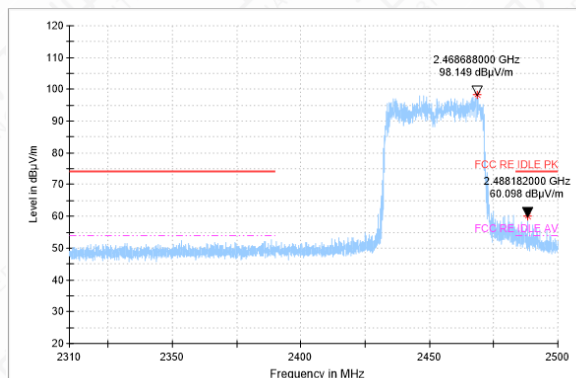
Bandedge-11AX(40M)-CH9-PK
