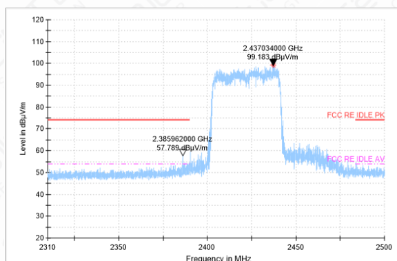
Bandedge-11AC(40M)-CH3-PK
