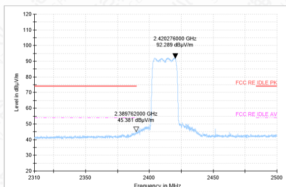
Bandedge-11AC-CH1-AV
