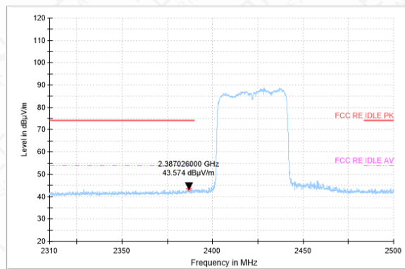
Bandedge-11AX(40M)-CH3-AV
