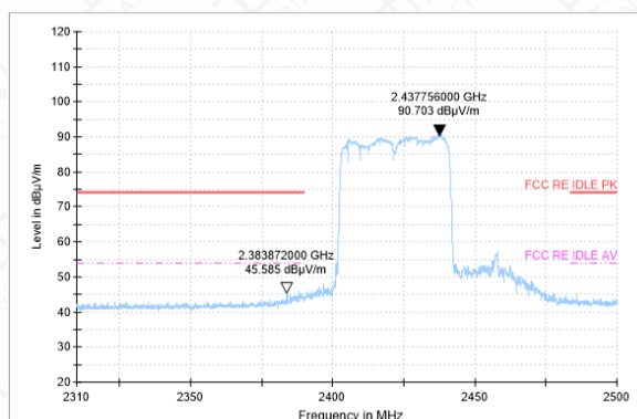
Bandedge-11AC(40M)-CH3-AV
