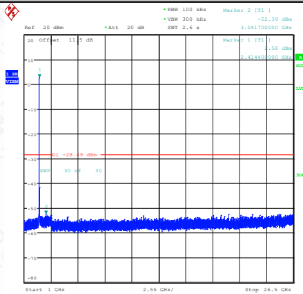
11AC20SISO-Ant1-2412-1000~26500-PASS
