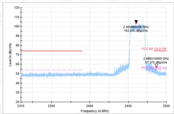
Bandedge-11AX-CH11-PK
