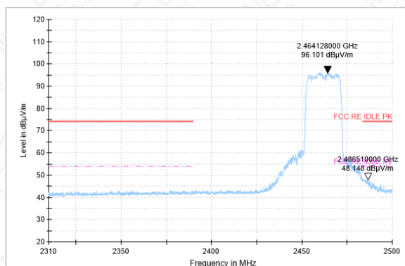
Bandedge-11AC-CH11-AV
