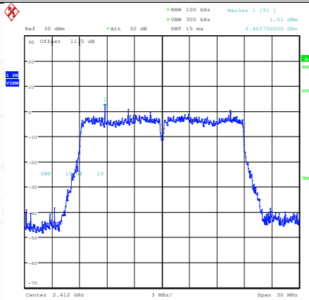
11AC20SISO-Ant1-2412-0~Reference-PASS
