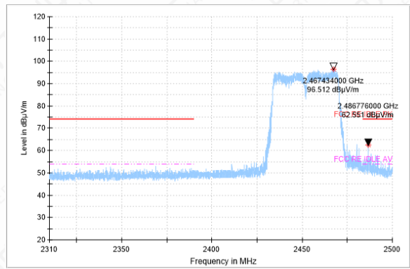
Bandedge-11N(40M)-CH9-PK
