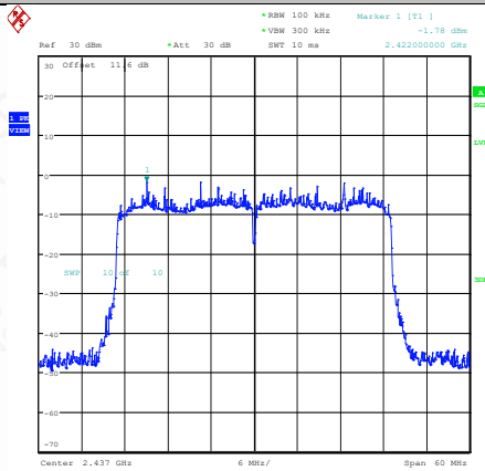
11AX40SISO-Ant1-2437-0~Reference-PASS
