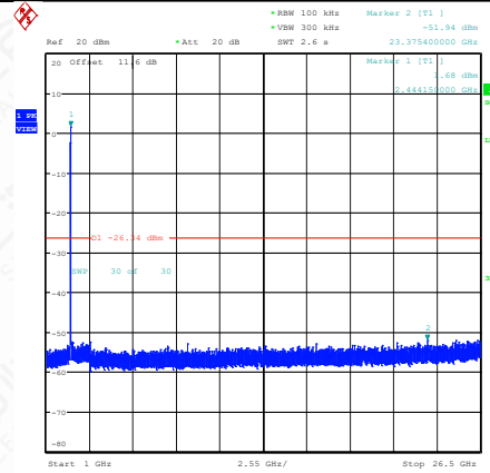
11AC20SISO-Ant1-2437-1000~26500-PASS
