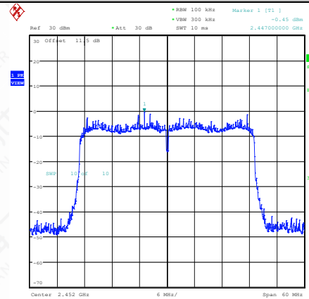
11AX40SISO-Ant1-2452-0~Reference-PASS
