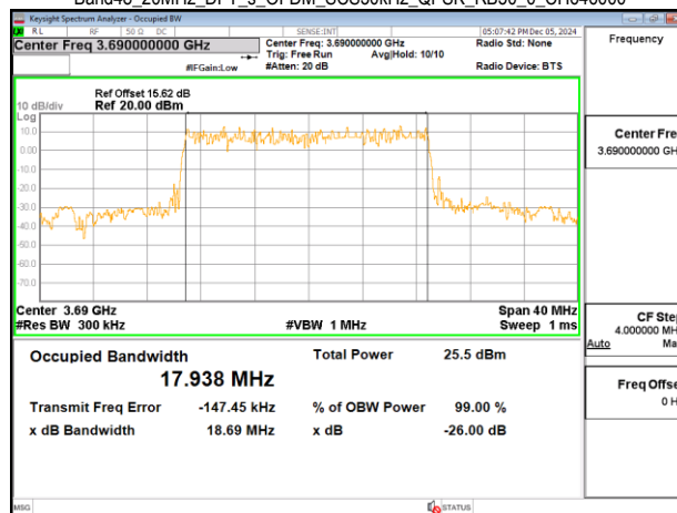
Band48_20MHz_DFT_s_OFDM_SCS30kHz_QPSK_RB50_0_CH646000
