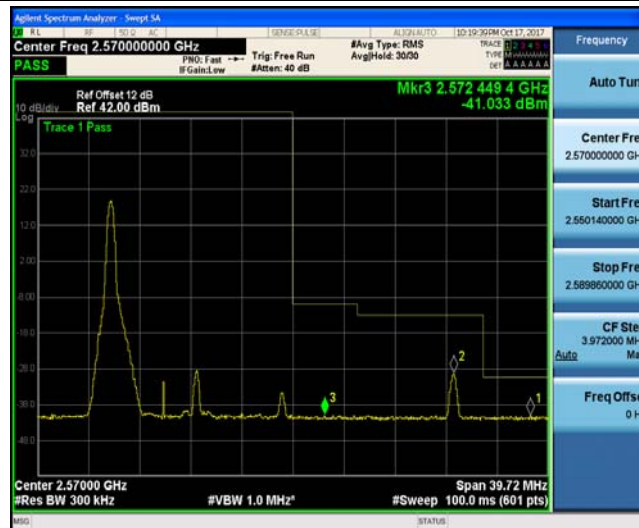
Band7_15MHz_16QAM_21375_1RB#0_-41.02,-29.82,-41.02_PASS
