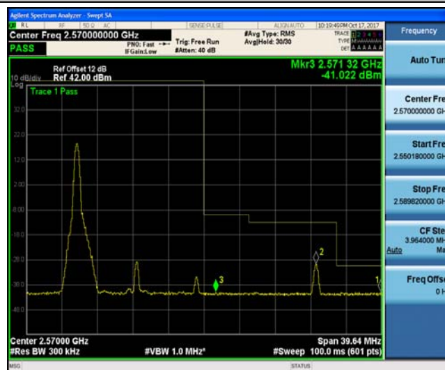
Band7_15MHz_QPSK_21375_75RB#0_-40.83,-36.96,-31.88_PASS
