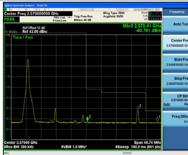
Band7_20MHz_QPSK_21350_100RB#0_-40.92,-37.24,-33.67_PASS
