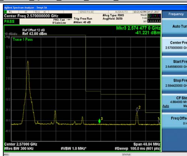
Band7_20MHz_16QAM_21350_1RB#0_-41.22,-30.74,-40.76_PASS
