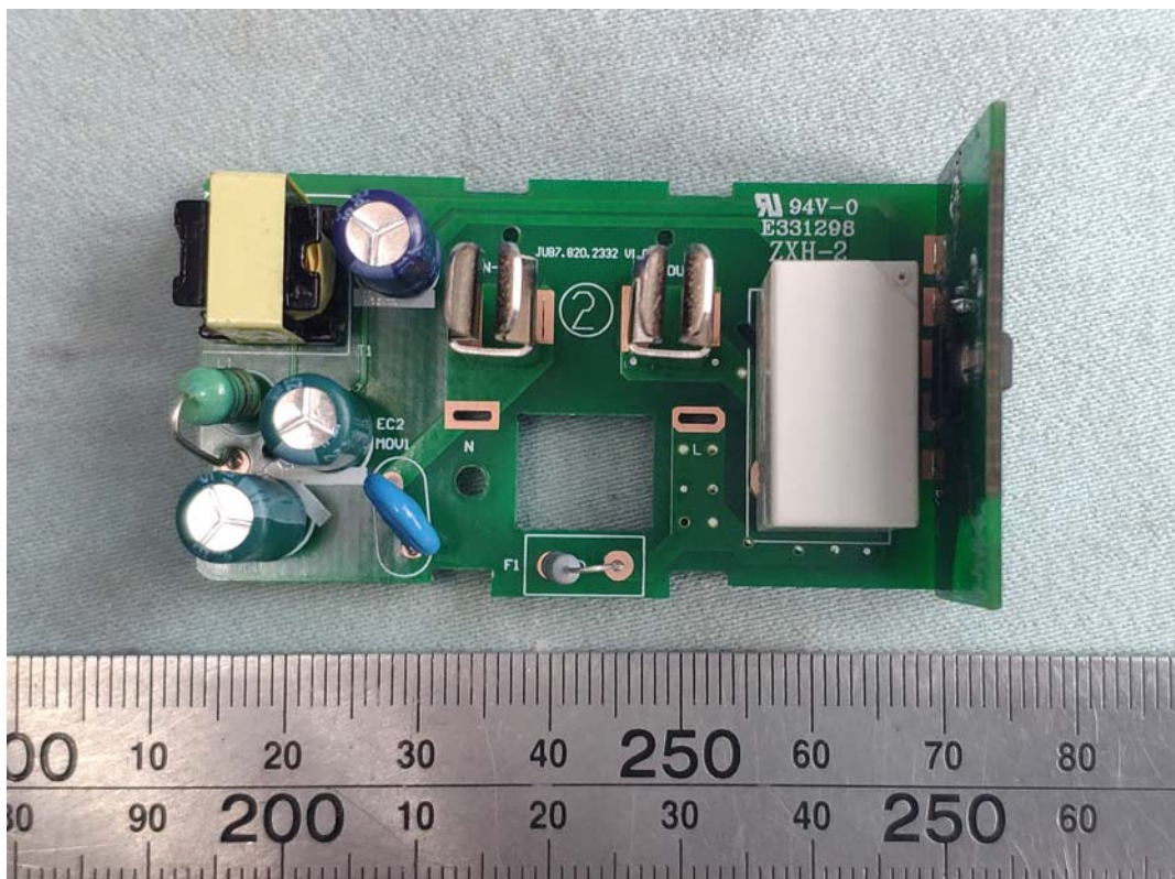
FIGURE 8 SMART PLUG (MODEL: CPLGSTDBLW1)(HVIN: CPLGSTDXCW1T) MAIN BOARD (COMPONENT SIDE)
