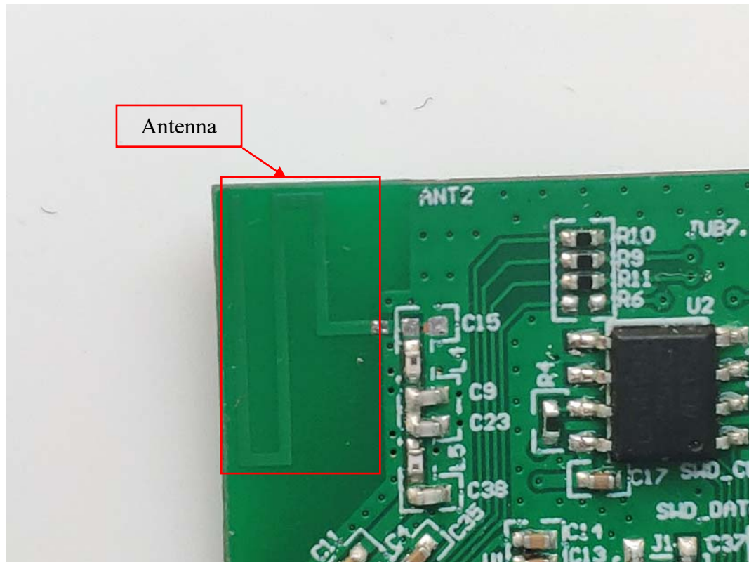
FIGURE 13 SMART PLUG (MODEL: CPLGSTDBLW1)(HVIN: CPLGSTDXCW1T) BT ANT
