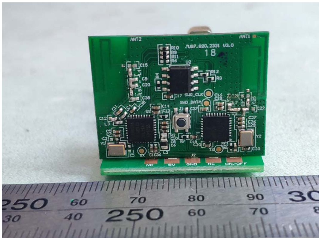
FIGURE 10 SMART PLUG (MODEL: CPLGSTDBLW1)(HVIN: CPLGSTDXCW1T) RF BOARD (COMPONENT SIDE)
