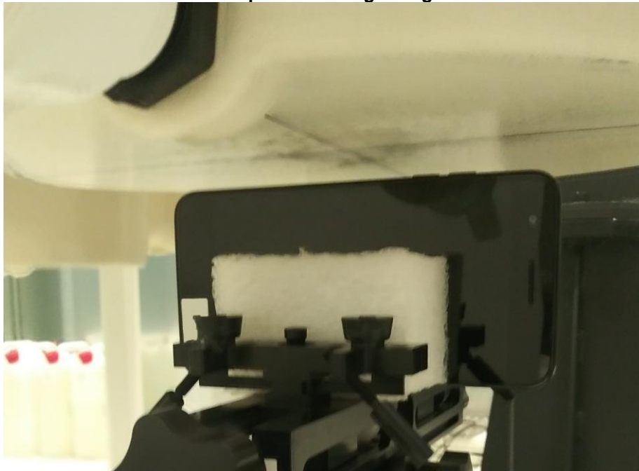
SAR Test Setup Photo 10: Left Edge at 1.0 cm
