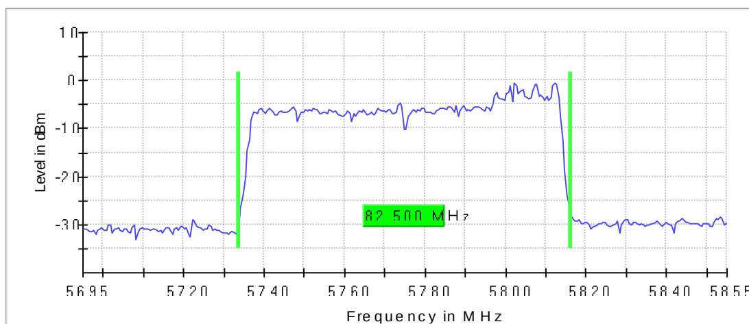
26 dB Bandwidth
