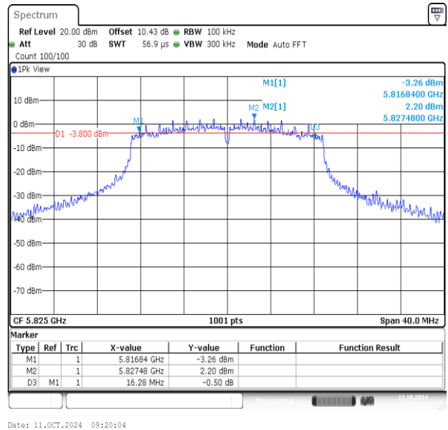
11AC20MIMO-Ant2-5825-PASS
