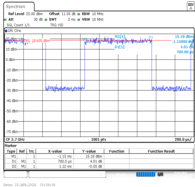
NTNV-11A-Ant2-5700
