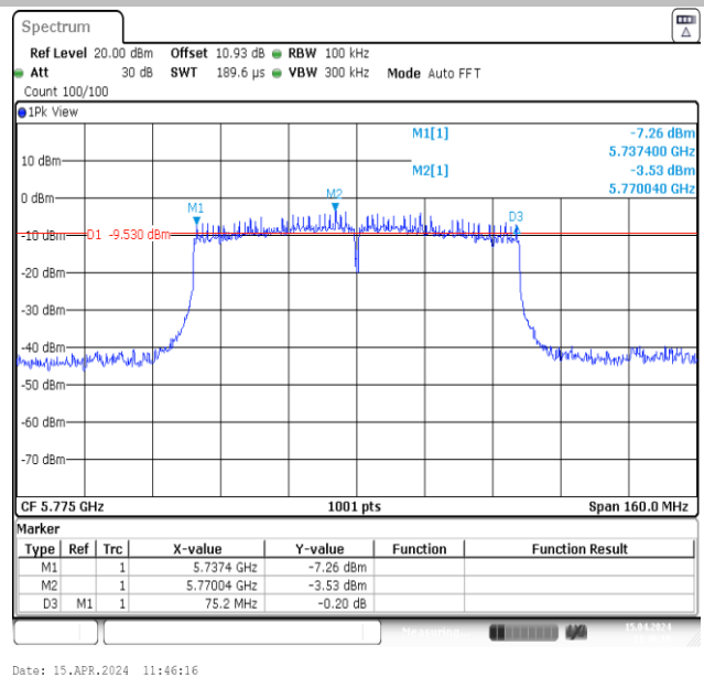
11AC80MIMO-Ant2-5775-PASS
