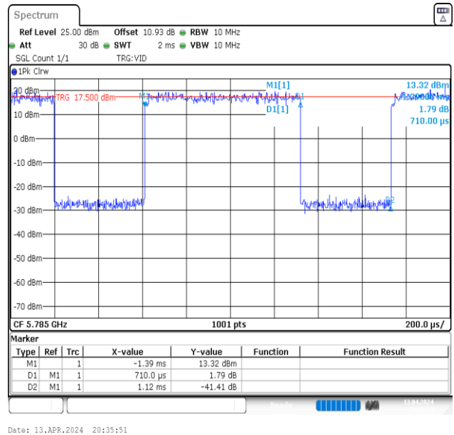
NTNV-11A-Ant2-5785
