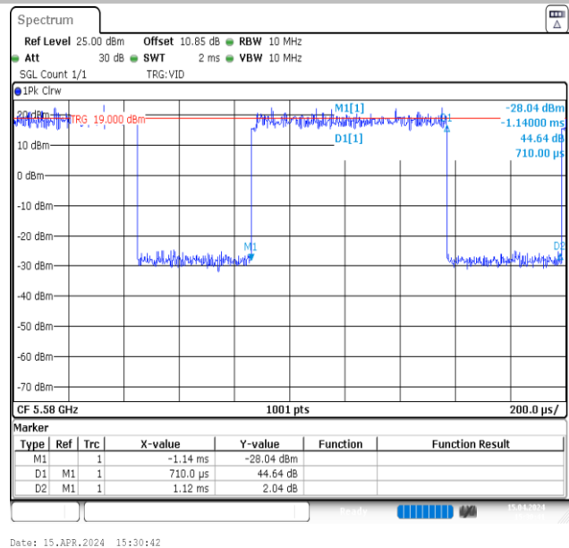
NTNV-11A-Ant2-5580
