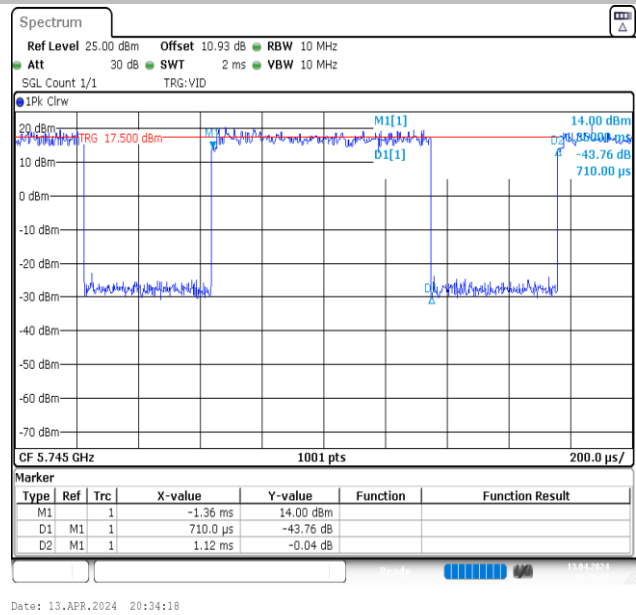
NTNV-11A-Ant2-5745
