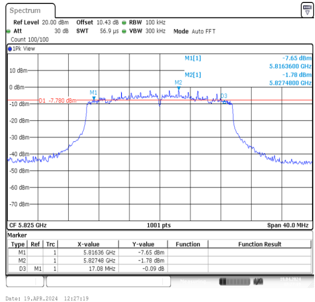
11AX20MIMO-Ant2-5825-PASS
