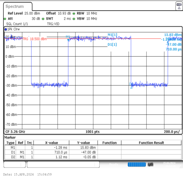
NTNV-11A-Ant2-5260
