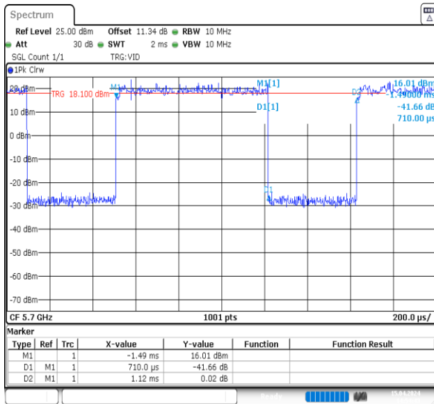
NTNV-11A-Ant1-5700
