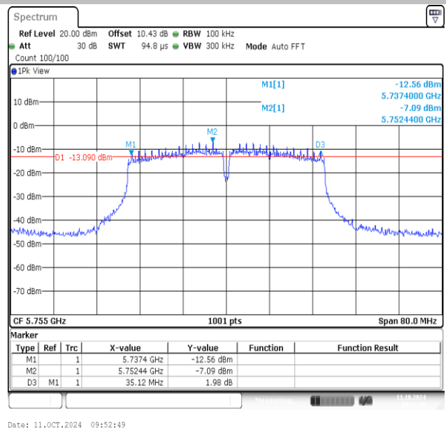
11AC40MIMO-Ant2-5755-PASS
