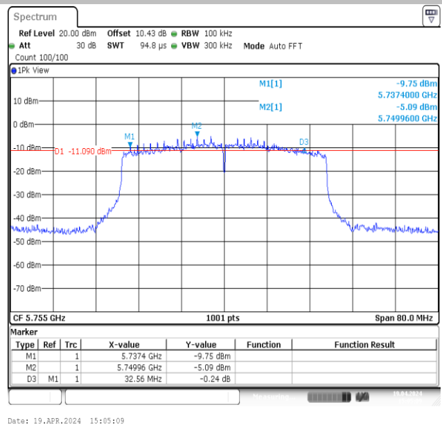
11AX40MIMO-Ant2-5755-PASS
