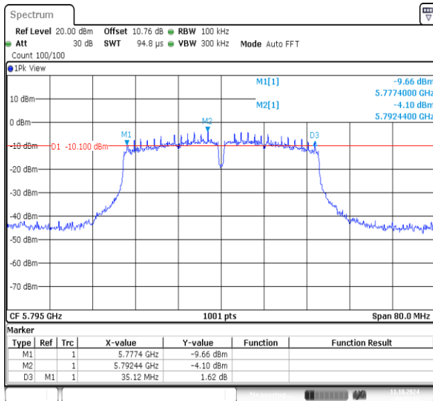
11AC40MIMO-Ant1-5795-PASS
