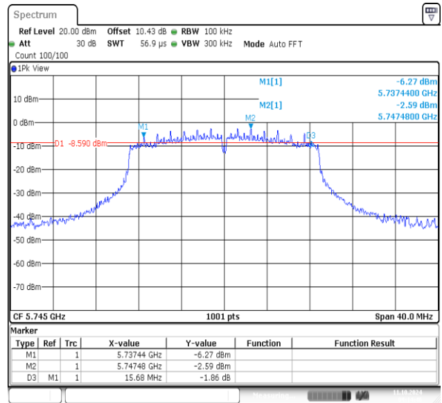
11AC20MIMO-Ant2-5745-PASS
