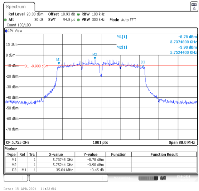
11N40MIMO-Ant2-5755-PASS
