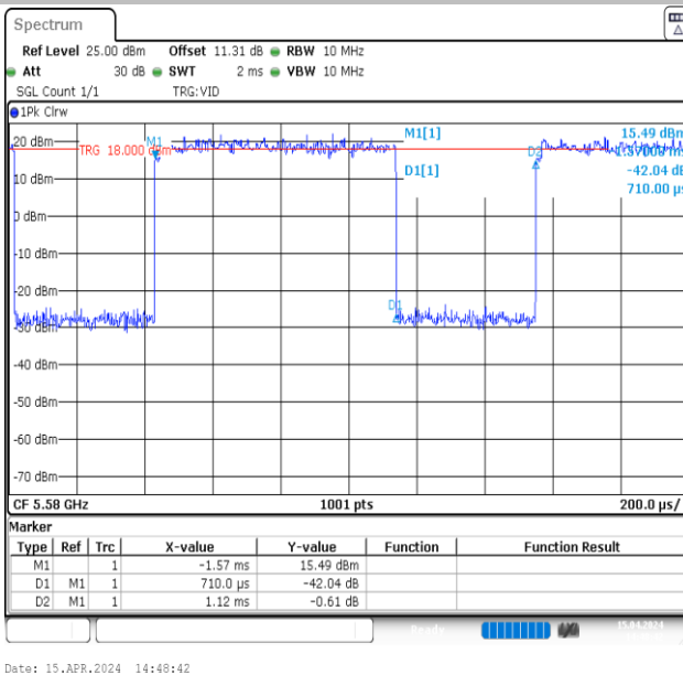
NTNV-11A-Ant1-5580
