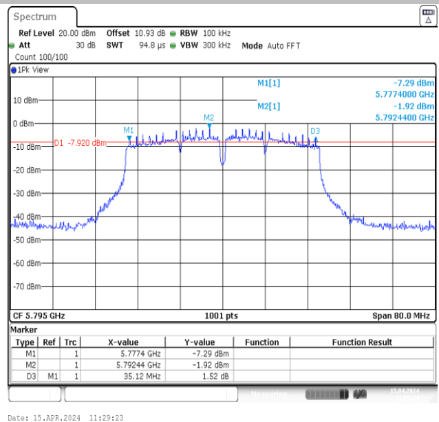
11N40MIMO-Ant2-5795-PASS
