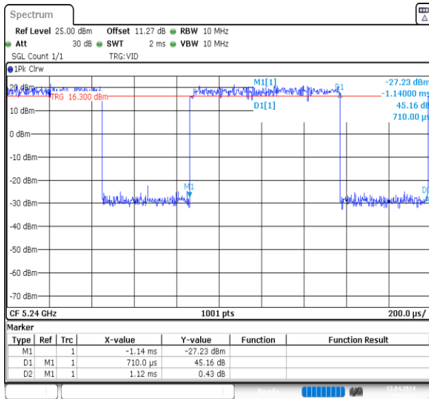
NTNV-11A-Ant1-5240
