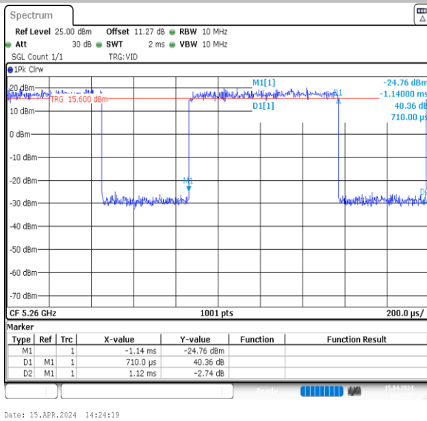
NTNV-11A-Ant1-5260
