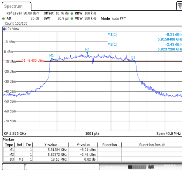
11AX20MIMO-Ant1-5825-PASS
