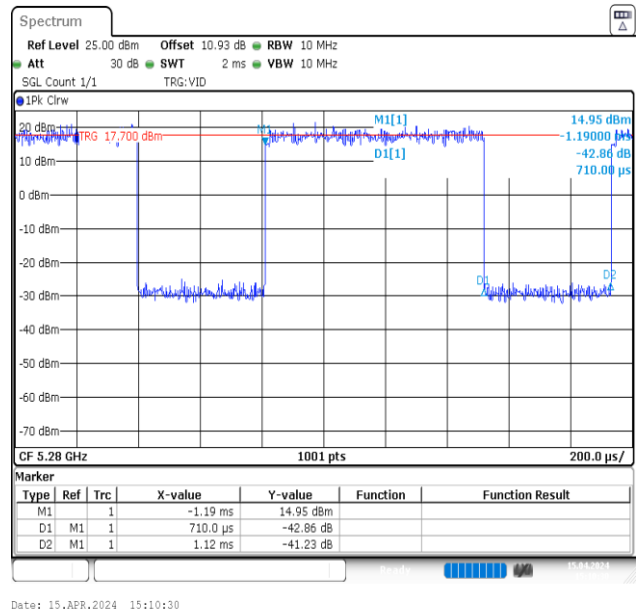
NTNV-11A-Ant2-5280
