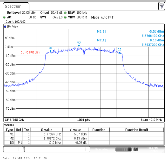
11AX20MIMO-Ant2-5785-PASS
