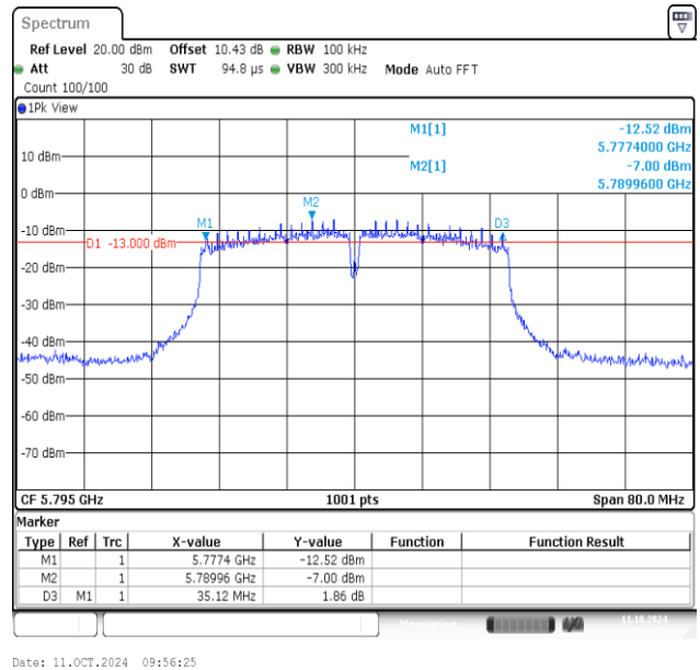
11AC40MIMO-Ant2-5795-PASS
