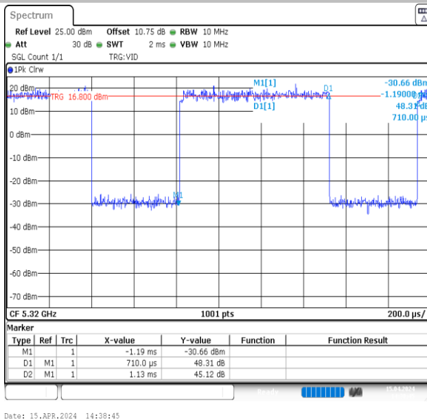
NTNV-11A-Ant1-5320
