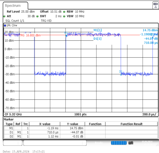
NTNV-11A-Ant2-5320
