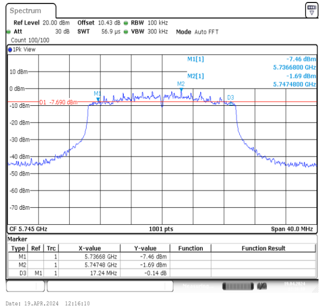
11AX20MIMO-Ant2-5745-PASS
