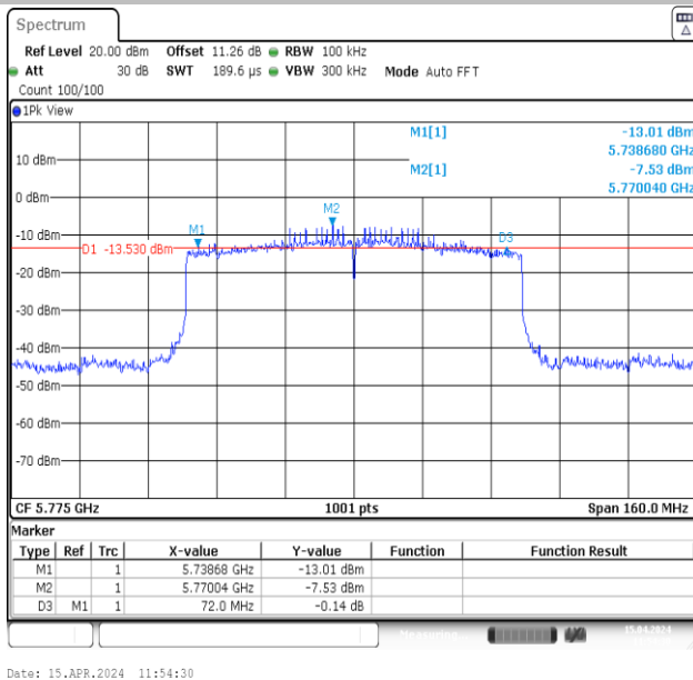
11AX80MIMO-Ant1-5775-PASS
