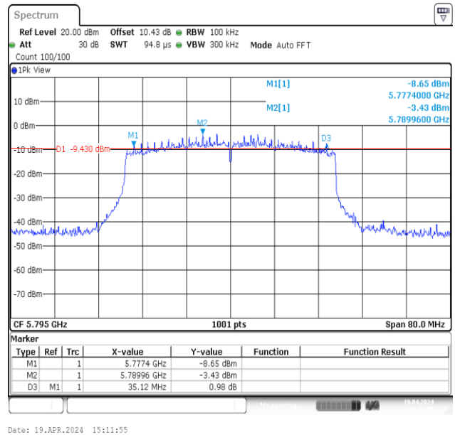
11AX40MIMO-Ant2-5795-PASS
