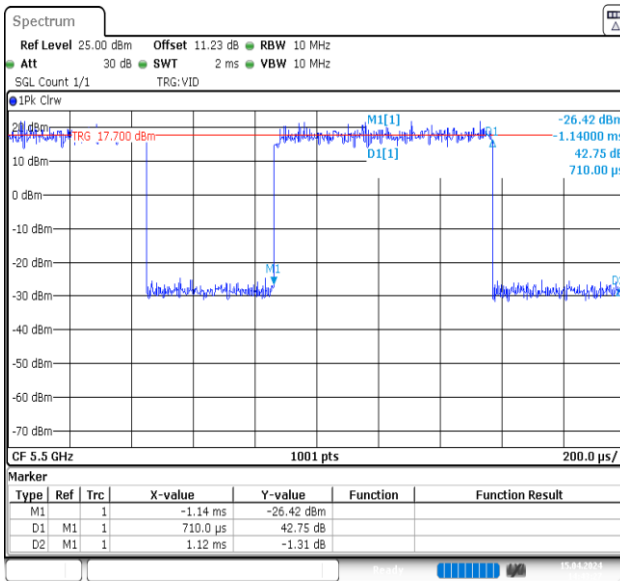
NTNV-11A-Ant1-5500
