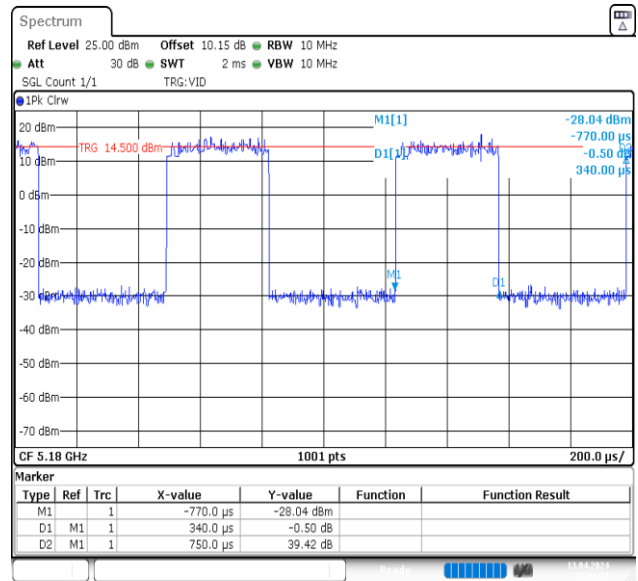
NTNV-11N20MIMO-Ant2-5180
