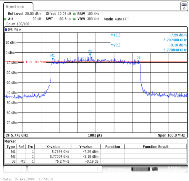
11AX80MIMO-Ant2-5775-PASS
