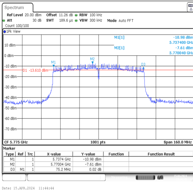
11AC80MIMO-Ant1-5775-PASS
