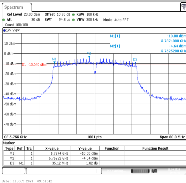
11AC40MIMO-Ant1-5755-PASS
