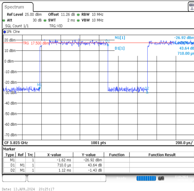
NTNV-11A-Ant1-5825
