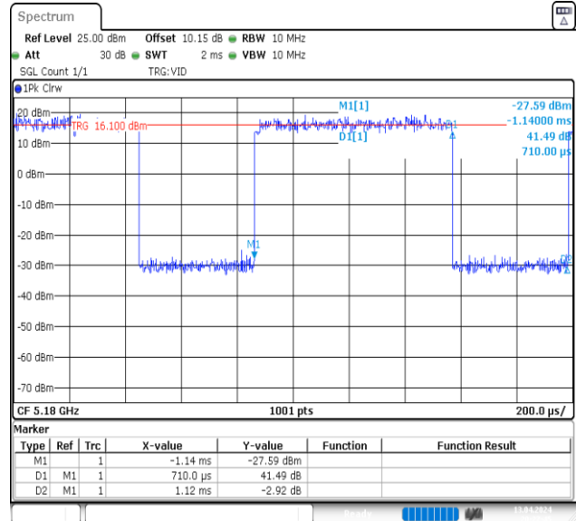
NTNV-11A-Ant2-5180
