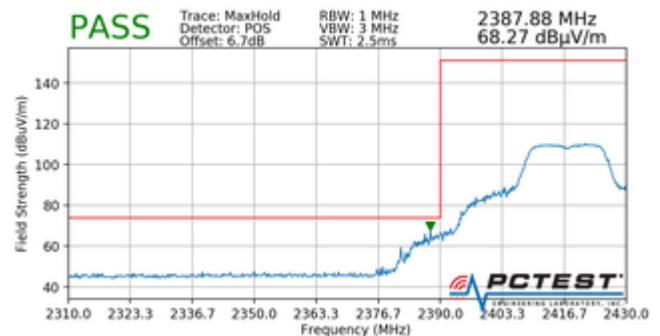
Plot 7-38. Radiated Restricted Lower Band Edge Measurement (Peak)
