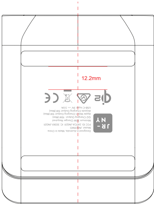
BASE VIEW
