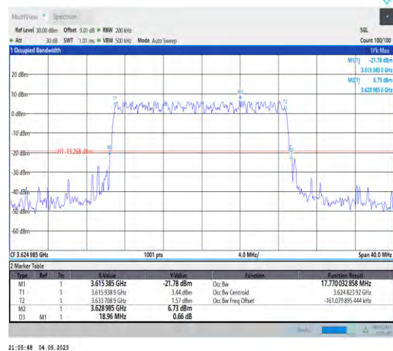
1-N48-PC3-30-20-M-5-DFT-256QAM-Outer_Full-50 @0-Ant1-17.77-18.960-≤20-PASS
