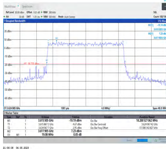
1-N48-PC3-30-20-M-7-CP-16QAM-Outer_Full-51@0- Ant1-18.201-19.080-≤20-PASS
