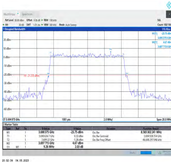
1-N48-PC3-30-10-H-9-CP-256QAM-Outet_Full-24@0 0-Ant1-8.583-9.260-≤10-PASS
