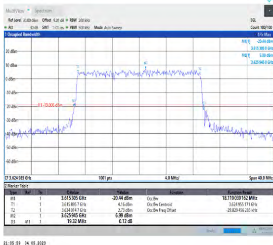
1-N48-PC3-30-20-M-6-CP-QPSK-Outer_Full-51@0- Ant1-18.119-19.320-≤20-PASS
