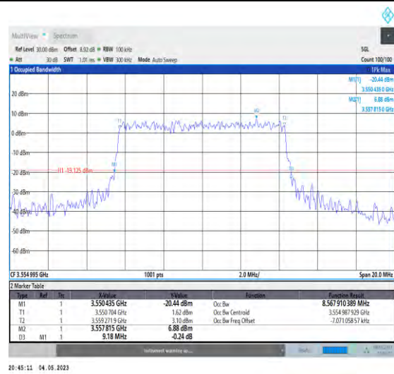
1-N48-PC3-30-10-L-6-CP-QPSK-Outer_Full-24@0- Ant1-8.568-9.180-≤10-PASS
