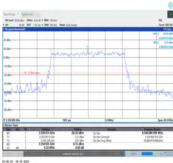
1-N48-PC3-30-10-L-7-CP-16QAM-Outer_Full-24@0- Ant1-8.546-9.240-≤10-PASS
