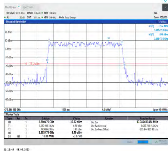
1-N48-PC3-30-20-H-4-DFT-64QAM-Outer_Full-50@0-Ant1-17.746-18.880-≤20-PASS
