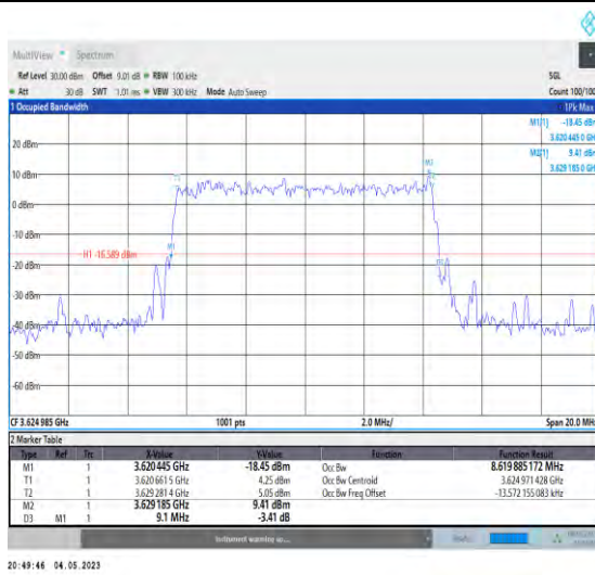
1-N48-PC3-30-10-M-4-DFT-64QAM-Outer_Full-24@ 0-Ant1-8.62-9.100-≤10-PASS
