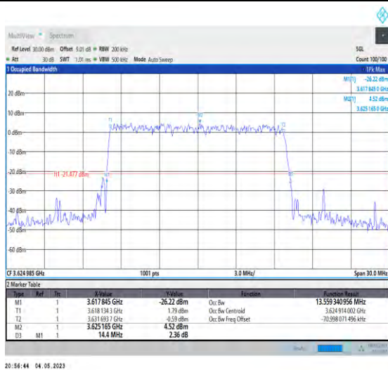
1-N48-PC3-30-15-M-9-CP-256QAM-Outer_Full-38@ 0-Ant1-13.559-14.400-≤15-PASS
