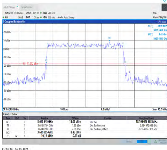
1-N48-PC3-30-20-M-8-CP-64QAM-Outer_Full-51@0- Ant1-18.195-19.120-≤20-PASS
