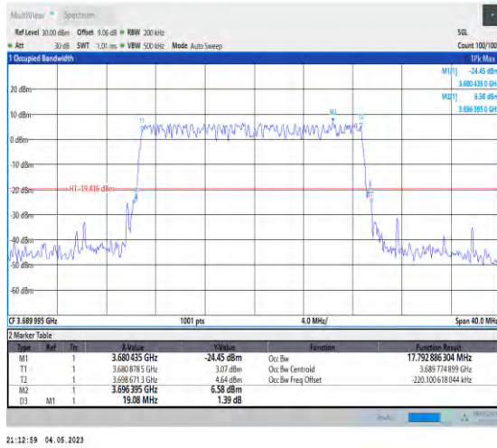
1-N48-PC3-30-20-H-5-DFT-256QAM-Outer_Full-50 @0-Ant1-17.793-19.080-≤20-PASS
