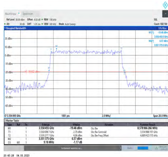
1-N48-PC3-30-10-L-8-CP-64QAM-Outer_Full-24@0- Ant1-8.579-9.180-≤10-PASS
