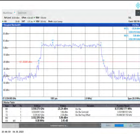
1-N48-PC3-30-10-L-5-DFT-256QAM-Outer_Full-24 @0-Ant1-8.573-9.380-≤10-PASS
