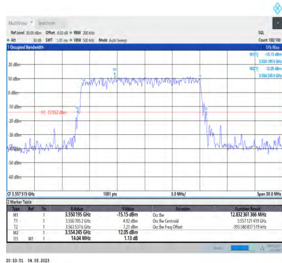
1-N48-PC3-30-15-L-1-DFT-QPSK-Outet_Full-36@0- Ant1-12.832-14.040-≤15-PASS
