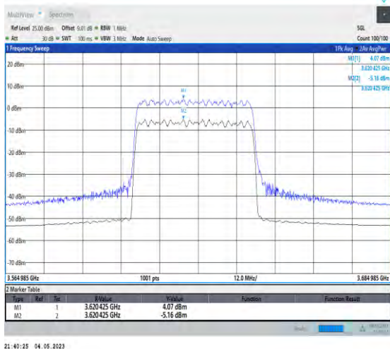
1-N48-PC3-30-40-M-1-DFT-256QAM-Outer_Full-100 @0-Ant1-9.23-100%-0.00-9.23-PASS-≤13
