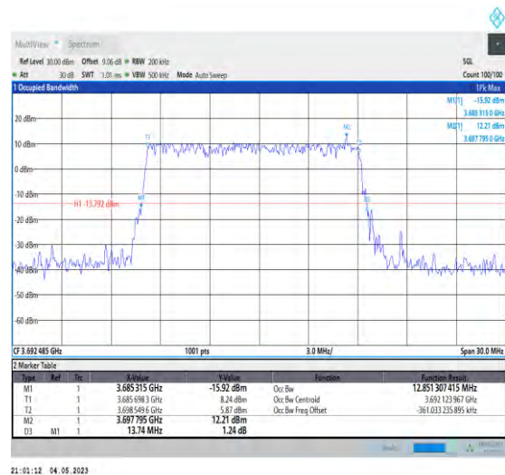
1-N48-PC3-30-15-H-3-DFT-16QAM-Outer_Full-36@ 0-Ant1-12.851-13.740-≤15-PASS
