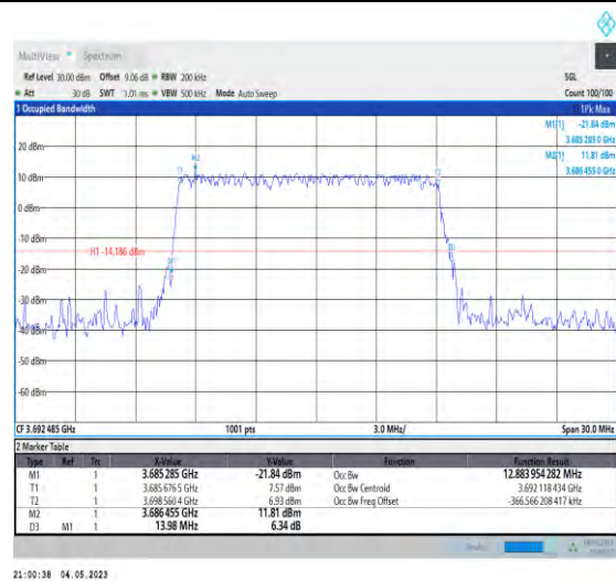
1-N48-PC3-30-15-H-1-DFT-QPSK-Outer_Full-36@0 -Ant1-12.884-13.980-≤15-PASS
