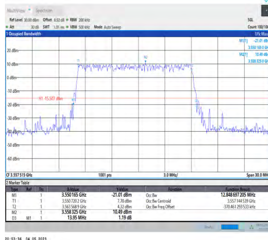
1-N48-PC3-30-15-L-3-DFT-16QAM-Outer_Full-36@ 0-Ant1-12.849-13.950-≤15-PASS
