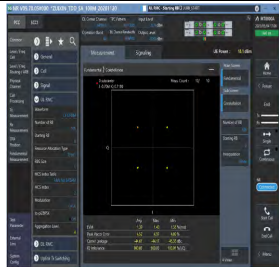
1-N48-PC3-30-40-M-6-CP-QPSK-Outer_Full-106@ 0-Ant1-see graph-PASS
