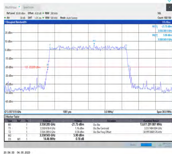
1-N48-PC3-30-15-L-9-CP-256QAM-Outer_Full-38@0- 0-Ant1-13.611-14.460-≤15-PASS
