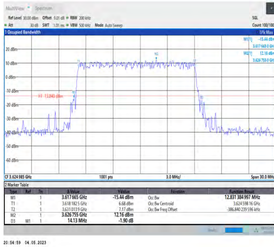
1-N48-PC3-30-15-M-1-DFT-QPSK-Outer_Full-36@0 -Ant1-12.831-14.130-≤15-PASS
