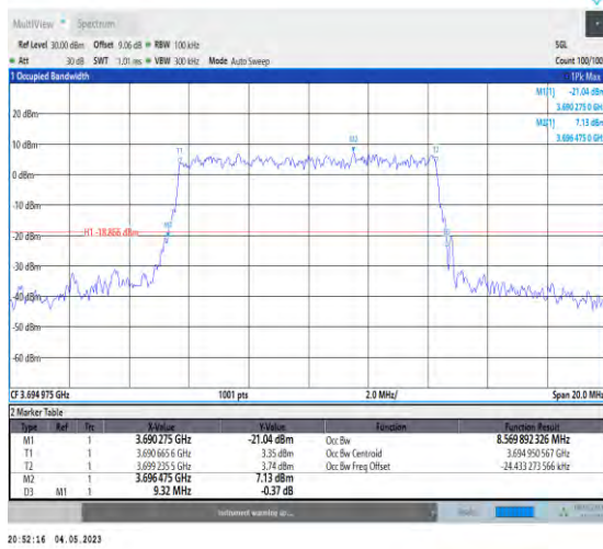
1-N48-PC3-30-10-H-7-CP-16QAM-Outet_Full-24@0 -Ant1-8.57-9.320-≤10-PASS
