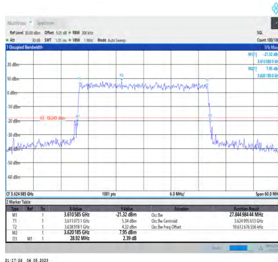
1-N48-PC3-30-30-M-6-CP-QPSK-Outer_Full-78@0- Ant1-27.845-28.920-≤30-PASS
