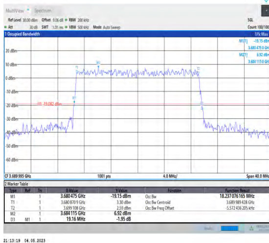
1-N48-PC3-30-20-H-7-CP-16QAM-Outer_Full-51@0 -Ant1-18.237-19.160-≤20-PASS
