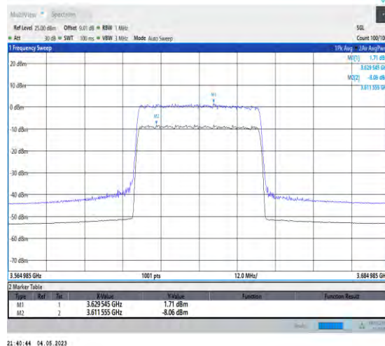
1-N48-PC3-30-40-M-2-CP-256QAM-Outer_Full-106 @0-Ant1-9.77-100%-0.00-9.77-PASS-≤13
