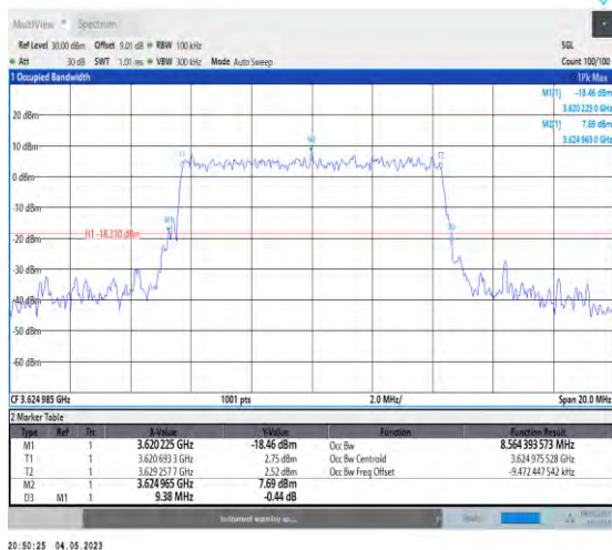
1-N48-PC3-30-10-M-8-CP-64QAM-Outter_Full-24@0 -Ant1-8.564-9.380-≤10-PASS
