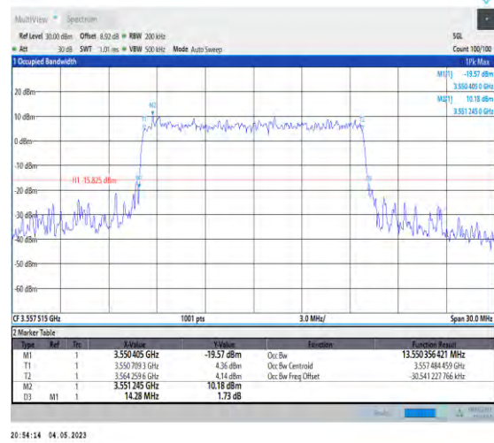
1-N48-PC3-30-15-L-7-CP-16QAM-Outer_Full-38@0- Ant1-13.55-14.280-≤15-PASS
