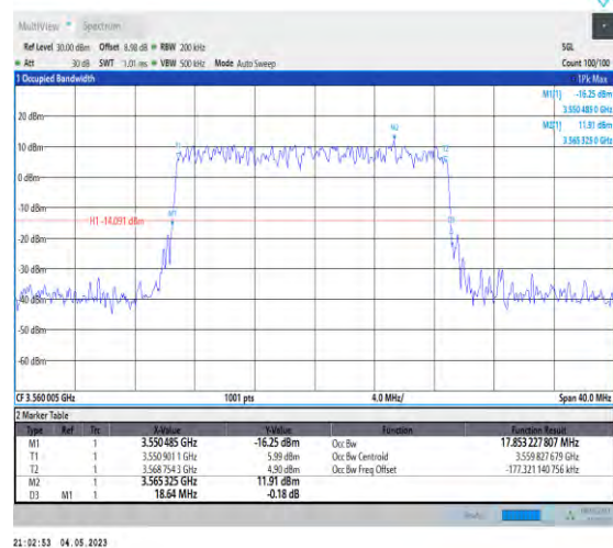
1-N48-PC3-30-20-L-2-DFT-PI2BPSK-Outter_Full-50@0-Ant1-17.853-18.640-≤20-PASS
