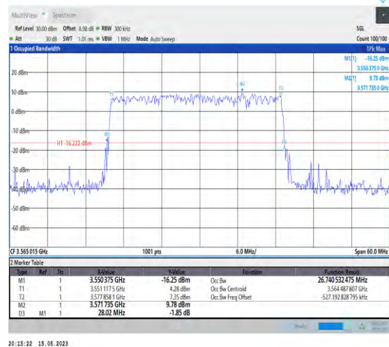
1-N48-PC3-30-30-L-3-DFT-16QAM-Outer_Full-75@ 0-Ant1-26.740-28.020-≤30-PASS
