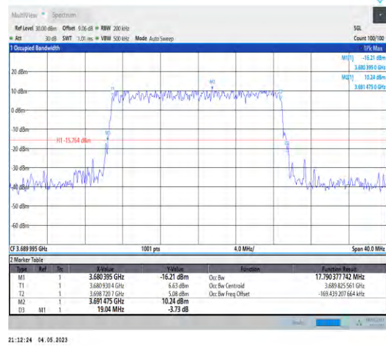
1-N48-PC3-30-20-H-2-DFT-PI2BPSK-Outer_Full-50@0-Ant1-17.79-19.040-≤20-PASS
