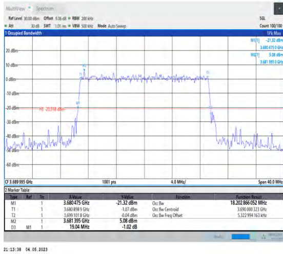
1-N48-PC3-30-20-H-9-CP-256QAM-Outer_Full-51@ 0-Ant1-18.203-19.040-≤20-PASS
