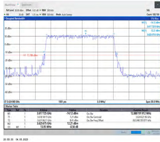
1-N48-PC3-30-15-M-2-DFT-PI2BPSK-Outer_Full-36 @0-Ant1-12.88-13.950-≤15-PASS
