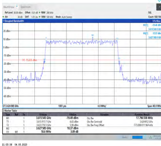
1-N48-PC3-30-20-M-4-DFT-64QAM-Outer_Full-50@ 0-Ant1-17.797-18.600-≤20-PASS
