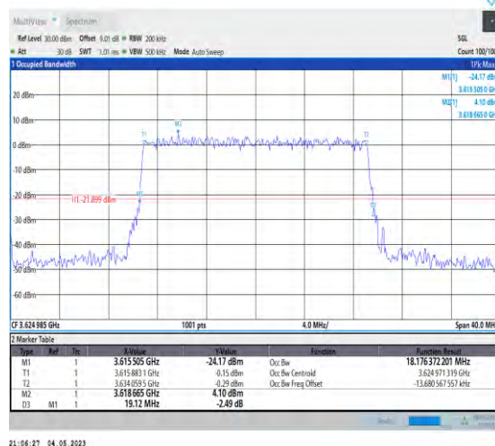
1-N48-PC3-30-20-M-9-CP-256QAM-Outer_Full-51@0- Ant1-18.176-19.120-≤20-PASS
