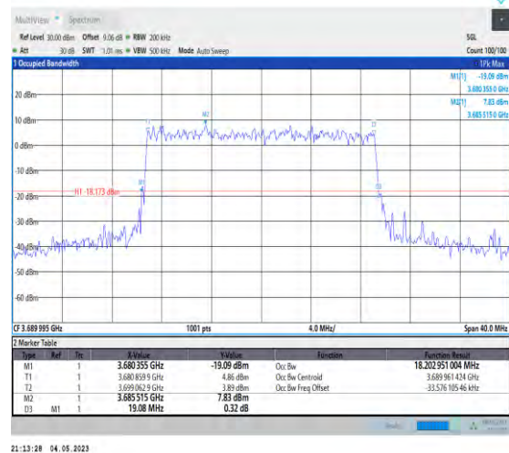
1-N48-PC3-30-20-H-8-CP-64QAM-Outer_Full-51@0 -Ant1-18.203-19.080-≤20-PASS
