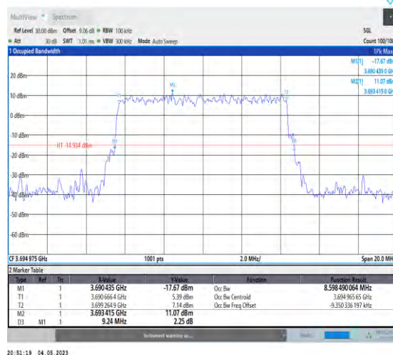
1-N48-PC3-30-10-H-2-DFT-PI2BPSK-Outter_Full-24@0 @0-Ant1-8.598-9.240-≤10-PASS
