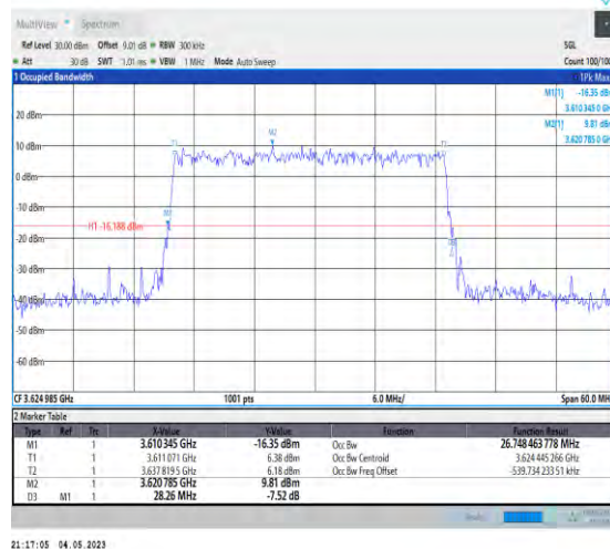
1-N48-PC3-30-30-M-4-DFT-64QAM-Outer_Full-75@ 0-Ant1-26.748-28.260-≤30-PASS
