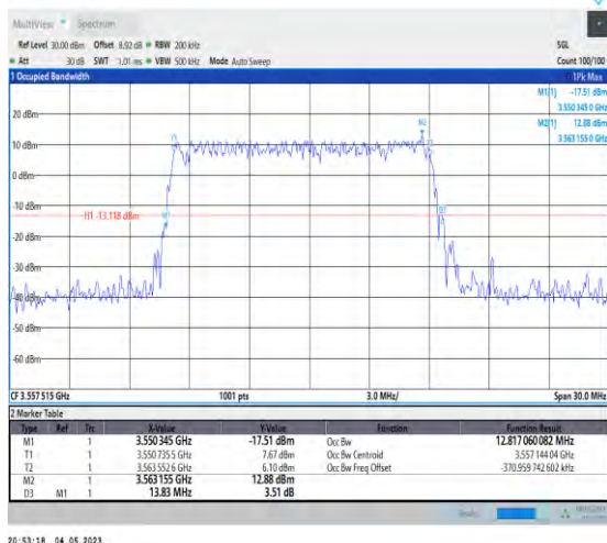
1-N48-PC3-30-15-L-2-DFT-PI2BPSK-Outer_Full-36 @0-Ant1-12.817-13.830-≤15-PASS
