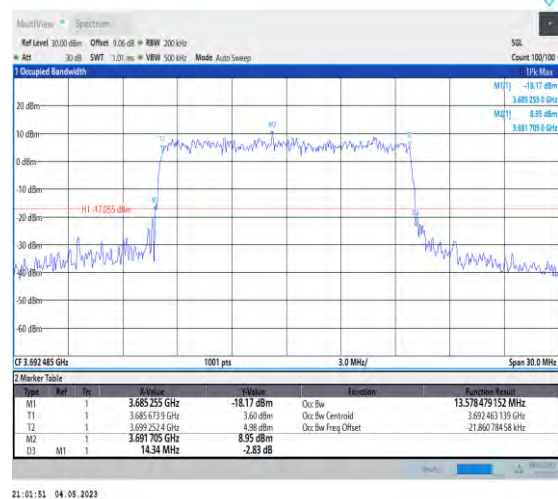
1-N48-PC3-30-15-H-7-CP-16QAM-Outer_Full-38@0- Ant1-13.578-14.340-≤15-PASS
