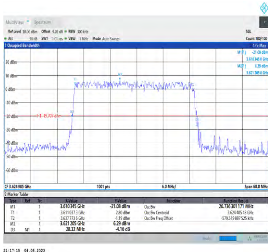
1-N48-PC3-30-30-M-5-DFT-256QAM-Outer_Full-75 @0-Ant1-26.736-28.320-≤30-PASS
