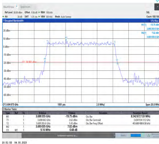
1-N48-PC3-30-10-H-5-DFT-256QAM-Outer_Full-24 @0-Ant1-8.543-9.160-≤10-PASS
