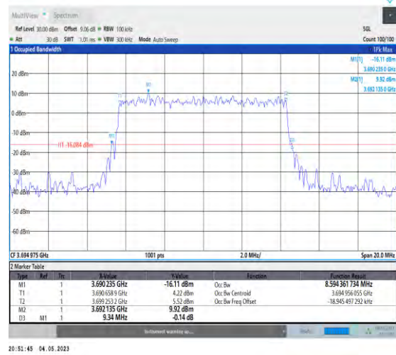
1-N48-PC3-30-10-H-4-DFT-64QAM-Outer_Full-24@ 0-Ant1-8.594-9.340-≤10-PASS
