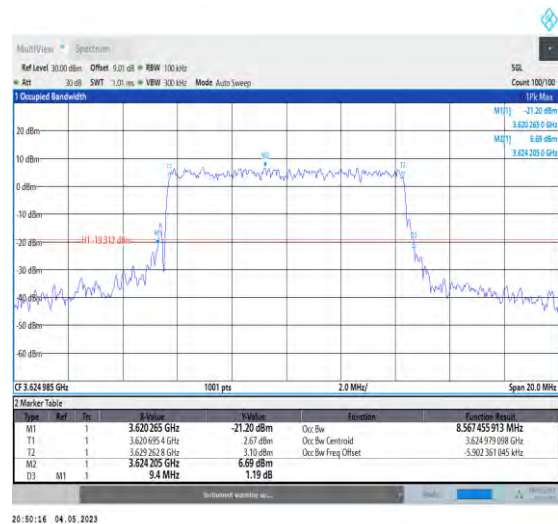
1-N48-PC3-30-10-M-7-CP-16QAM-Outer_Full-24@0- Ant1-8.567-9.400-≤10-PASS
