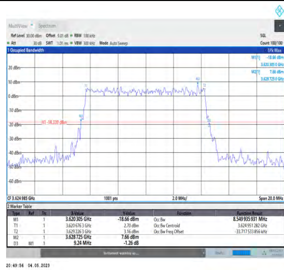
1-N48-PC3-30-10-M-5-DFT-256QAM-Outer_Full-24@ 0-Ant1-8.55-9.240-≤10-PASS
