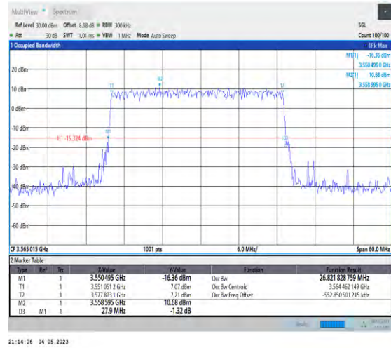
1-N48-PC3-30-30-L-1-DFT-QPSK-Outer_Full-75@0- Ant1-26.822-27.900-≤30-PASS
