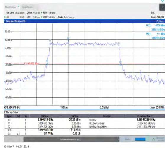
1-N48-PC3-30-10-H-6-CP-QPSK-Outer_Full-24@0- Ant1-8.555-9.100-≤10-PASS
