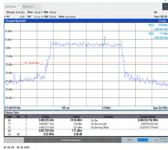
1-N48-PC3-30-10-H-8-CP-64QAM-Outet_Full-24@0 -Ant1-8.585-9.320-≤10-PASS
