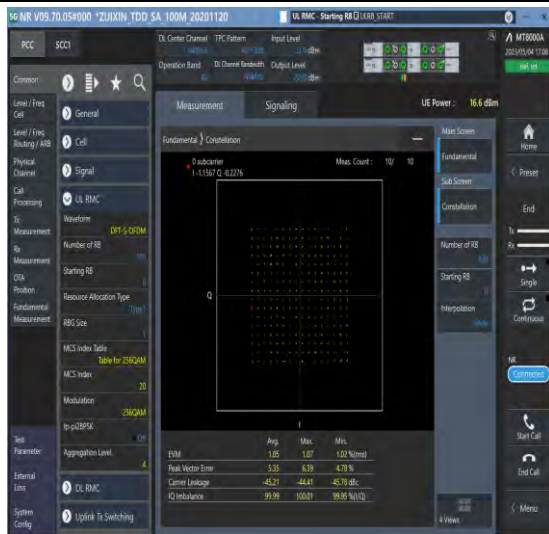
1-N48-PC3-30-40-M-5-DFT-256QAM-Outer_Full-100 @0-Ant1-see graph-PASS
