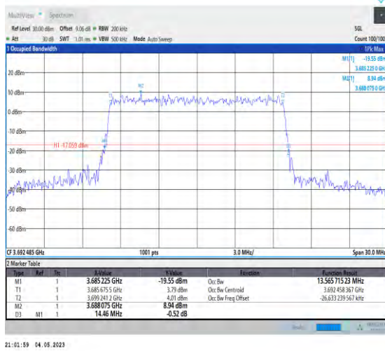
1-N48-PC3-30-15-H-8-CP-64QAM-Outter_Full-38@0 -Ant1-13.566-14.460-≤15-PASS
