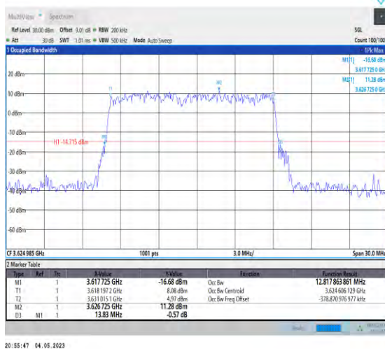
1-N48-PC3-30-15-M-3-DFT-16QAM-Outer_Full-36@ 0-Ant1-12.818-13.830-≤15-PASS
