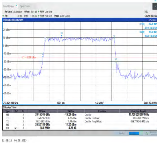
1-N48-PC3-30-20-M-2-DFT-PI2BPSK-Outer_Full-50 @0-Ant1-17.729-18.800-≤20-PASS
