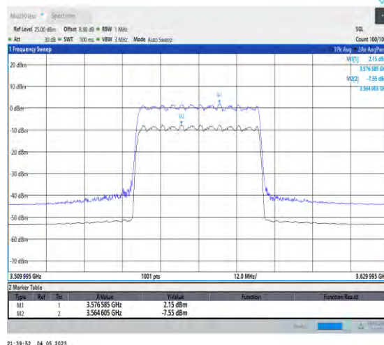
1-N48-PC3-30-40-L-2-CP-256QAM-Outer_Full-106 @0-Ant1-9.70-100%-0.00-9.70-PASS-≤13
