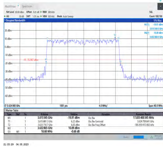
1-N48-PC3-30-20-M-3-DFT-16QAM-Outer_Full-50@ 0-Ant1-17.835-18.680-≤20-PASS
