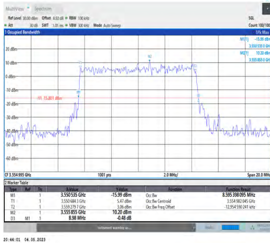
1-N48-PC3-30-10-L-1-DFT-QPSK-Outer_Full-24@0-Ant1-8.595-8.980-≤10-PASS
