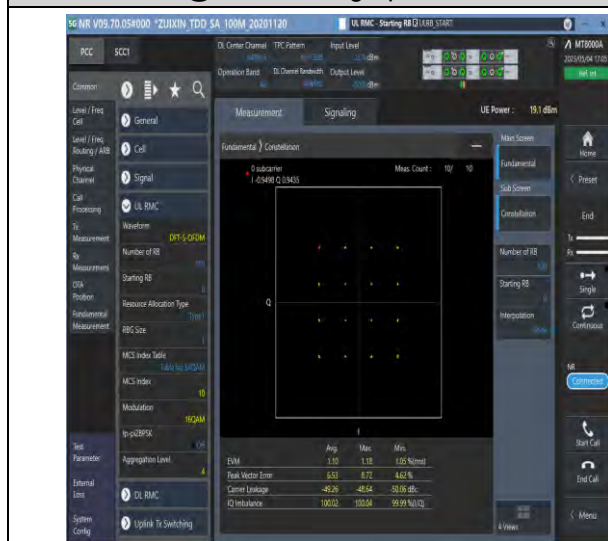
1-N48-PC3-30-40-M-3-DFT-16QAM-Outter_Full-100 @0-Ant1-see graph-PASS
