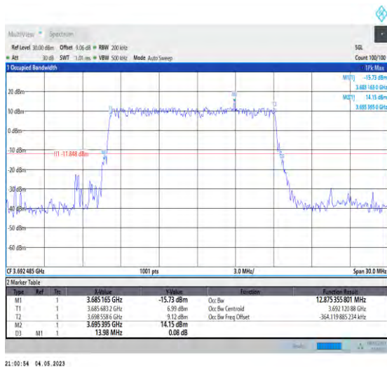
1-N48-PC3-30-15-H-2-DFT-PI2BPSK-Outer_Full-36 @0-Ant1-12.875-13.980-≤15-PASS
