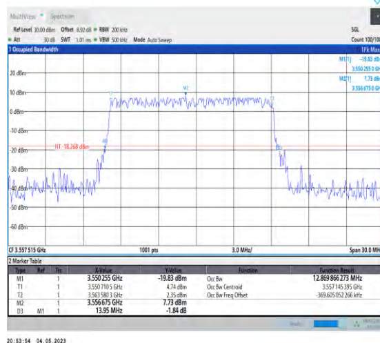
1-N48-PC3-30-15-L-5-DFT-256QAM-Outer_Full-36 @0-Ant1-12.87-13.950-≤15-PASS
