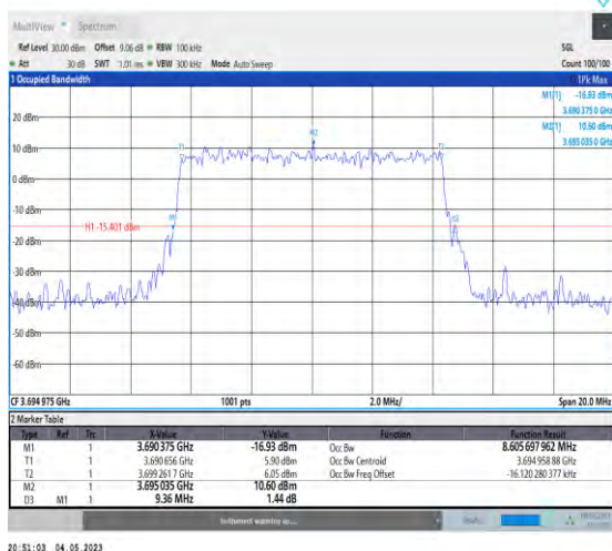
1-N48-PC3-30-10-H-1-DFT-QPSK-Outter_Full-24@0- Ant1-8.606-9.360-≤10-PASS
