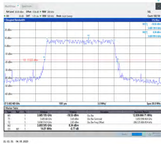
1-N48-PC3-30-15-H-5-DFT-256QAM-Outer_Full-36@ 0-Ant1-12.837-14.010-≤15-PASS
