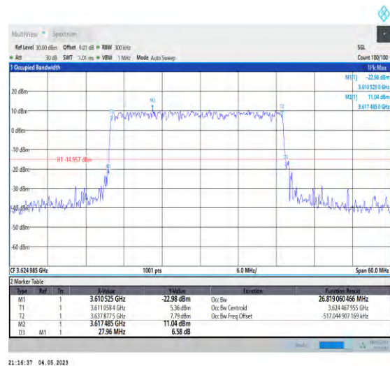
1-N48-PC3-30-30-M-2-DFT-PI2BPSK-Outer_Full-75@0-Ant1-26.819-27.960-≤30-PASS
