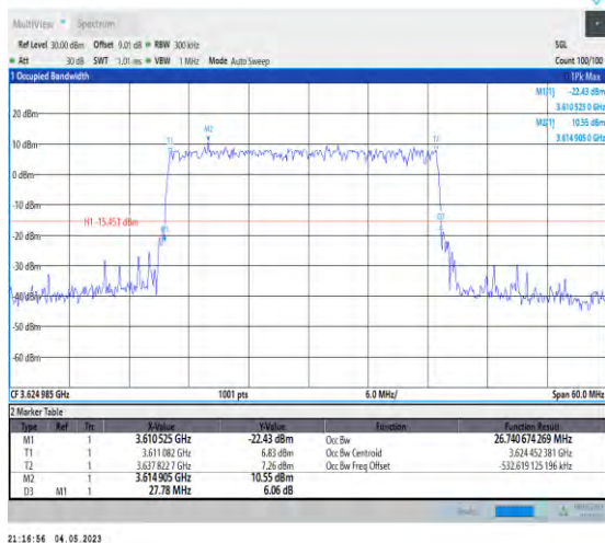
1-N48-PC3-30-30-M-3-DFT-16QAM-Outer_Full-75@ 0-Ant1-26.741-27.780-≤30-PASS
