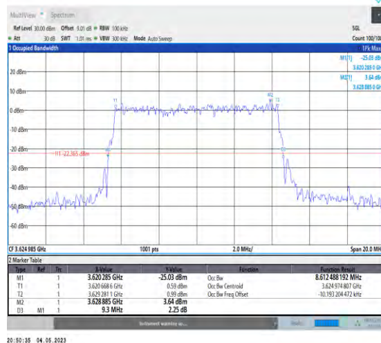
1-N48-PC3-30-10-M-9-CP-256QAM-Outter_Full-24@0 0-Ant1-8.612-9.300-≤10-PASS
