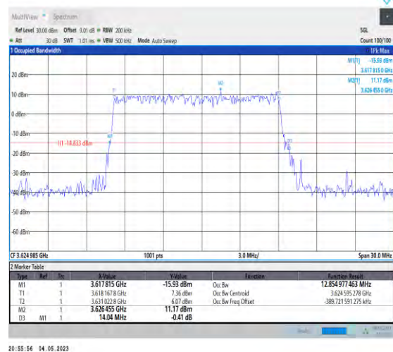
1-N48-PC3-30-15-M-4-DFT-64QAM-Outer_Full-36@ 0-Ant1-12.855-14.040-≤15-PASS
