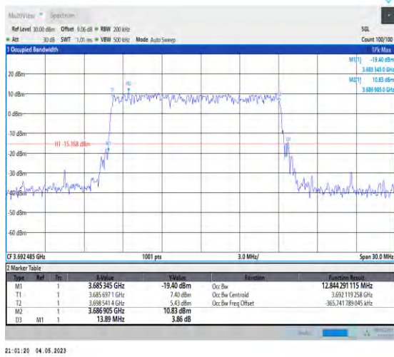
1-N48-PC3-30-15-H-4-DFT-64QAM-Outer_Full-36@ 0-Ant1-12.844-13.890-≤15-PASS
