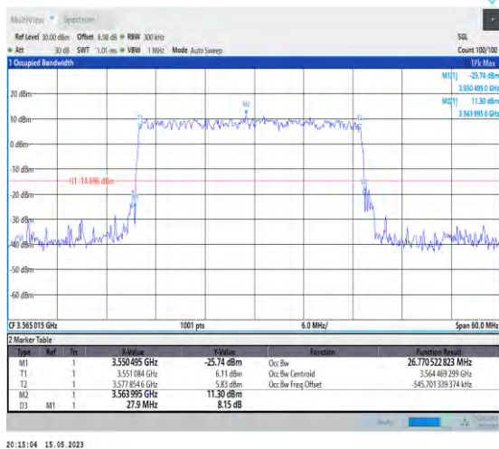
1-N48-PC3-30-30-L-2-DFT-PI2BPSK-Outer_Full-75 @0-Ant1-26.770-27.900-≤30-PASS
