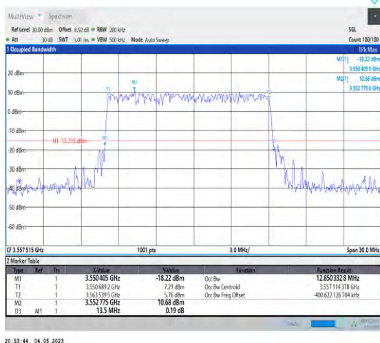
1-N48-PC3-30-15-L-4-DFT-64QAM-Outer_Full-36@ 0-Ant1-12.85-13.500-≤15-PASS
