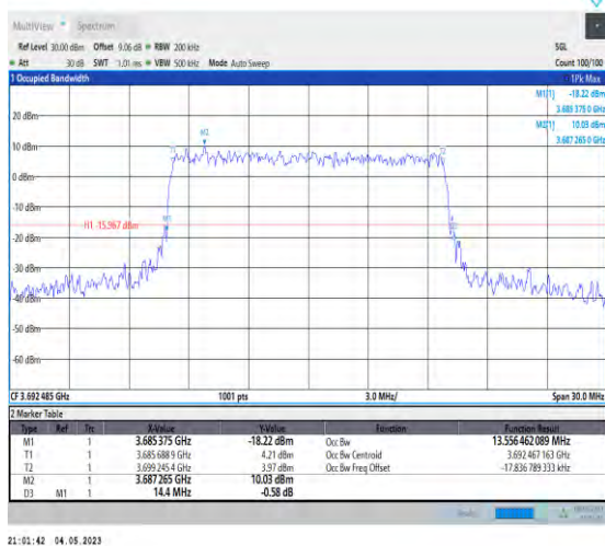
1-N48-PC3-30-15-H-6-CP-QPSK-Outer_Full-38@0- Ant1-13.556-14.400-≤15-PASS
