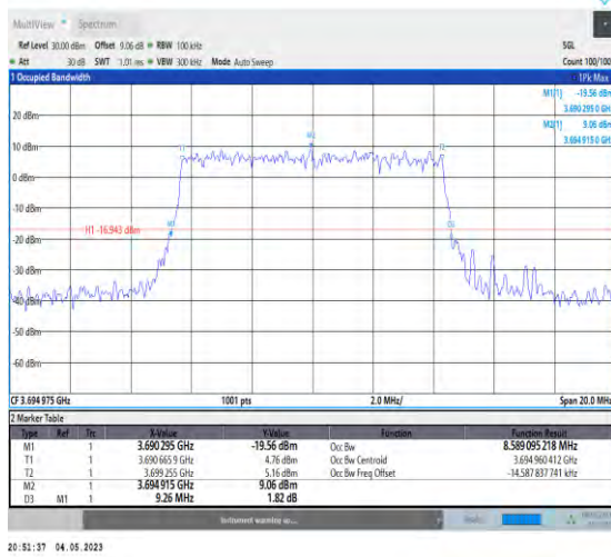
1-N48-PC3-30-10-H-3-DFT-16QAM-Outer_Full-24@ 0-Ant1-8.589-9.260-≤10-PASS
