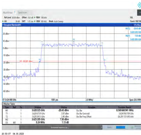
1-N48-PC3-30-10-M-6-CP-QPSK-Outer_Full-24@0- Ant1-8.57-9.240-≤10-PASS
