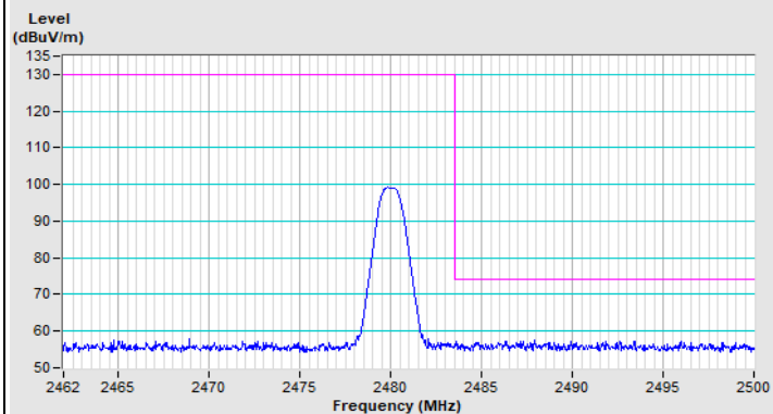
BT GFSK Channel 78
