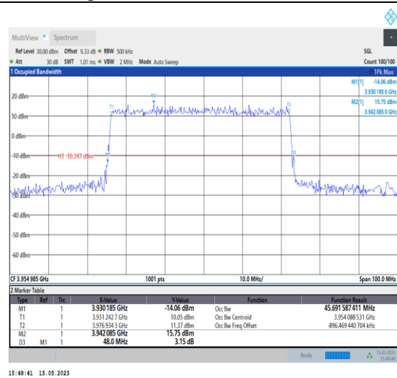
1-N77-3700-3980-PC1-30-50-H-1-DFT-QPSK-Outer_Full-128@0-Ant0-45.692-48.000-≤50-PASS
