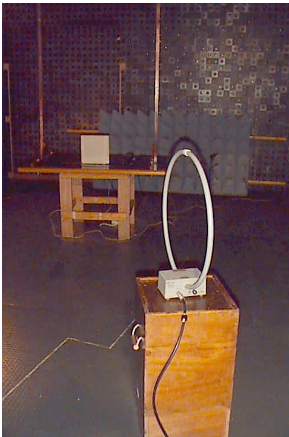
Photograph No.2 Radiated emissions measurement setup in the anechoic chamber with loop antenna
