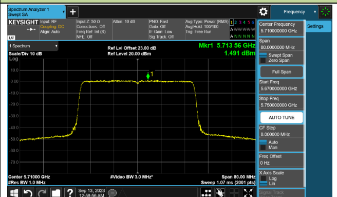
Channel 14 (5710MHz)
