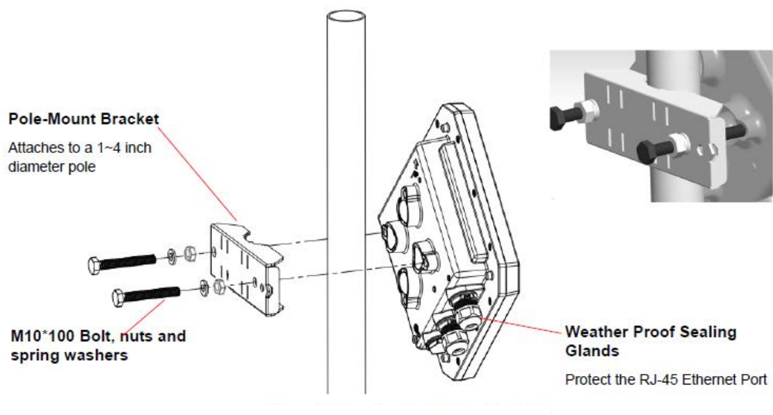
Figure 1: Mounting the ODU on the Pole
