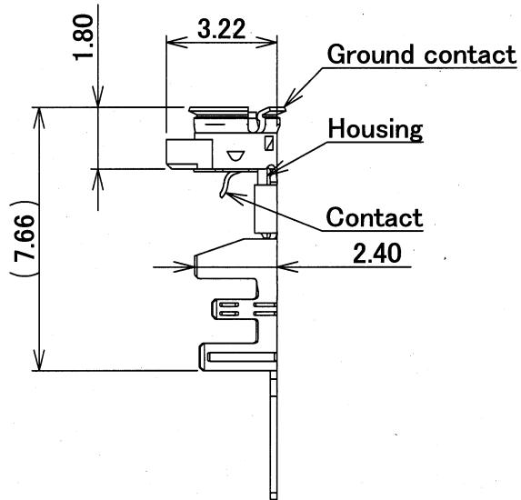
Part No. 20670-001R-18 For semi auto termination machine
