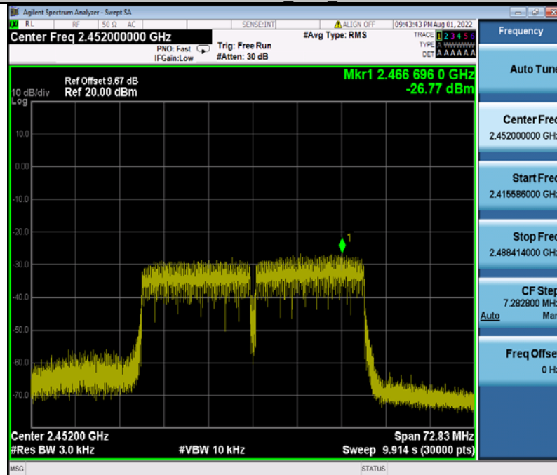
11N40SISO_Ant1_2452
