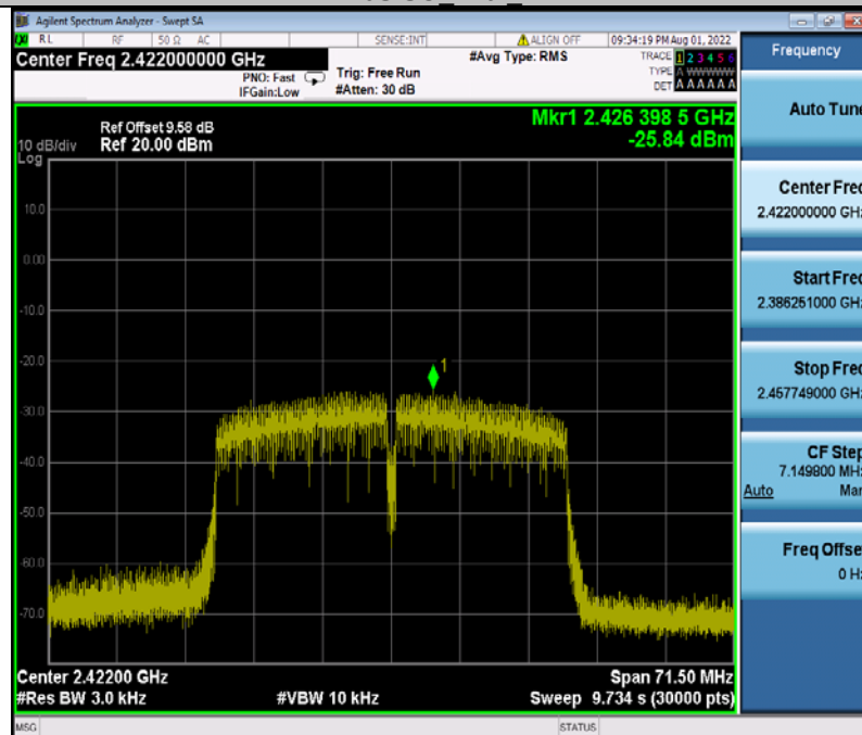
11N40SISO_Ant1_2422
