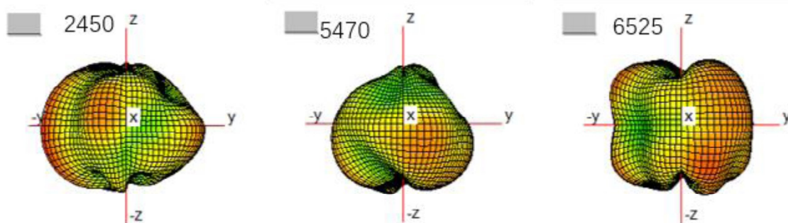
Main Antenna-2
