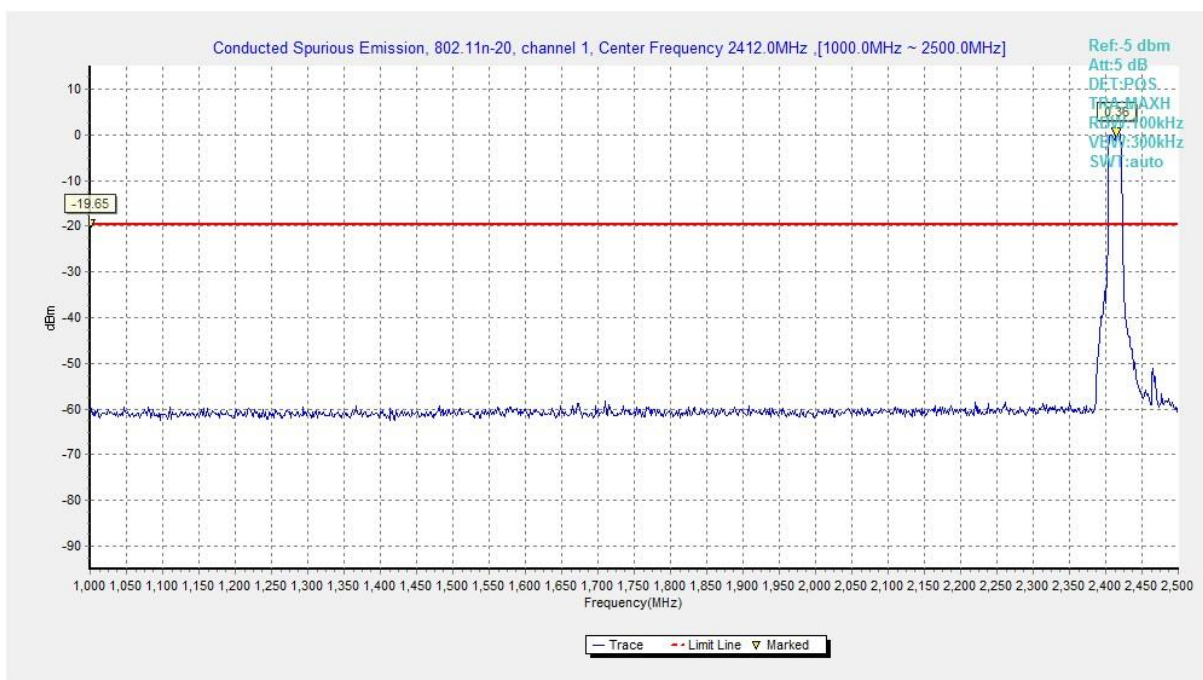
Fig.A.6.1.83 Transmitter Spurious Emission - Conducted (802.11n-HT20, Ch1, 1 GHz-2.5 GHz)
