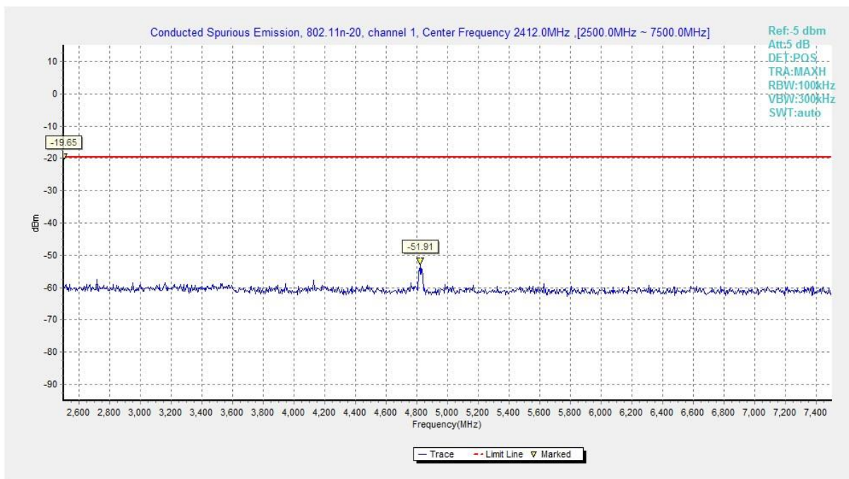
Fig.A.6.1.84 Transmitter Spurious Emission - Conducted (802.11n-HT20, Ch1, 2.5 GHz-7.5 GHz)
