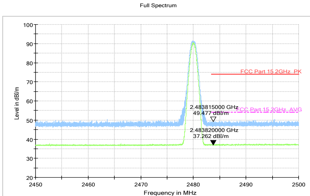
Fig.59. Radiated emission (Power) GFSK, high channel
