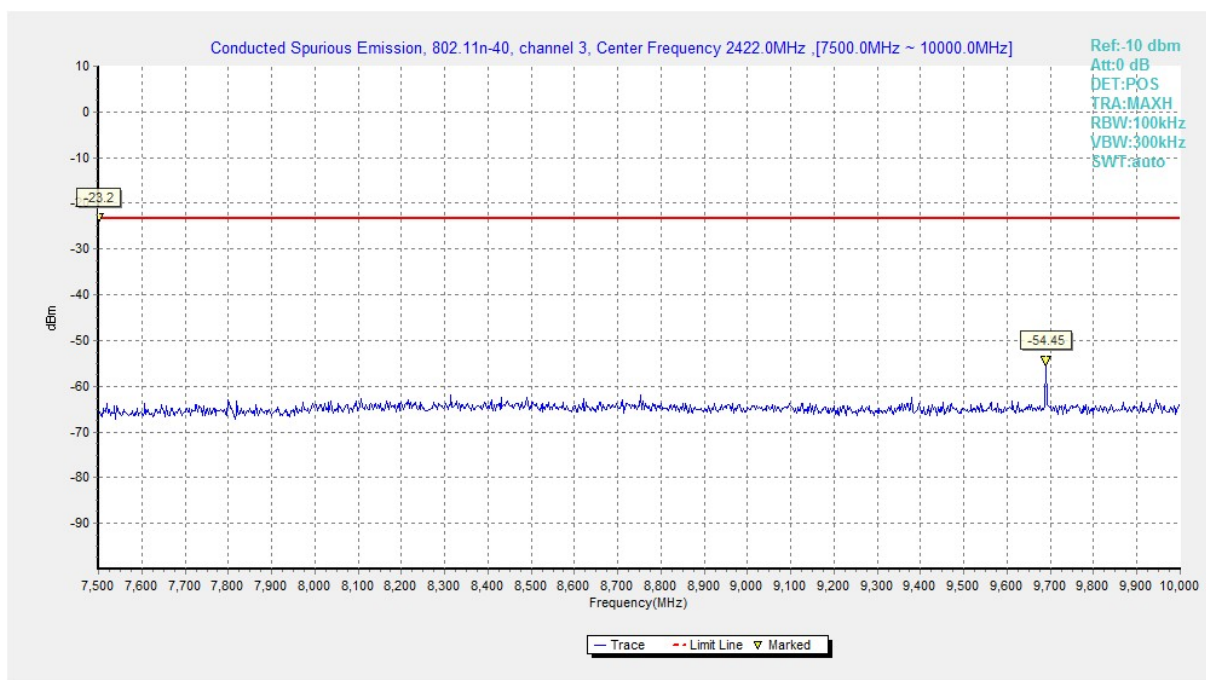
Fig.A.6.1.77 Conducted Spurious Emission (802.11n-HT40, Ch3, 7.5 GHz-10 GHz)
