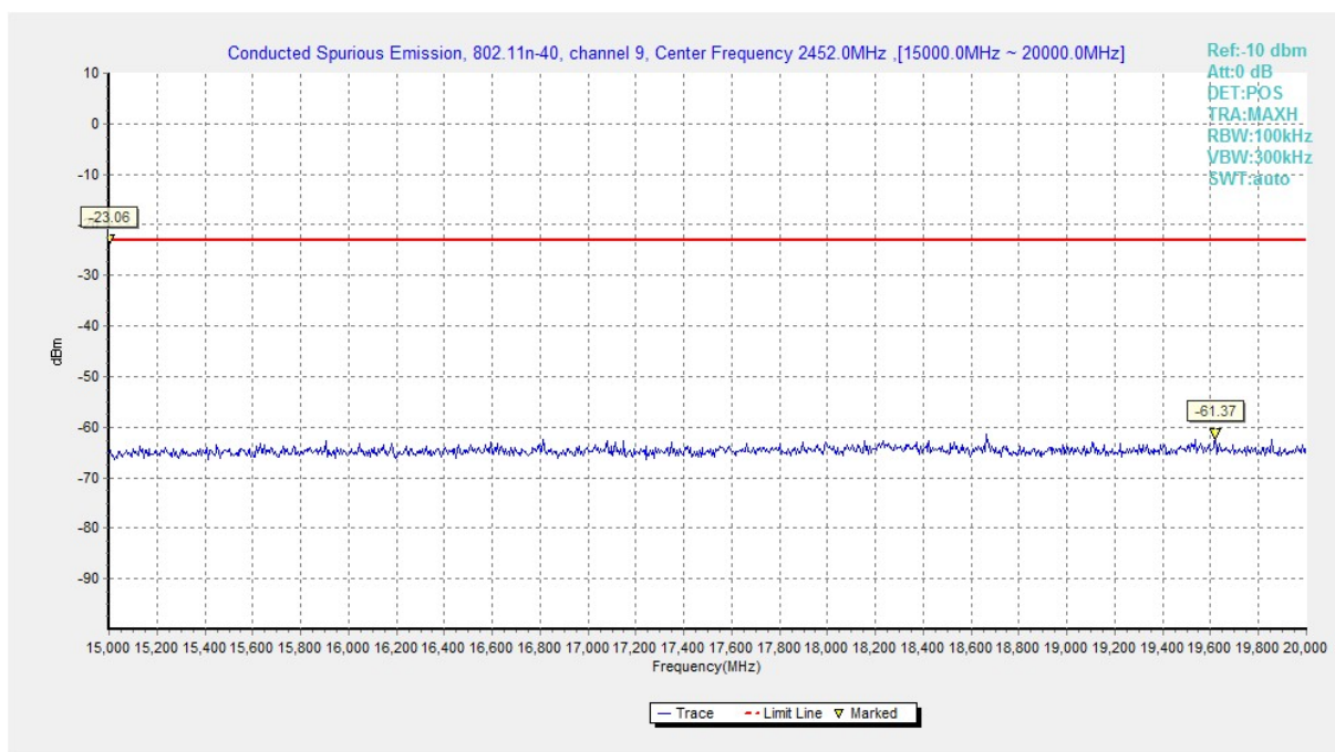
Fig.A.6.1.95 Conducted Spurious Emission (802.11n-HT40, Ch9, 15 GHz-20 GHz)
