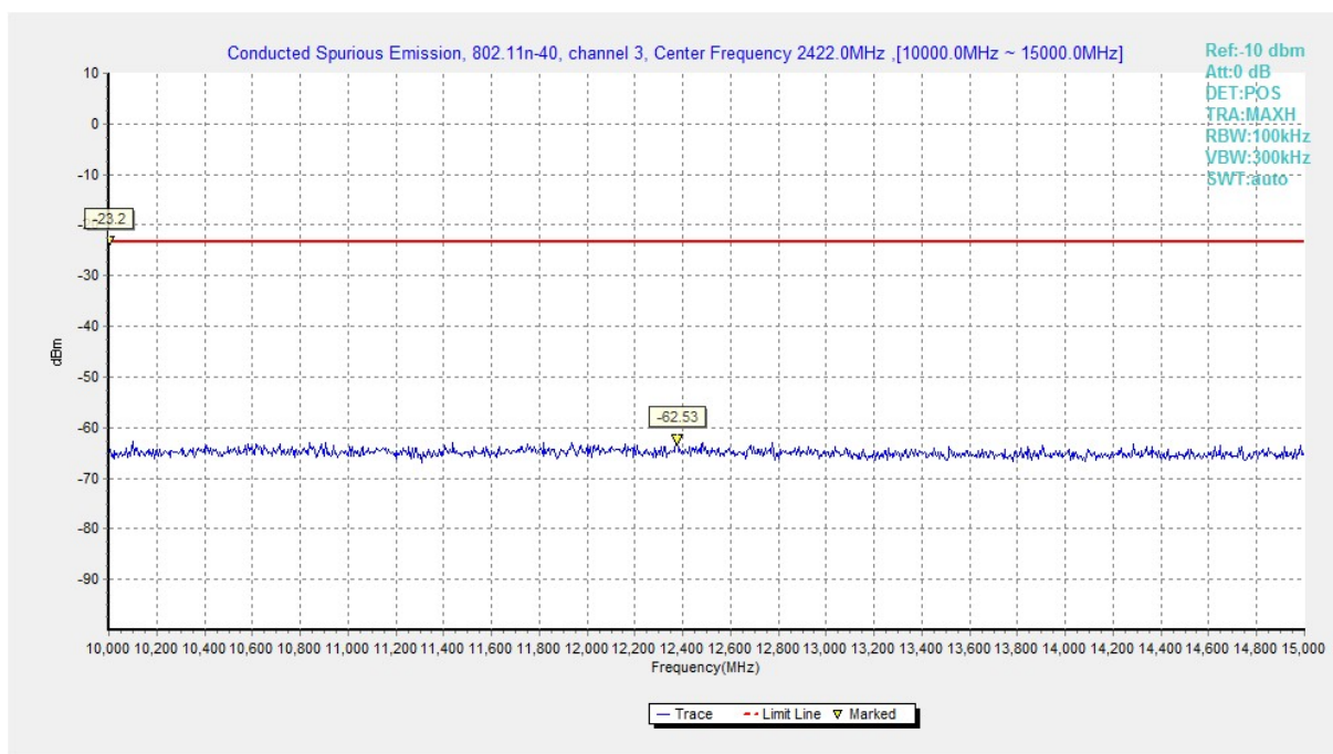
Fig.A.6.1.78 Conducted Spurious Emission (802.11n-HT40, Ch3, 10 GHz-15 GHz)
