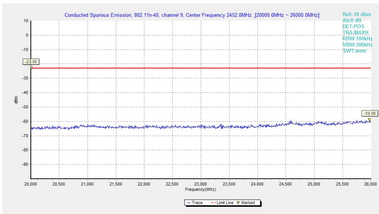
Fig.A.6.1.96 Conducted Spurious Emission (802.11n-HT40, Ch9, 20 GHz-26 GHz)
