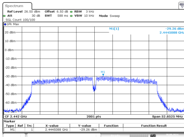
802.11n40_2442MHz_Chain 1 -29.26dBm/3kHz
