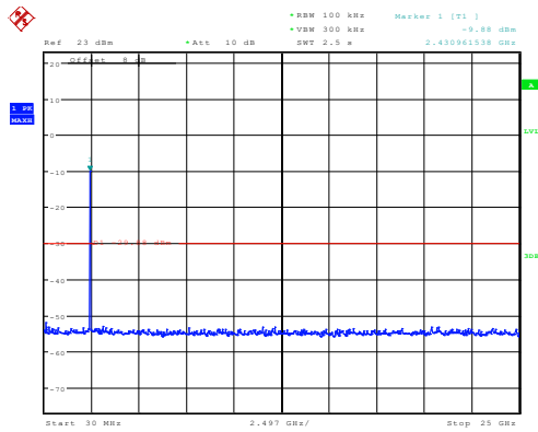
802.11g_2442MHz_Chain 1
