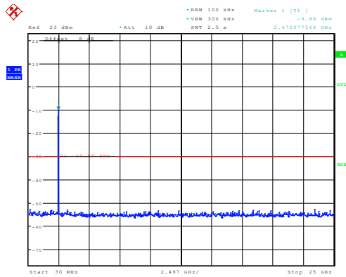
802.11g_2472MHz_Chain 0
