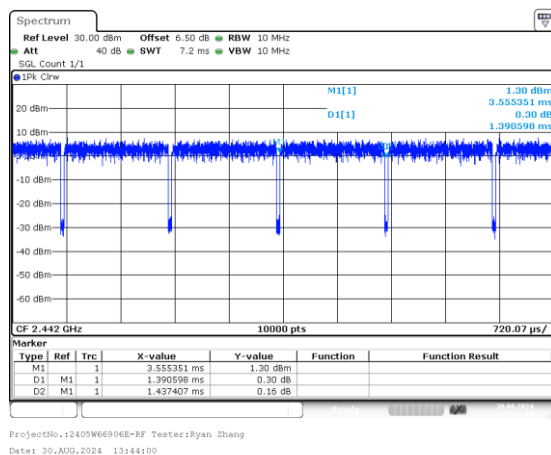
802.11g_2442MHz_Chain 1 1.391ms,1.437ms
