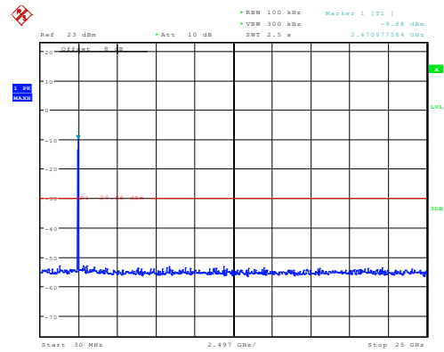
802.11n20_2472MHz_Chain 1
