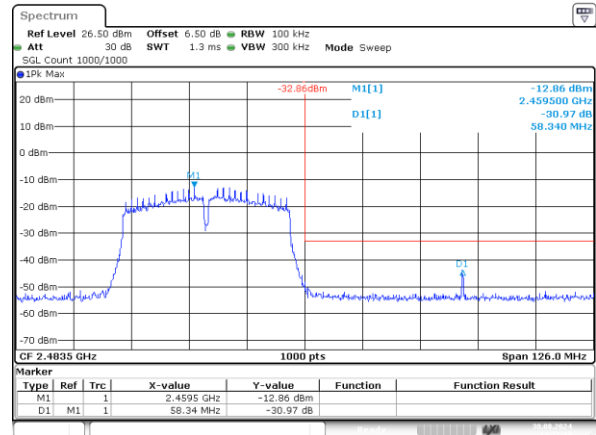
802.11n40_2462MHz_Chain 0
