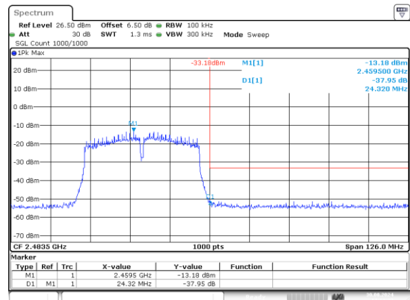
802.11n40_2462MHz_Chain 1
