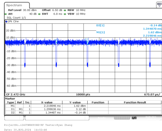
802.11n20_2472MHz_Chain 1 1.300ms,1.345ms
