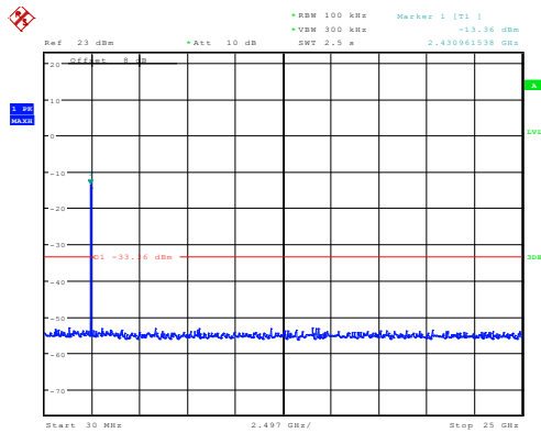
802.11n40_2462MHz_Chain 0
