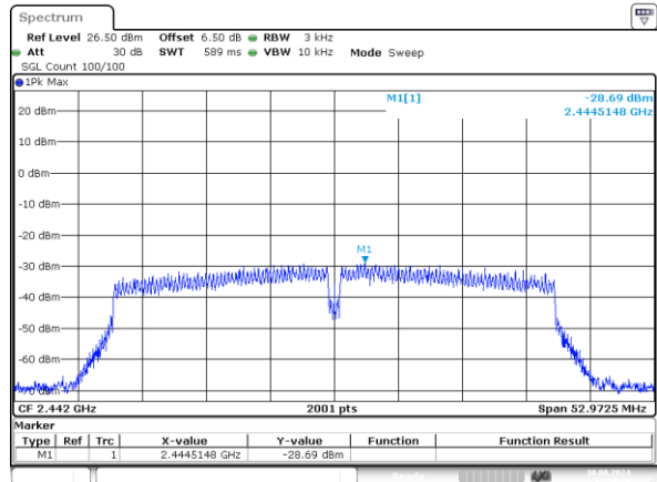
802.11n40_2442MHz_Chain 0 -28.69dBm/3kHz
