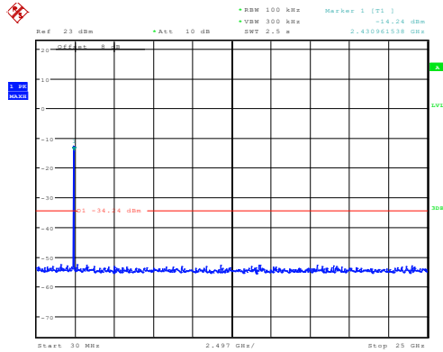
802.11n40_2422MHz_Chain 0
