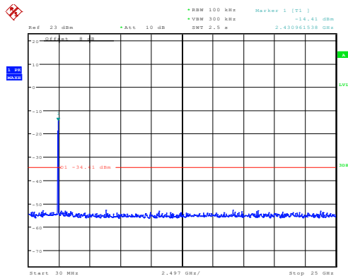
802.11n40_2442MHz_Chain 1
