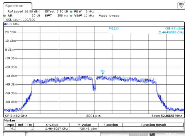
802.11n40_2462MHz_Chain 1 -28.45dBm/3kHz
