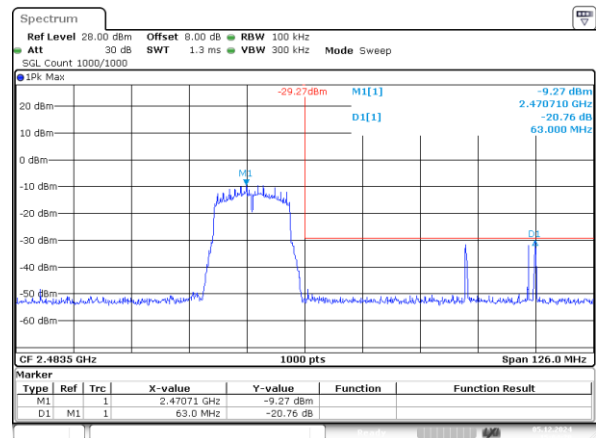
802.11g_2472MHz_Chain 1
