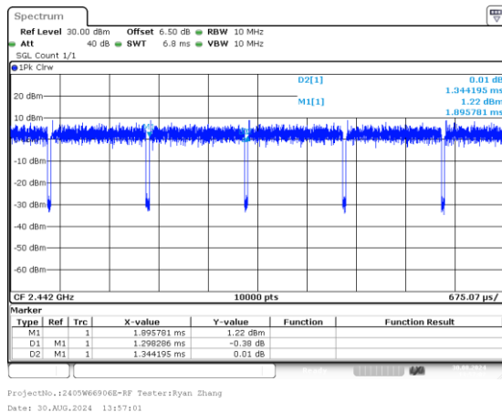
802.11n20_2442MHz_Chain 1 1.298ms,1.344ms
