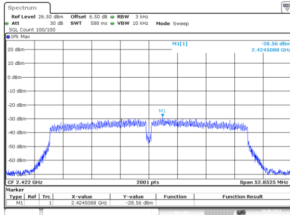
802.11n40_2422MHz_Chain 0 -28.56dBm/3kHz
