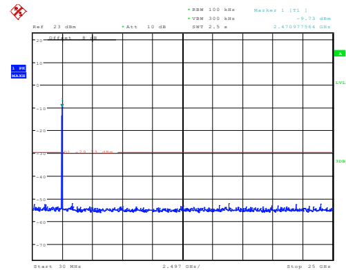
802.11g_2472MHz_Chain 1
