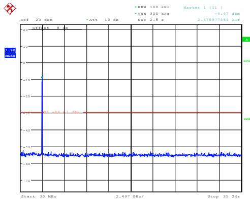
802.11n20_2472MHz_Chain 0
