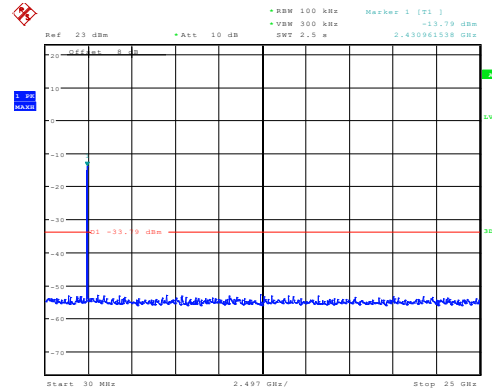
802.11n40_2442MHz_Chain 0
