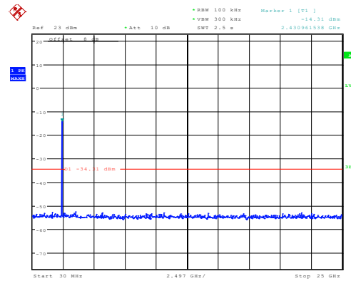
802.11n40_2422MHz_Chain 1
