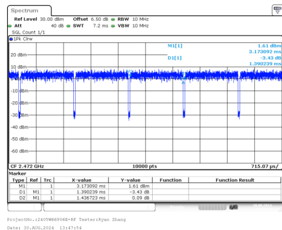
802.11g_2472MHz_Chain 1 1.390ms,1.437ms
