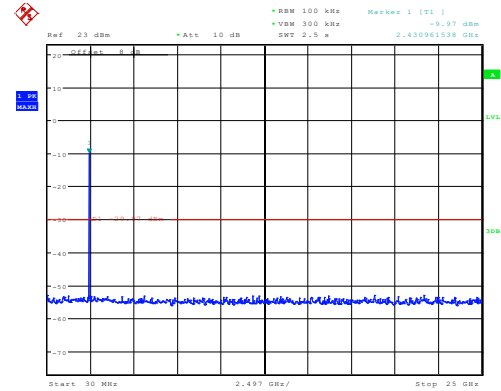
802.11g_2442MHz_Chain 0
