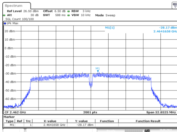
802.11n40_2462MHz_Chain 0 -28.17dBm/3kHz
