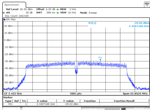
802.11n40_2422MHz_Chain 1 -29.03dBm/3kHz
