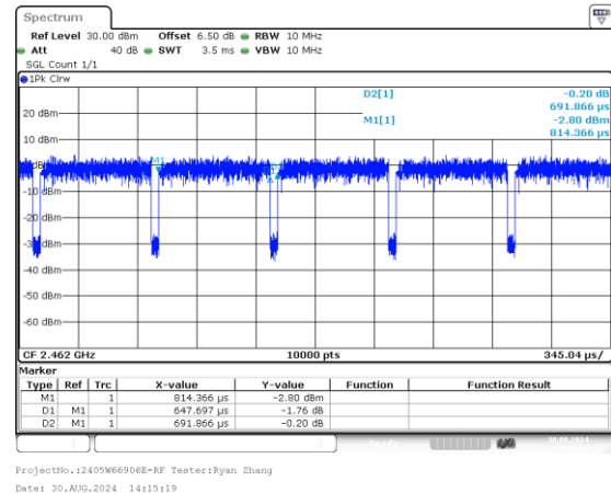
802.11n40_2462MHz_Chain 1 0.648ms,0.692ms
