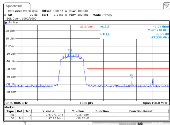
802.11n20_2472MHz_Chain 0
