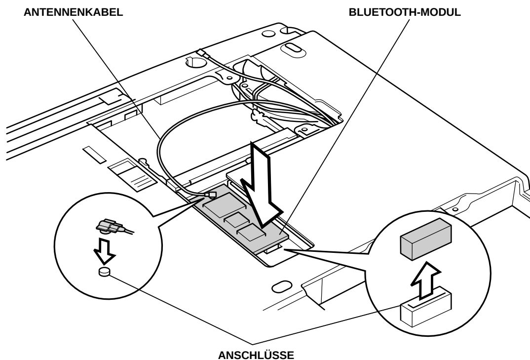
Bluetooth-Modul installieren
