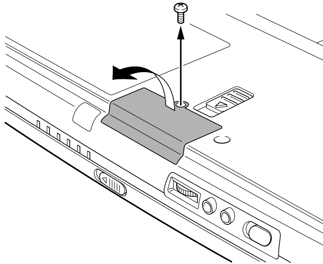
Removing the Bluetooth module slot cover
