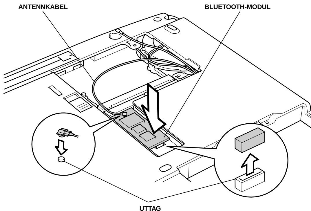
Installera Bluetooth-modulen
