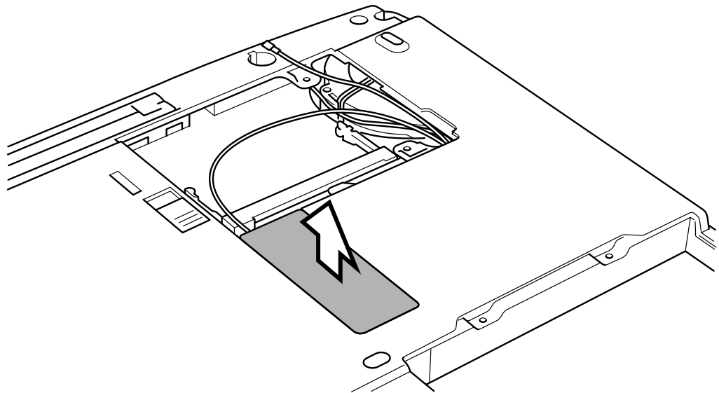
Removing the Bluetooth module slot cover
