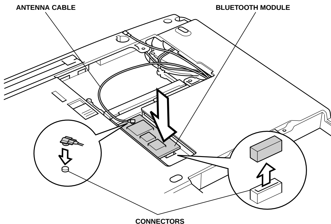
Installing the Bluetooth module
