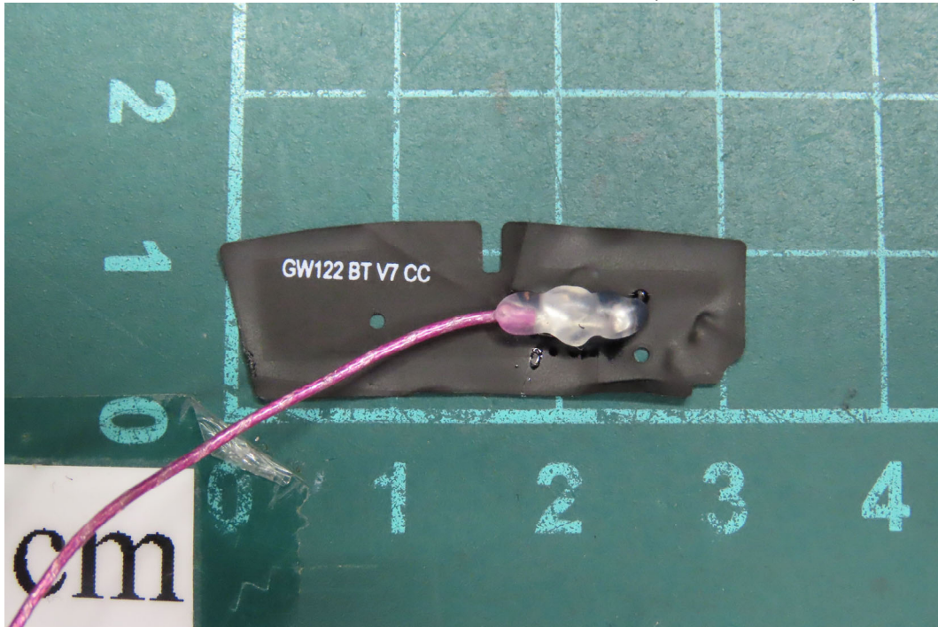
(31) EUT Photo - Brand Name: Cicent, Model No.: 102BK3F1438 (BT/BLE Antenna)
