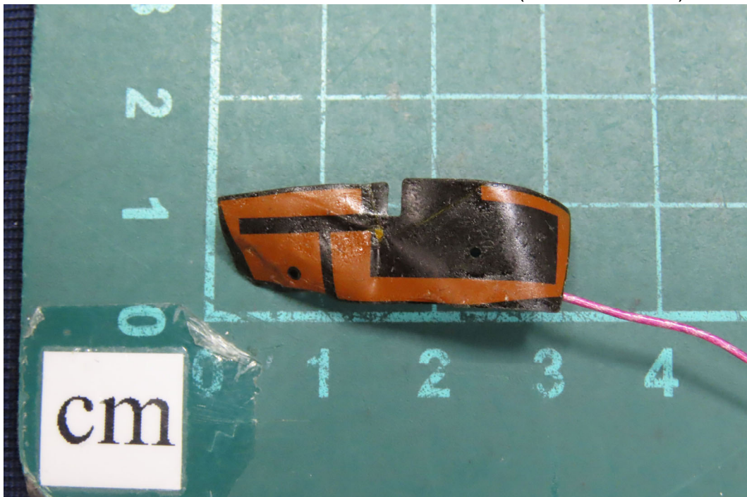
(32) EUT Photo - Brand Name: Cicent, Model No.: 102BK3F1438 (BT/BLE Antenna)
