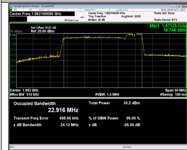
2-2-20MHz-5MHz-64QAM-64QAM-18700-18817-100RB#0-25RB#0-PASS
