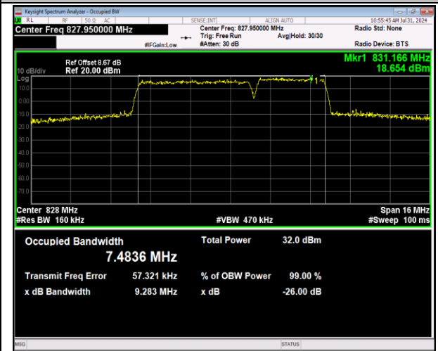
5-5-5MHz-3MHz-64QAM-64QAM-20425-20464-25RB#0-80 -15RB#0-PASS
