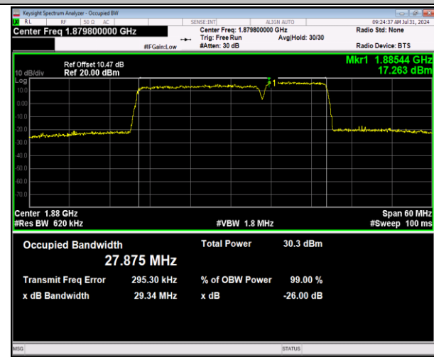
2-2-20MHz-10MHz-64QAM-64QAM-18851-18995-100RB#0-50RB#0-PASS
