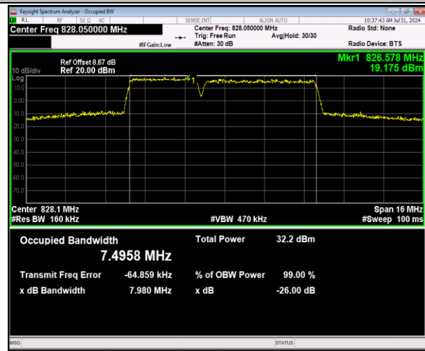
5-5-3MHz-5MHz-64QAM-64QAM-20416-20455-15RB#0-25RB#0-PASS
