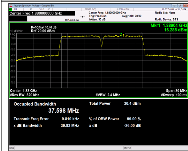
2-2-20MHz-20MHz-64QAM-64QAM-18801-18999-100RB#0-100RB#0-PASS
