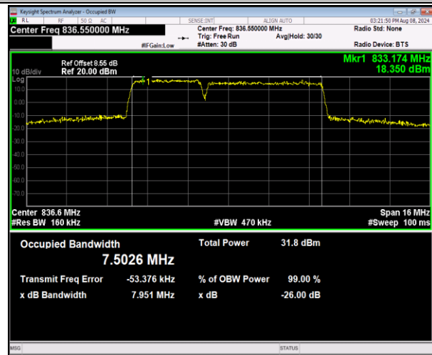
5-5-3MHz-5MHz-16QAM-16QAM-20501-20540-15RB#0-25RB#0-PASS
