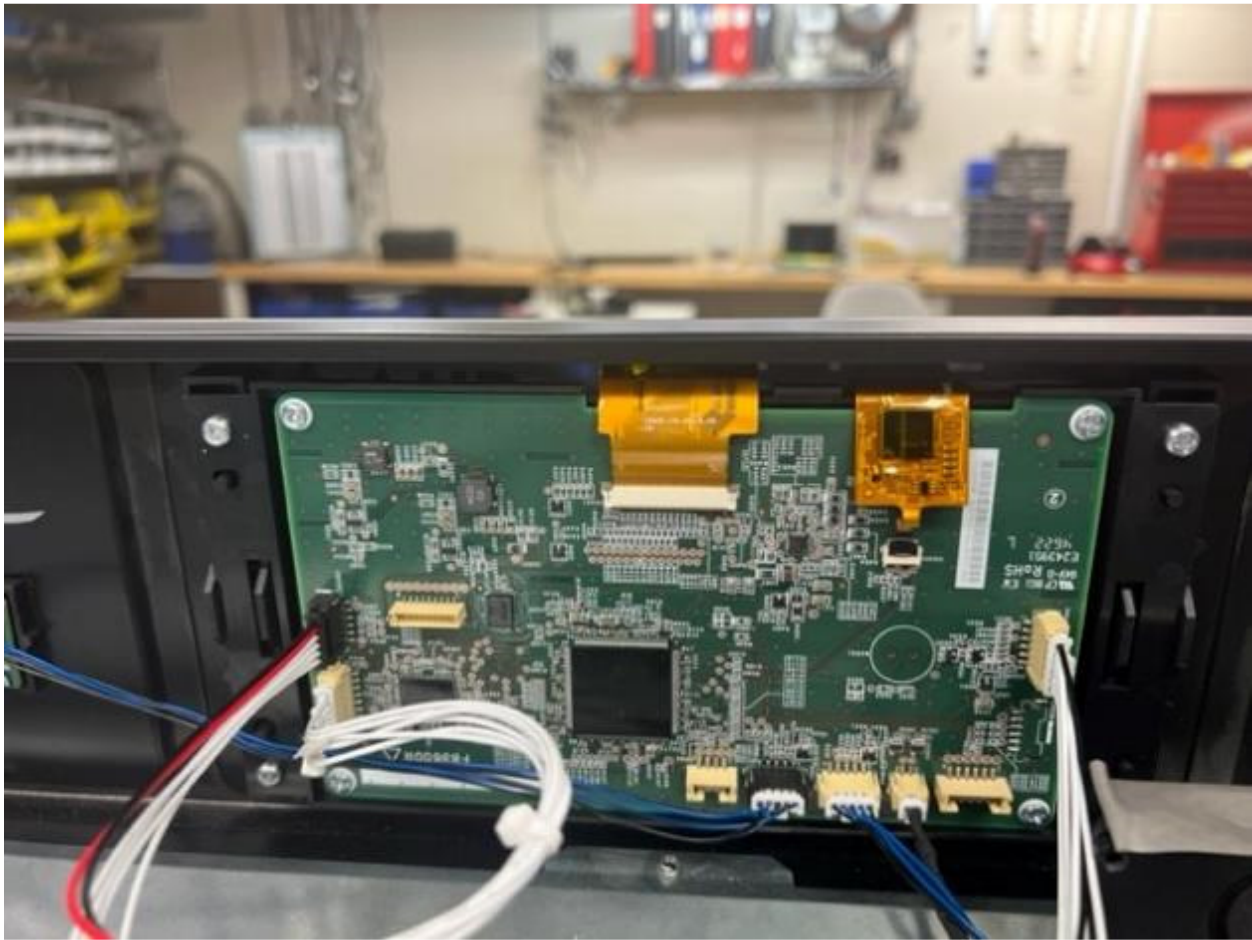
Figure 7. Rear Display Panel top of Convection Oven
