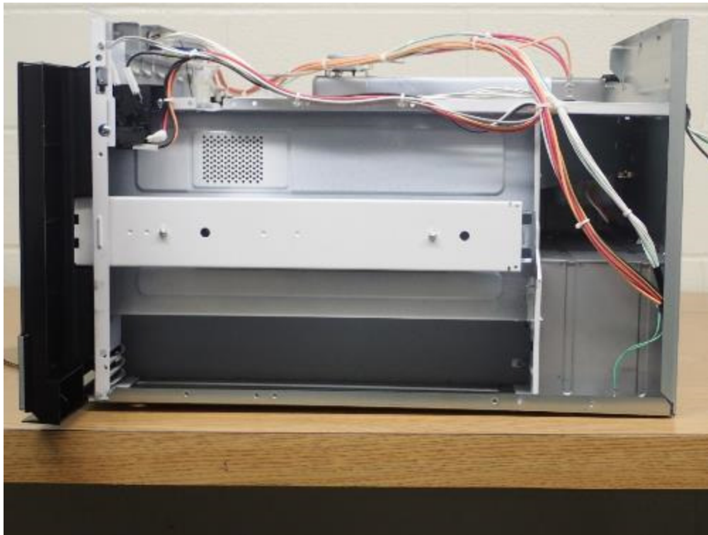
Figure 5. Right Side
