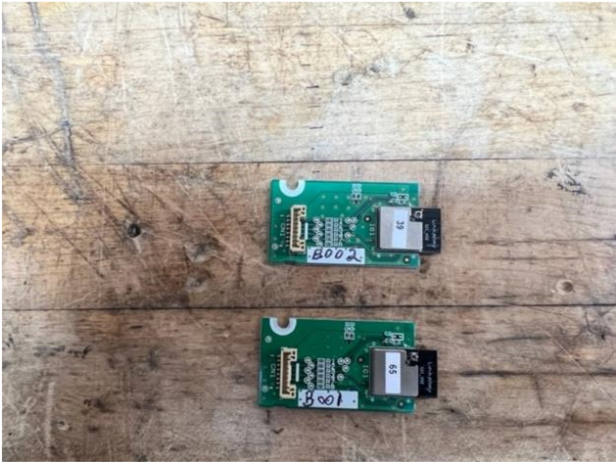
Figure 13. Wi-Fi modules on host interface boards, Top View
