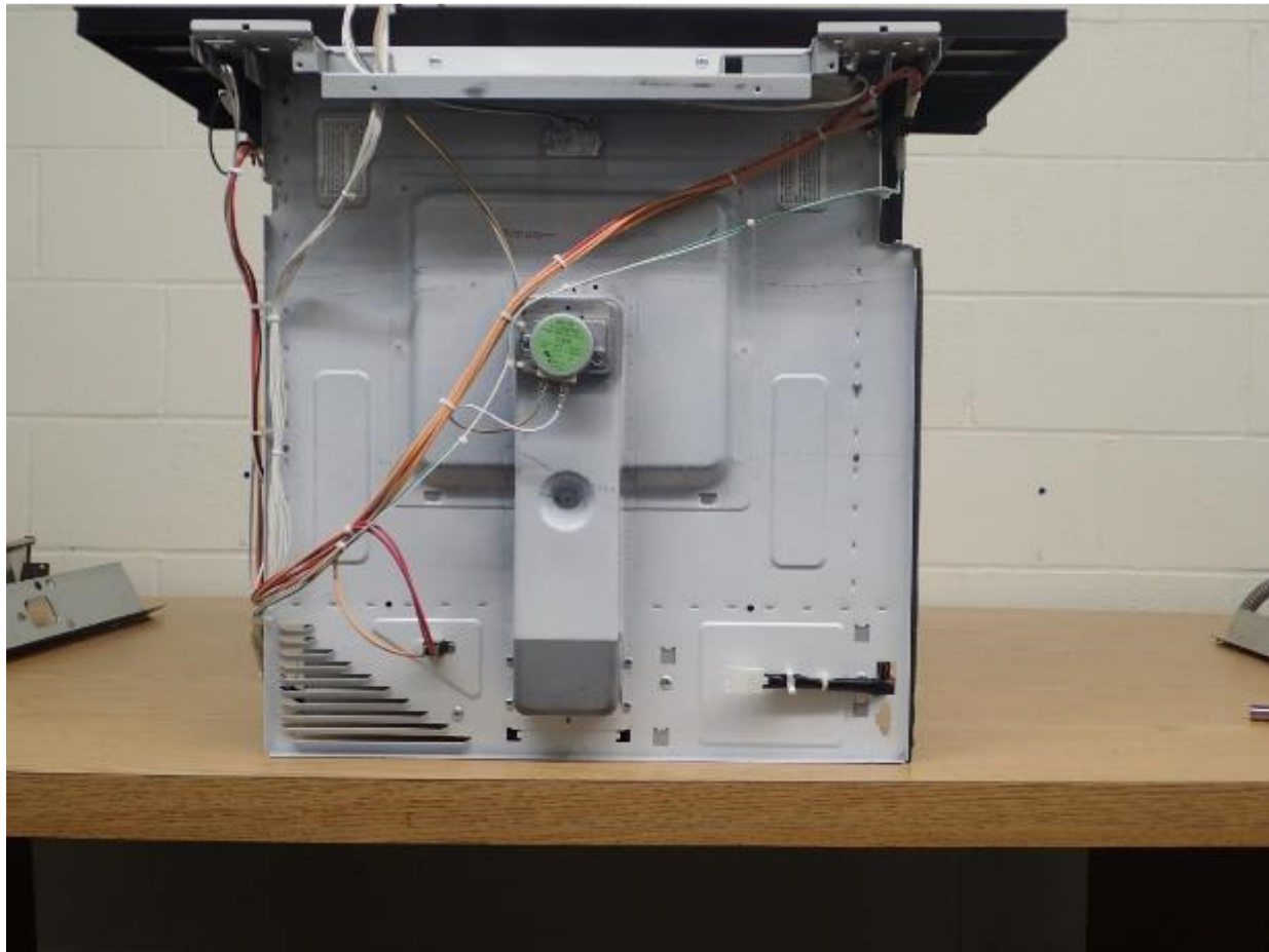
Figure 6. Top Side
