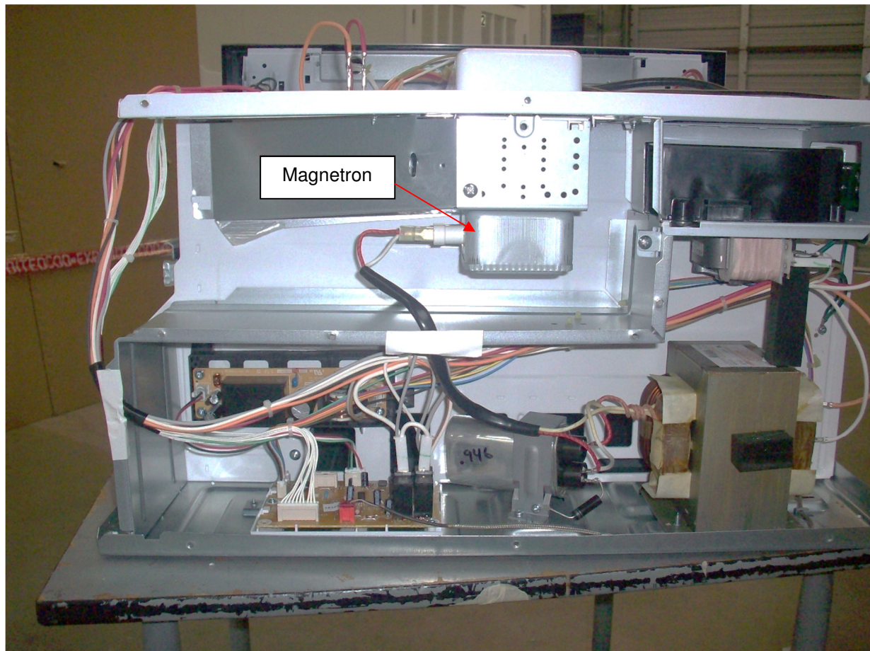
Figure 3. Rear View
