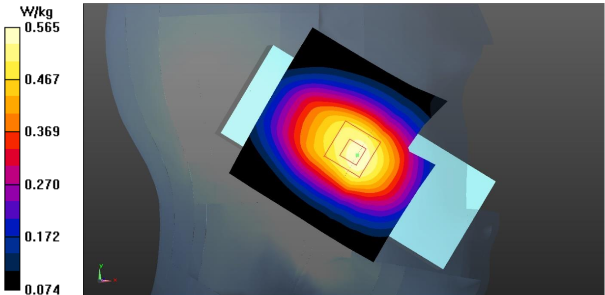
Fig.17 LTE Band 12 Head
