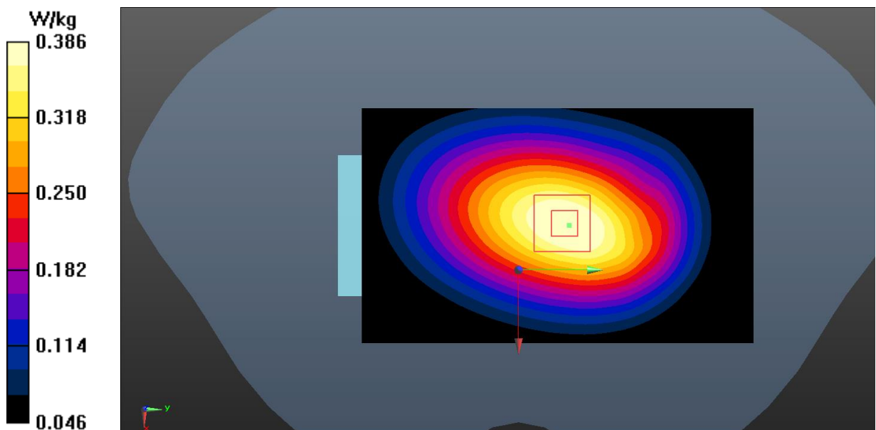
Fig.18 LTE Band 12 Body
