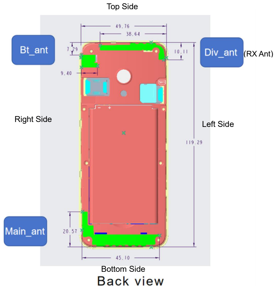
Picture 11.1 Antenna Locations (Back View)
