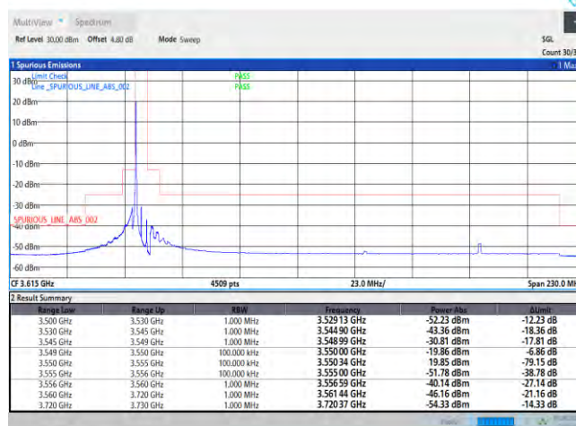
Band48-5MHz-QPSK-55265-25RB#0
