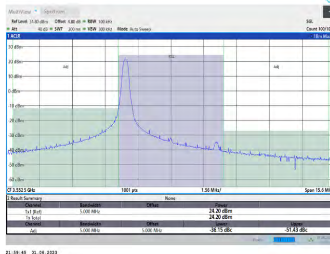
Band48-5MHz-QPSK-55265-1RB#24
