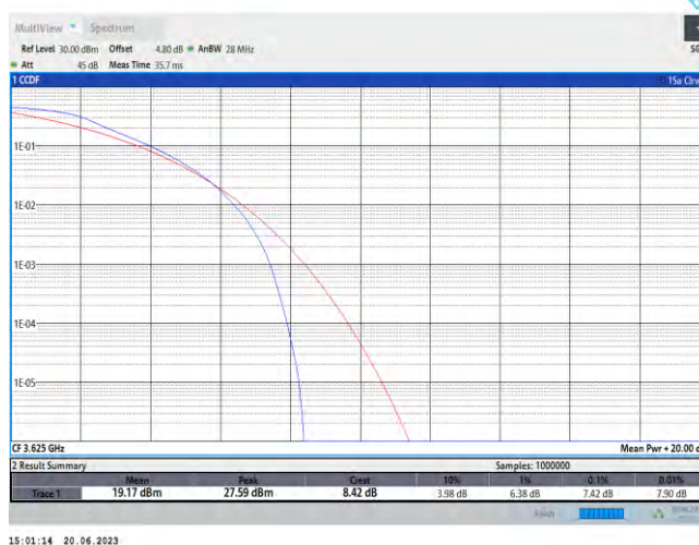
Band48-20MHz-QPSK-55990-100RB#0
