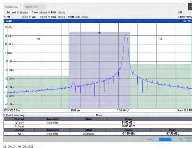
Band48-5MHz-QPSK-55265-1RB#24
