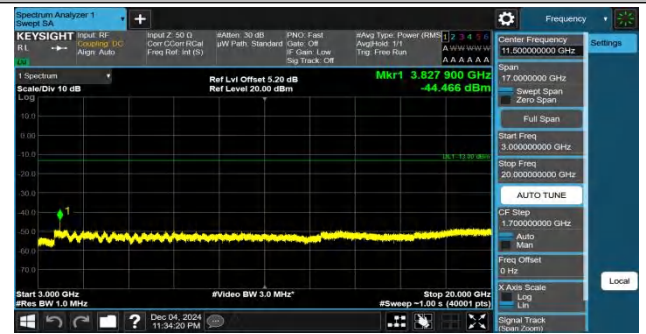
Band25-20MHz-QPSK-26590-1RB#99-3000~20000-PASS
