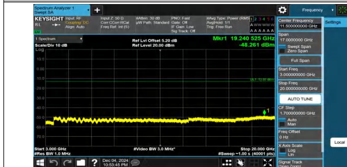
Band25-3MHz-QPSK-26365-1RB#0-3000~20000-PASS
