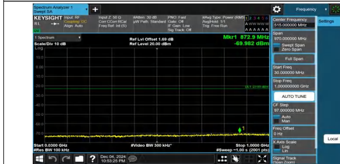
Band25-3MHz-QPSK-26365-1RB#0-30~1000-PASS
