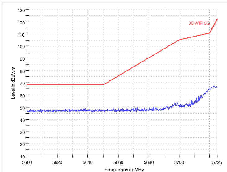
Radiated Emission Band Edge Channel No.:151 Test Mode: 802.11ac Polarization: H
