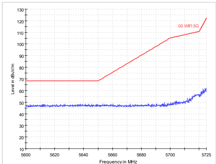
Radiated Emission Band Edge Channel No.:149 Test Mode: 802.11ac Polarization: H
